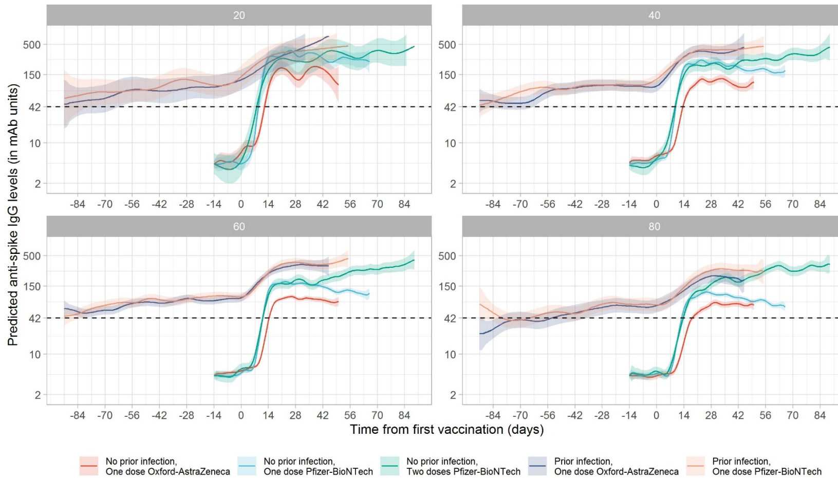
Figure 4. Predicted anti-spike IgG levels (in mAb units) by time from first vaccination for ages 20, 40, 60, and 80 years (full models shown in Figure S8, plotted by vaccine in Figure 3). Line colour indicates predicted response for different vaccine type and prior infection status. Data identical to Figure 3, but Figure 3 panels represent age rather than vaccine type.
