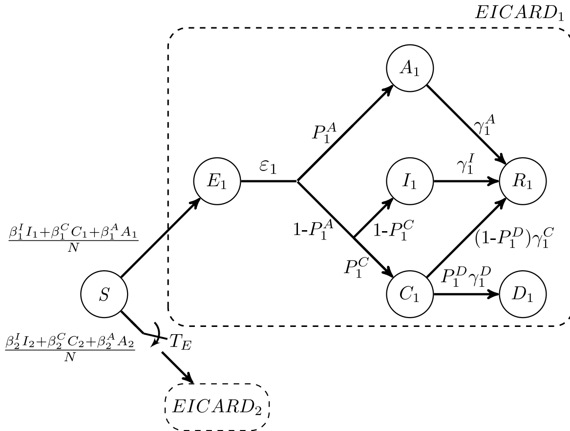
Fig. 1. Schematic of the 2-SEICARD model. For simplicity, the lower branch, corresponding to the second strain, is not depicted, and it is denoted by EICARD_2 . The EICARD_2 branch appears in the model for t \geq T_E .
