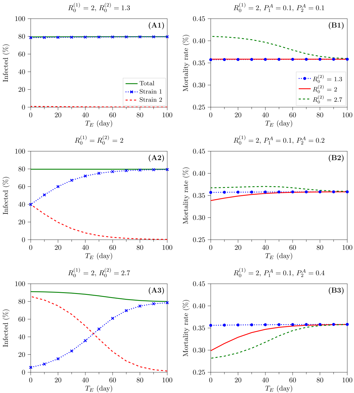
Fig. 2. The effect of R_0^{(1)} , R_0^{(2)} , P_1^A , P_2^A , and T_E on the total number of infected cases (A1-A3) and the mortality rate (B1-B3). These figures indicate that increased transmissibility of the new emergent strain does not necessarily reflect more severity of the disease. A1-A3 : The fraction of the population who are infected with strains 1 and 2 and the total percentage of the infected cases are depicted for three cases of R_0^{(1)} > R_0^{(2)} (A1), R_0^{(1)} = R_0^{(2)} (A2), and R_0^{(1)} < R_0^{(2)} (A3). Also, these figures demonstrate that the emergent time of the new strain ( T_E ) should be considered to determine the winner of the viral competition. The legends of all figures are the same as those in Fig. A1. B1-B3 : For R_0^{(1)} = 2 and P_1^A = 0.1 , these figures show the effect of increase in the fraction of asymptomatic cases of the emergent strain ( P_2^A = 0.1 (B1), 0.2 (B2), and 0.4 (B3)), on the mortality rate for different levels of transmissibility of the new variant ( R_0^{(2)} = 1.3, 2 , and 2.7). The legends of all figures are the same as those in Fig. B1.
