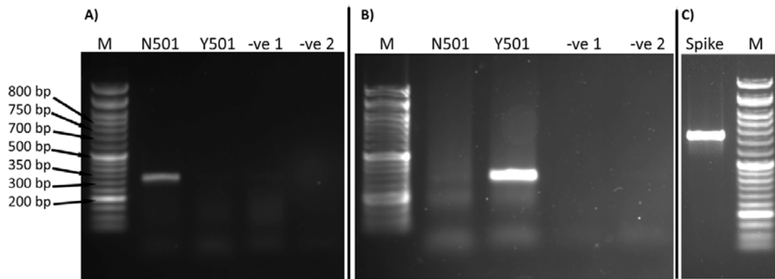
Figure 3: Agarose gel electrophoresis (1.5%). PCR products of reactions containing the specific primer of N501 A mis R wildtype (N501) or Y501 T mis R mutant (Y501) with the N501Y Endpoint F primer. -ve= contains only primers and master mix without RNA. M= Markers 50 bp. Panel A: an example of the wildtype N501. Panel B: an example of the mutant Y501. Panel C: an example of spike 748 primers sent for sequencing.
