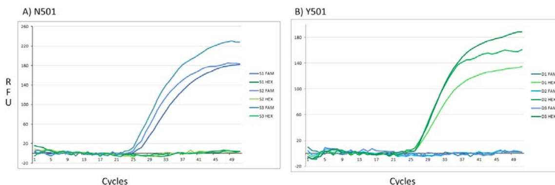
Figure 2: Taqman probe based rRT PCR. Three examples of the wildtype N501 (A) showed only FAM signals and the three samples of the mutant Y501 (B) showed only HEX signals.
