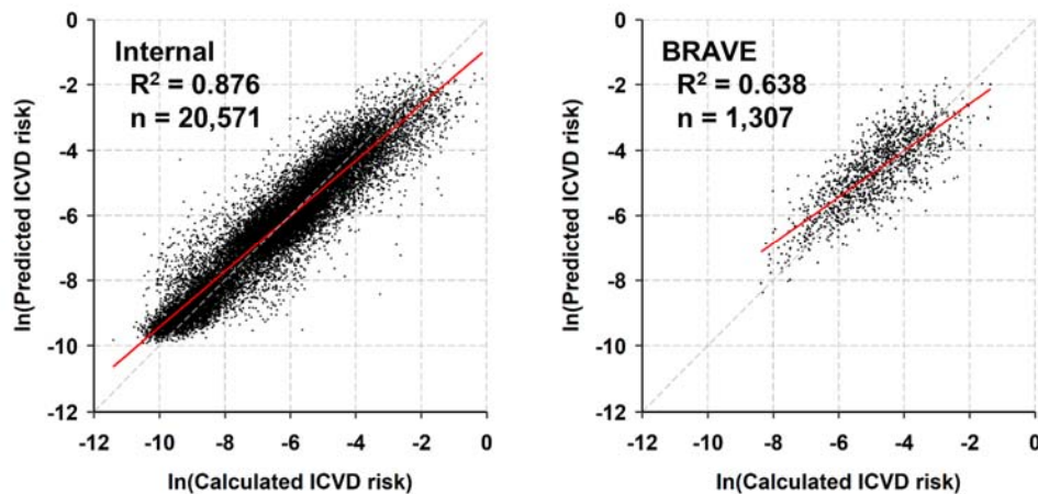
Figure 2. Prediction of natural logarithm of 10-year ICVD risk (or y_{ICVD} )
