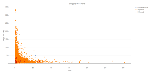
Figure 34: Charge per day for positive discharge status in Surgery
