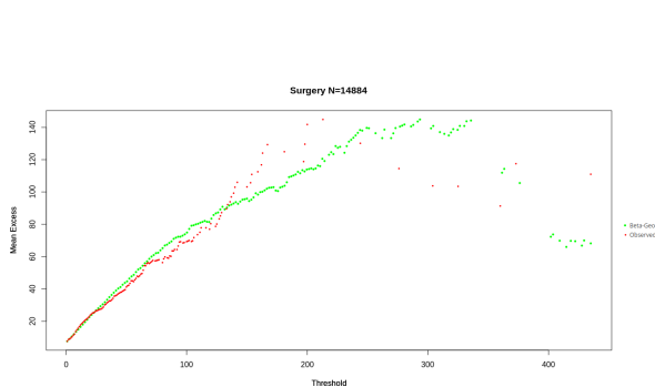
Figure 69: Mean Excess function of observed and fitted LOS per patient in Surgery
