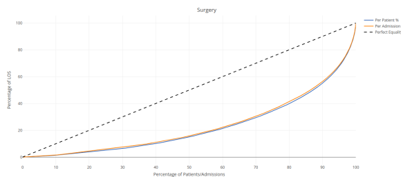
Figure 22: Lorenz curve of LOS in Surgery
