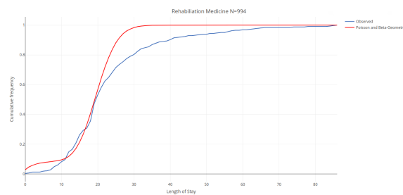
Figure 68: CDF of observed and fitted LOS per admission in Rehabilitation Medicine
