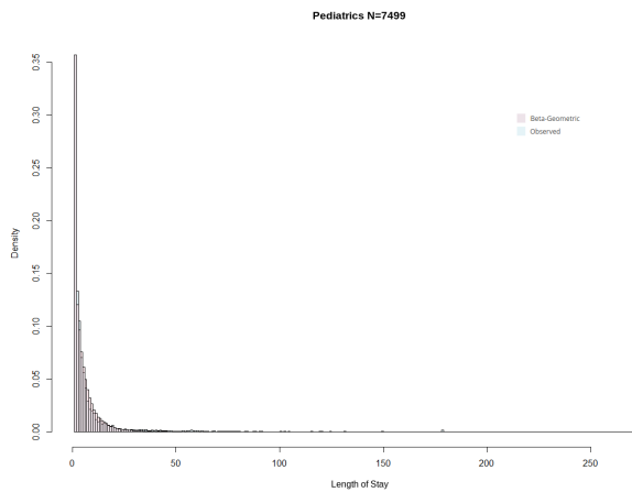
Figure 65: Histogram of observed and fitted LOS per admission in Pediatrics
