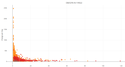
Figure 36: Charge per day for positive discharge status in Obstetrics and Gynaecology
