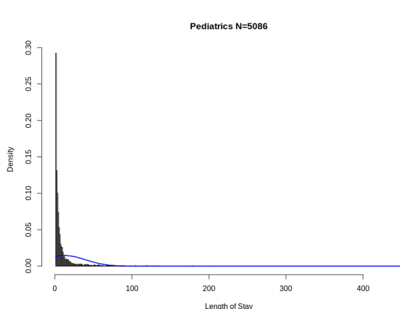
Figure 11: Histogram of LOS per patient in Pediatrics
