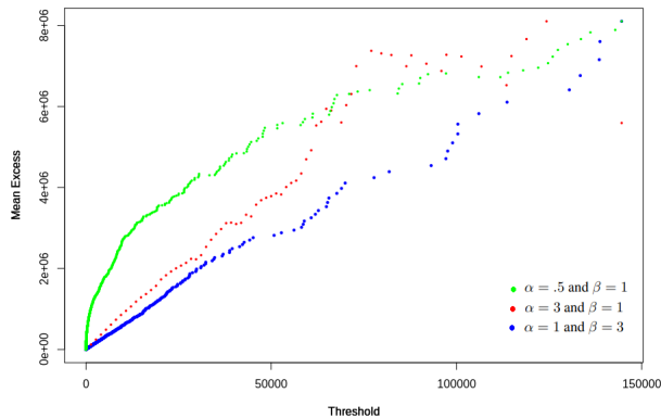
Figure 19: Mean Excess Functions for Beta-Geometric distributions
