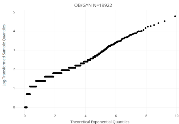
Figure 51: Q-Q plot of LOS per admission in Obstetrics and Gynaecology
