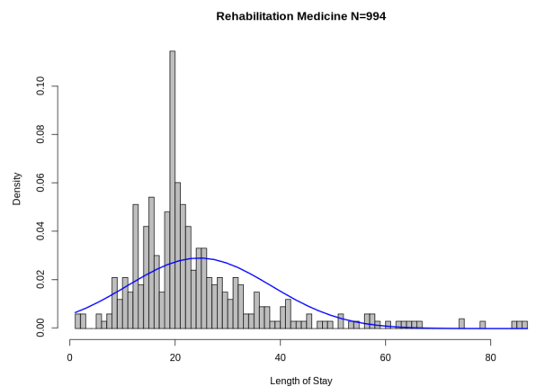
Figure 8: Histogram of LOS per admission in Rehabilitation Medicine
