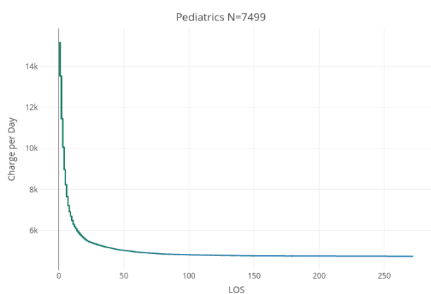
Figure 32: Average charge per day in Pediatrics
