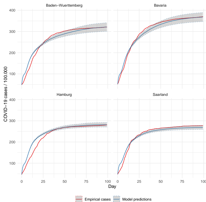
Figure 1: Model fit by state. The solid lines depict the number of reported COVID-19 cases and the average of infections across simulation runs. Shaded areas represent the 95% confidence intervals of the averages. The root mean squared error of the model’s predictions ranges between 10.17 for Bavaria and 17.68 for Hamburg.
