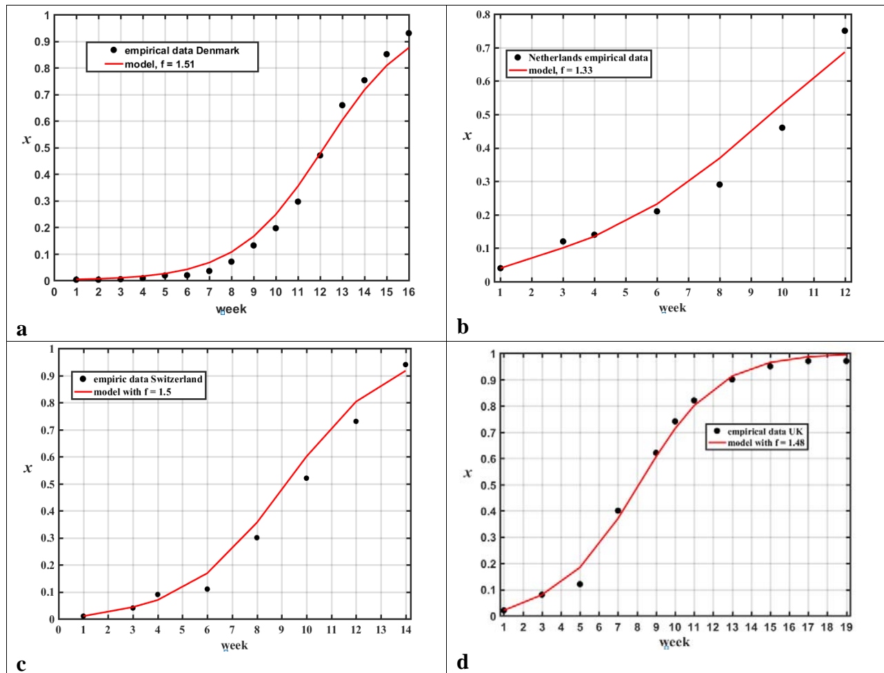
Figure 1: Change in the frequency of B.1.1.7 in the four countries of Table 1; empirical data (black circles) and formula (4) (solid line). (a) Denmark from November 2020 to 14 March 2021. (b) Netherlands from 7 December
