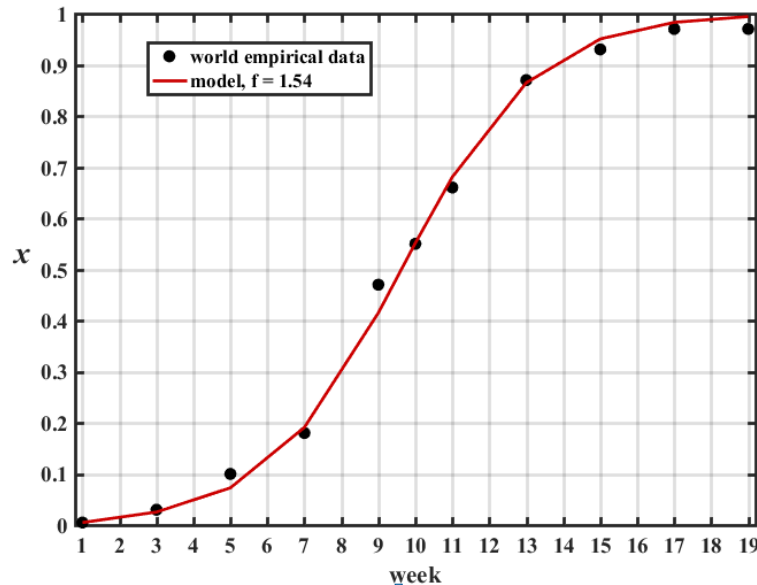
Figure 3: Change in the frequency of B.1.1.7. for the whole world: empirical data (black circles) and formula (4) (solid line).
