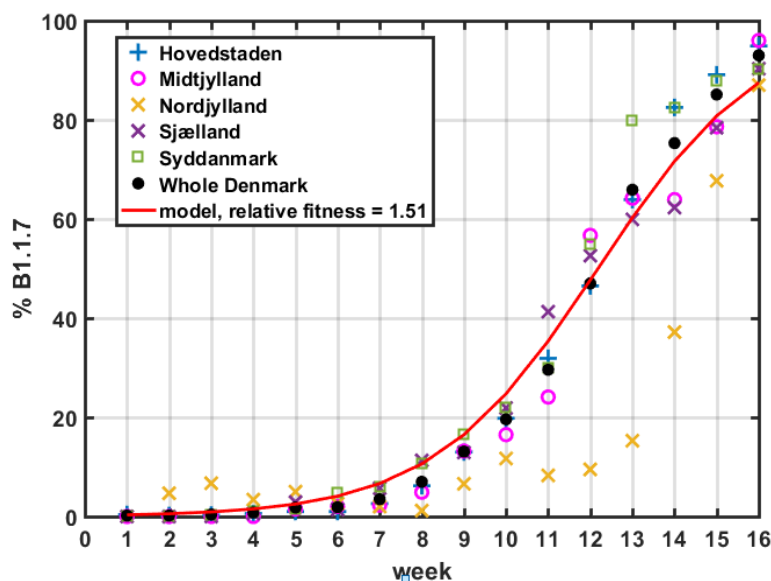
Figure 2: Change of the frequency of B.1.1.7 for different regions of Denmark as a percentage, empirical data (symbols) and formula (4) (red line).
