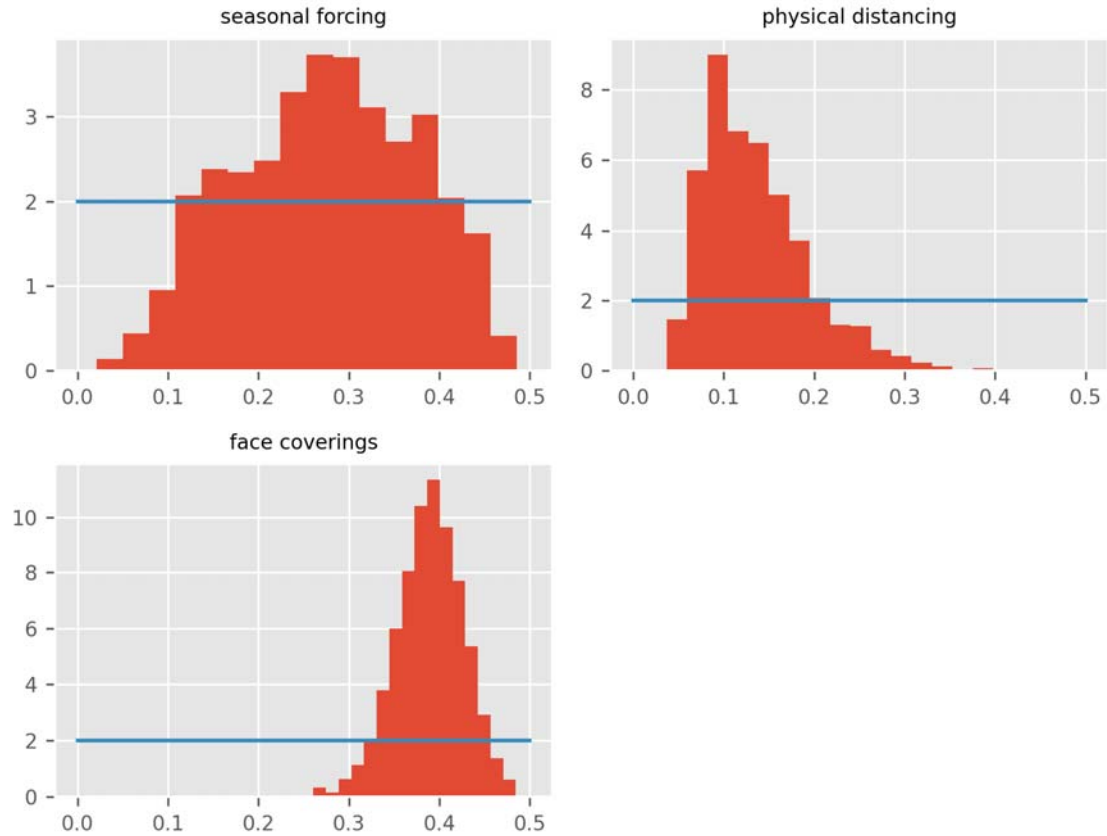
Figure 5. Posterior density histograms for key state-wide epidemiological parameters from accepted model runs. Red histograms, model posterior estimates; blue lines, prior distributions for same parameters (all are uniform or truncated normal distributions).
