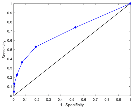
Figure 5: COVID-19 prediction performance of the olfactory test assuming equal weights for the odors. The best classification performance is obtained with a score of four or less correctly identified odors (COVID-19 positive). The UC-Christus dataset was employed to evaluate the performance of this model.
