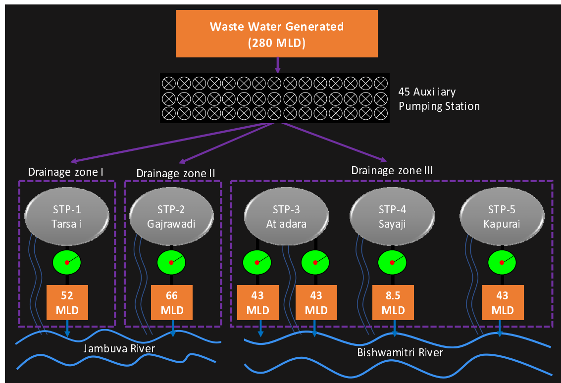
Fig.2. Sampling points and layout of the wastewater treatment in Vadodara, Gujarat, India
