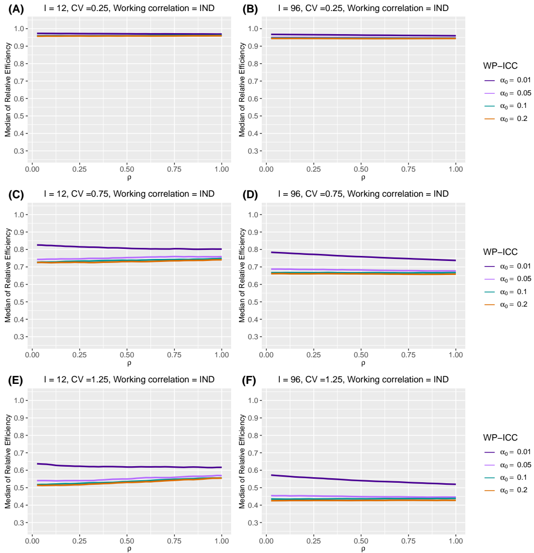
Web Figure 32 The median of relative efficiency (RE) as a function of within-period intraclass correlation coefficient (WP-ICC) \alpha_0 \in \{0.01, 0.05, 0.1, 0.2\} and the decay rate \rho \in (0, 1) , when the true correlation model is exponential decay (ED) and the working correlation model is independence (IND). Design factors considered are as follows: number of clusters I = 12 and 96 , number of periods J = 5 , mean cluster-period size \bar{n} = 100 , and the degree of between-cluster imbalance is defined by coefficient of variation CV \in \{0.25, 0.75, 1.25\} . No within-cluster imbalance is introduced.
