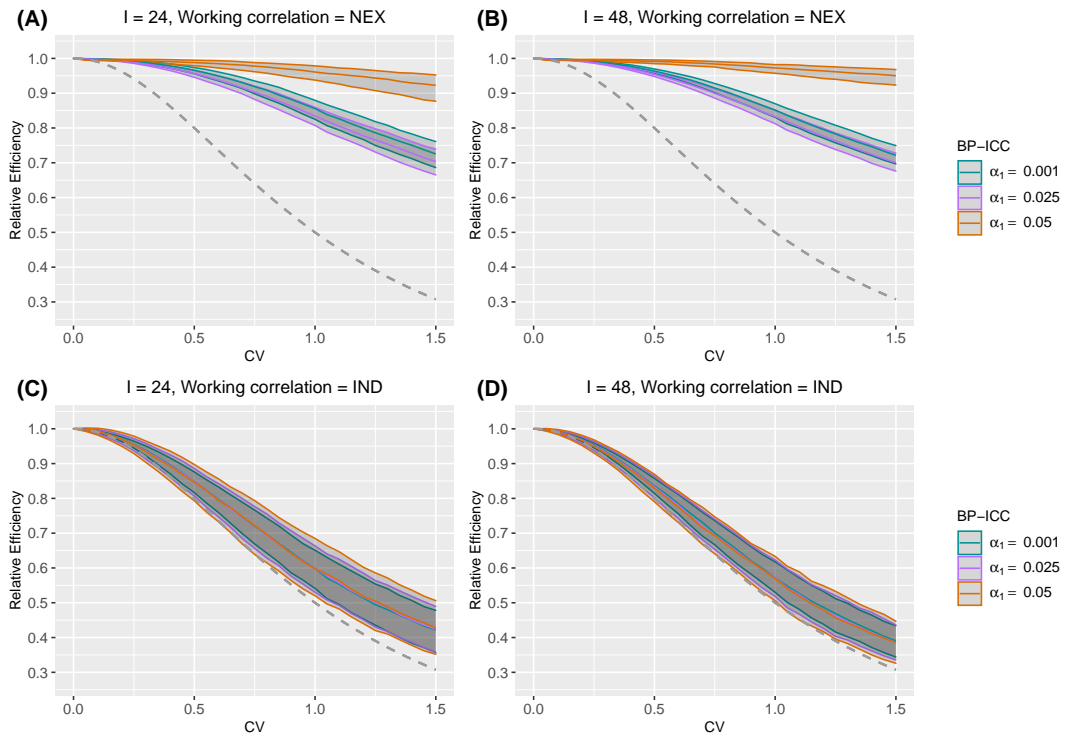
Web Figure 48 The median and interquartile range (IQR) of relative efficiency (RE) as a function of coefficient of variation (CV) measuring between-cluster imbalance, when the true correlation model is nested exchangeable (NEX). Design factors considered are as follows: number of clusters I = 24 and 48 , number of periods J = 5 . The within-period intraclass correlation coefficient (WP-ICC) \alpha_0 = 0.05 , and between-period intraclass correlation coefficient (BP-ICC) \alpha_1 \in \{0.001, 0.025, 0.05\} . No within-cluster imbalance is introduced. The broken grey curve shows the reciprocal of the conservative inflation factor 1 + CV^2 .
