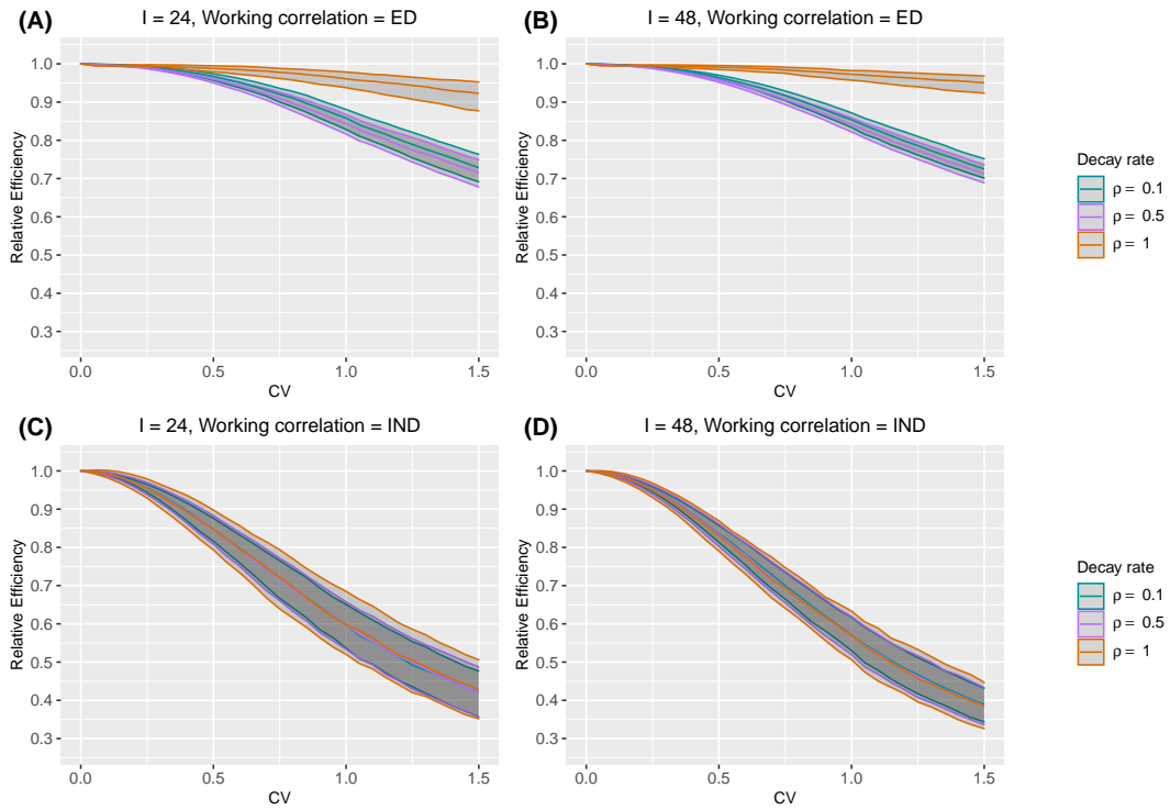
Web Figure 22 The median and interquartile range (IQR) of relative efficiency (RE) as a function of coefficient of variation (CV) measuring between-cluster imbalance, when the true correlation model is exponential decay. Design factors considered are as follows: number of clusters I = 24 and 48 , number of periods J = 5 . The within-period intraclass correlation coefficient (WP-ICC) \alpha_0 = 0.05 , and decay rate \rho \in \{0.1, 0.5, 1\} . No within-cluster variability in cluster-period sizes is introduced.
