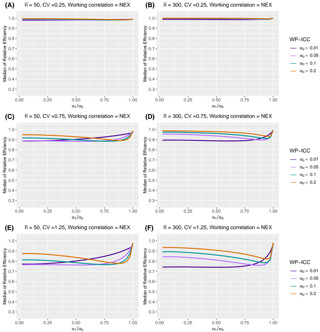
Web Figure 14 The median of relative efficiency (RE) as a function of the within-period intraclass correlation coefficient (WP-ICC) \alpha_0 \in \{0.01, 0.05, 0.1, 0.2\} and the ratio of between-period intraclass correlation coefficient (BP-ICC) to WP-ICC, \alpha_1/\alpha_0 \in [0, 1] , when both the true correlation model and the working correlation model are nested exchangeable (NEX). Design factors considered are as follows: number of clusters I = 96 , number of periods J = 5 , mean cluster-period sizes \bar{n} \in \{50, 300\} , and the degree of between-cluster imbalance is defined by coefficient of variation CV \in \{0.25, 0.75, 1.25\} . No within-cluster imbalance is introduced.
