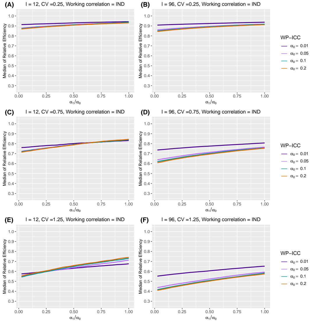
Web Figure 11 The median of relative efficiency (RE) as a function of the within-period intraclass correlation coefficient (WP-ICC) \alpha_0 \in \{0.01, 0.05, 0.1, 0.2\} and the ratio of between-period intraclass correlation coefficient (BP-ICC) to WP-ICC, \alpha_1/\alpha_0 \in [0, 1] , when the true correlation model is nested exchangeable (NEX) and the working correlation model is independence (IND). Design factors considered are as follows: number of clusters I = 12 and 96 , number of periods J = 5 , and the degree of between-cluster imbalance is defined by CV \in \{0.25, 0.75, 1.25\} . Within-cluster imbalance (pattern 4: randomly permuted) is introduced.
