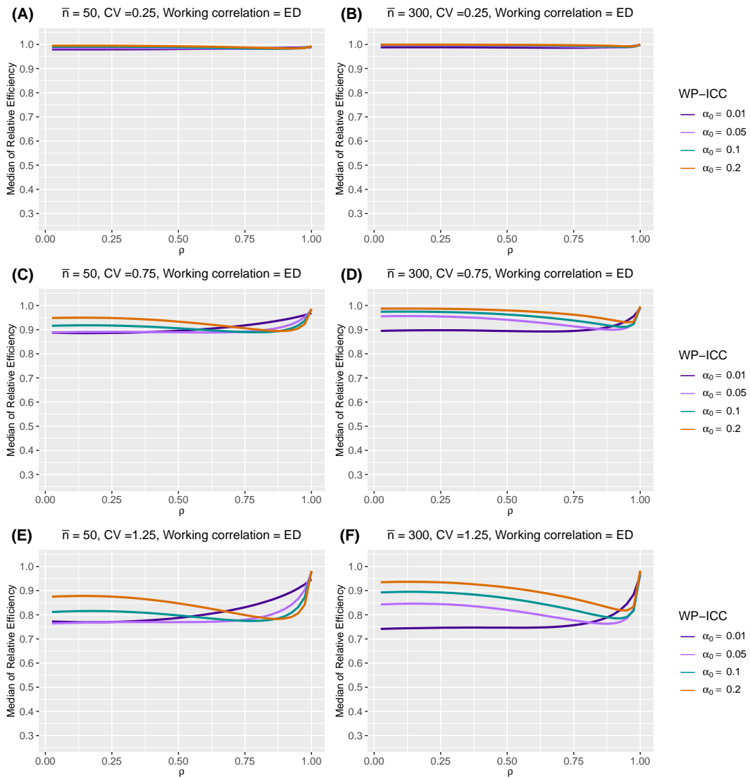
Web Figure 38 The median of relative efficiency (RE) as a function of the within-period intraclass correlation coefficient (WP-ICC) \alpha_0 \in \{0.01, 0.05, 0.1, 0.2\} and the decay rate \rho \in (0, 1) , when both the true correlation model and the working correlation model are exponential decay (ED). Design factors considered are as follows: number of clusters I = 96 , number of periods J = 5 , mean cluster-period sizes \bar{n} \in \{50, 300\} , and the degree of between-cluster imbalance is defined by coefficient of variation CV \in \{0.25, 0.75, 1.25\} . No within-cluster imbalance is introduced.
