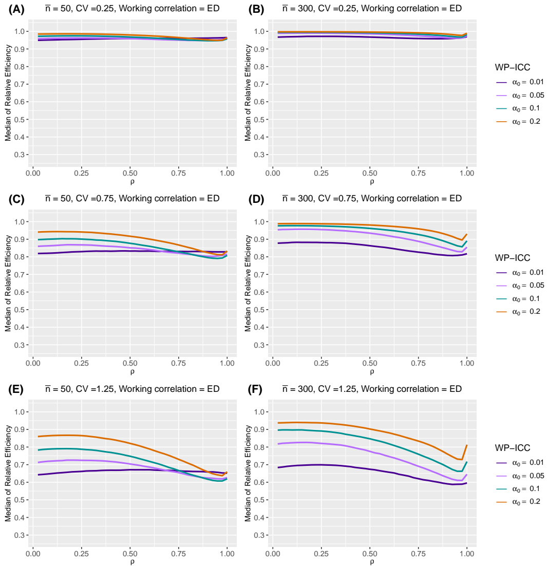
Web Figure 39 The median of relative efficiency (RE) as a function of the within-period intraclass correlation coefficient (WP-ICC) \alpha_0 \in \{0.01, 0.05, 0.1, 0.2\} and the decay rate \rho \in (0, 1) , when both the true correlation model and the working correlation model are exponential decay (ED). Design factors considered are as follows: number of clusters I = 12 , number of periods J = 5 , mean cluster-period sizes \bar{n} \in \{50, 300\} , and the degree of between-cluster imbalance is defined by coefficient of variation CV \in \{0.25, 0.75, 1.25\} . Within-cluster imbalance (pattern 4: randomly permuted) is introduced.
