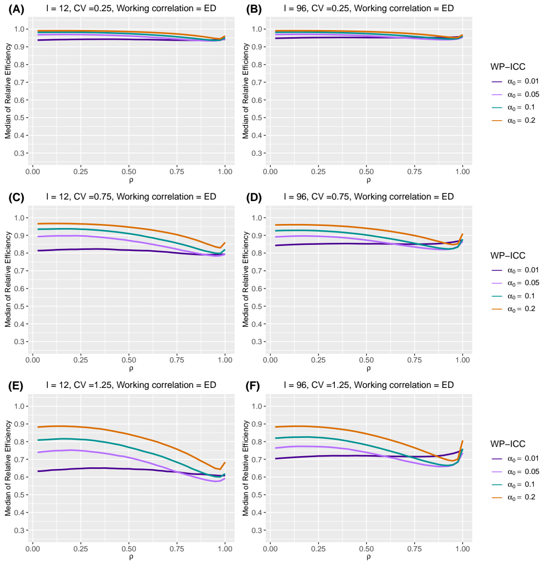
Web Figure 30 The median of relative efficiency (RE) as a function of within-period intraclass correlation coefficient (WP-ICC) \alpha_0 \in \{0.01, 0.05, 0.1, 0.2\} and the decay rate \rho \in (0, 1) , when both the true correlation model and the working correlation model are exponential decay (ED). Design factors considered are as follows: number of clusters I = 12 and 96 , number of periods J = 5 , mean cluster-period size \bar{n} = 100 , and the degree of between-cluster imbalance is defined by coefficient of variation CV \in \{0.25, 0.75, 1.25\} . Within-cluster imbalance (pattern 3: monotonically decreasing) is introduced.
