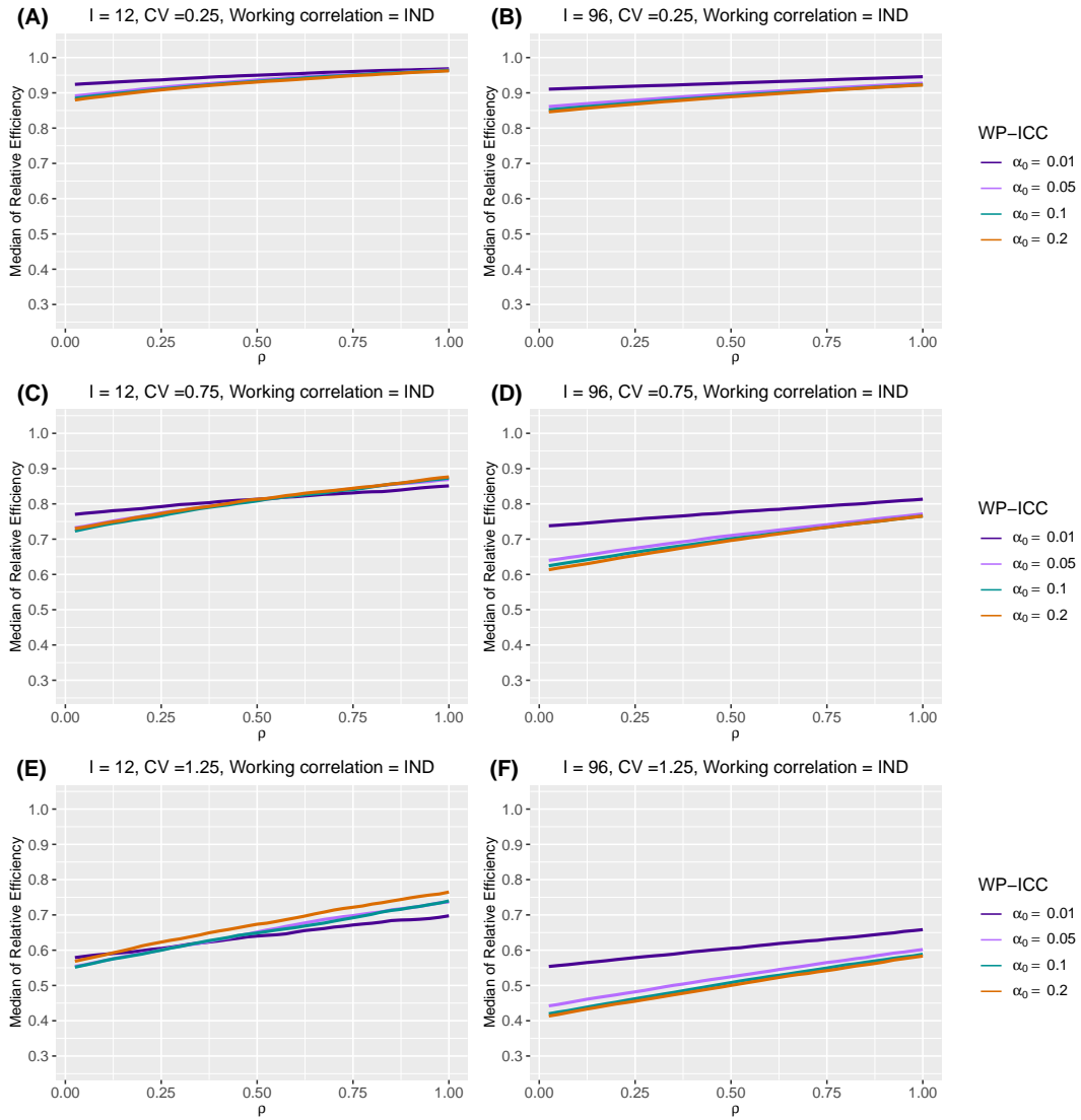
Web Figure 34 The median of relative efficiency (RE) as a function of within-period intraclass correlation coefficient (WP-ICC) \alpha_0 \in \{0.01, 0.05, 0.1, 0.2\} and the decay rate \rho \in (0, 1) , when the true correlation model is exponential decay (ED) and the working correlation model is independence (IND). Design factors considered are as follows: number of clusters I = 12 and 96, number of periods J = 5 , mean cluster-period size \bar{n} = 100 , and the degree of between-cluster imbalance is defined by coefficient of variation CV \in \{0.25, 0.75, 1.25\} . Within-cluster imbalance (pattern 2: monotonically increasing) is introduced.
