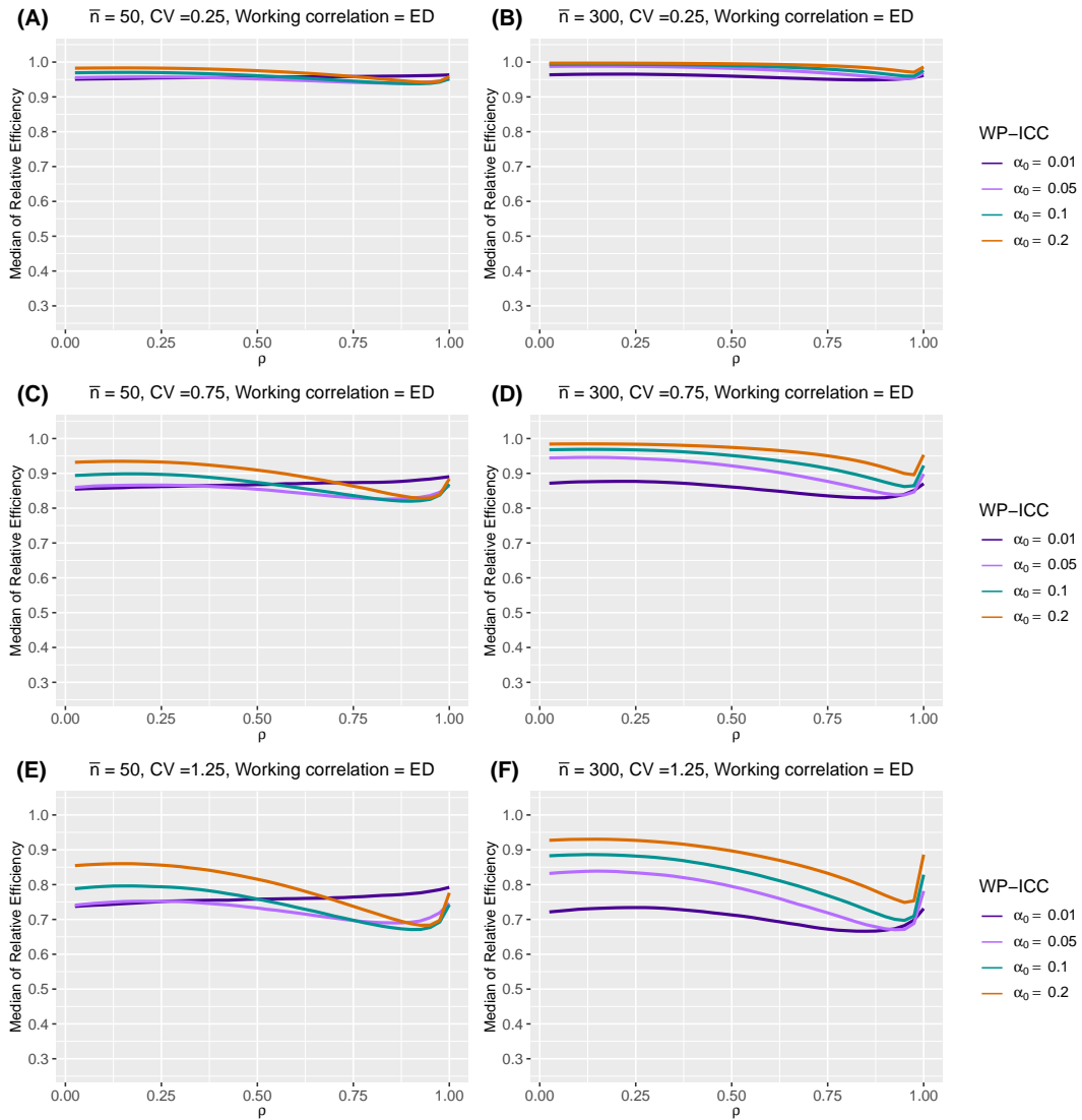
Web Figure 40 The median of relative efficiency (RE) as a function of the within-period intraclass correlation coefficient (WP-ICC) \alpha_0 \in \{0.01, 0.05, 0.1, 0.2\} and the decay rate \rho \in (0, 1) , when both the true correlation model and the working correlation model are exponential decay (ED). Design factors considered are as follows: number of clusters I = 96 , number of periods J = 5 , mean cluster-period sizes \bar{n} \in \{50, 300\} , and the degree of between-cluster imbalance is defined by coefficient of variation CV \in \{0.25, 0.75, 1.25\} . Within-cluster imbalance (pattern 4: randomly permuted) is introduced.
