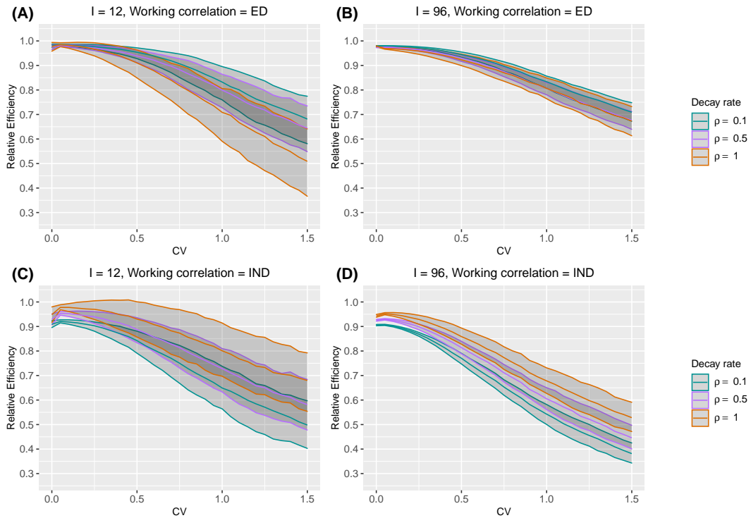
Web Figure 26 The median and interquartile range (IQR) of relative efficiency (RE) as a function of coefficient of variation (CV) measuring between-cluster imbalance, when the true correlation model is exponential decay. Design factors considered are as follows: number of clusters I = 12 and 96 , number of periods J = 5 . The within-period intraclass correlation coefficient (WP-ICC) \alpha_0 = 0.05 , and decay rate \rho \in \{0.1, 0.5, 1\} . Within-cluster imbalance (pattern 4: randomly permuted) is introduced.
