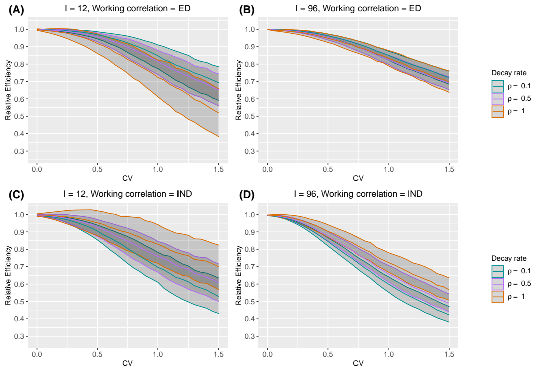
Web Figure 23 The median and interquartile range (IQR) of relative efficiency (RE) as a function of coefficient of variation (CV) measuring between-cluster imbalance, when the true correlation model is exponential decay. Design factors considered are as follows: number of clusters I = 12 and 96 , number of periods J = 5 . The within-period intraclass correlation coefficient (WP-ICC) \alpha_0 = 0.05 , and decay rate \rho \in \{0.1, 0.5, 1\} . Within-cluster imbalance (pattern 1: constant) is introduced.
