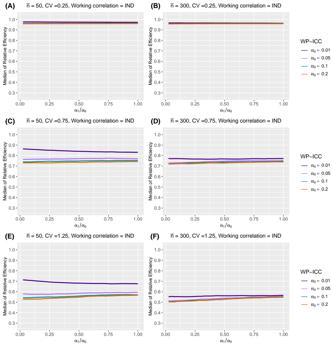
Web Figure 17 The median of relative efficiency (RE) as a function of the within-period intraclass correlation coefficient (WP-ICC) \alpha_0 \in \{0.01, 0.05, 0.1, 0.2\} and the ratio of between-period intraclass correlation coefficient (BP-ICC) to WP-ICC, \alpha_1/\alpha_0 \in [0, 1] , when the true correlation model is nested exchangeable (NEX) and the working correlation model is independence (IND). Design factors considered are as follows: number of clusters I = 12 , number of periods J = 5 , mean cluster-period sizes \bar{n} \in \{50, 300\} , and the degree of between-cluster imbalance is defined by coefficient of variation CV \in \{0.25, 0.75, 1.25\} . No within-cluster imbalance is introduced.
