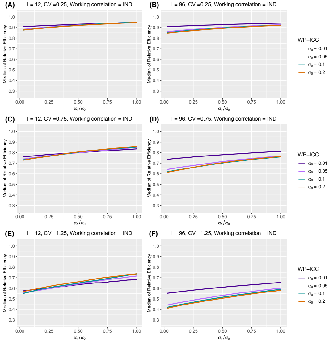
Web Figure 10 The median of relative efficiency (RE) as a function of the within-period intraclass correlation coefficient (WP-ICC) \alpha_0 \in \{0.01, 0.05, 0.1, 0.2\} and the ratio of between-period intraclass correlation coefficient (BP-ICC) to WP-ICC, \alpha_1/\alpha_0 \in [0, 1] , when the true correlation model is nested exchangeable (NEX) and the working correlation model is independence (IND). Design factors considered are as follows: number of clusters I = 12 and 96 , number of periods J = 5 , and the degree of between-cluster imbalance is defined by CV \in \{0.25, 0.75, 1.25\} . Within-cluster imbalance (pattern 3: monotonically decreasing) is introduced.
