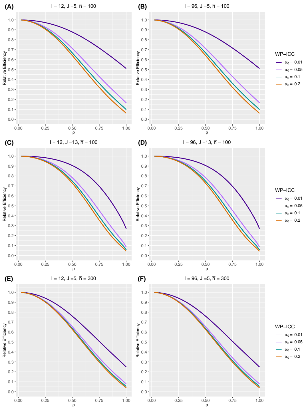
Web Figure 46 Median of new defined relative efficiency (RE) under the true versus independence (IND) working correlation model as a function of the within-period intraclass correlation coefficient (WP-ICC) \alpha_0 \in \{0.01, 0.05, 0.1, 0.2\} and the decay rate \rho \in [0, 1] , when the true correlation model is exponential decay (ED). Design factors considered are as follows: number of clusters I = 12 and 96 , number of periods J = 5 and 13 , and mean cluster-period sizes \bar{n} = 100 and 300 .
