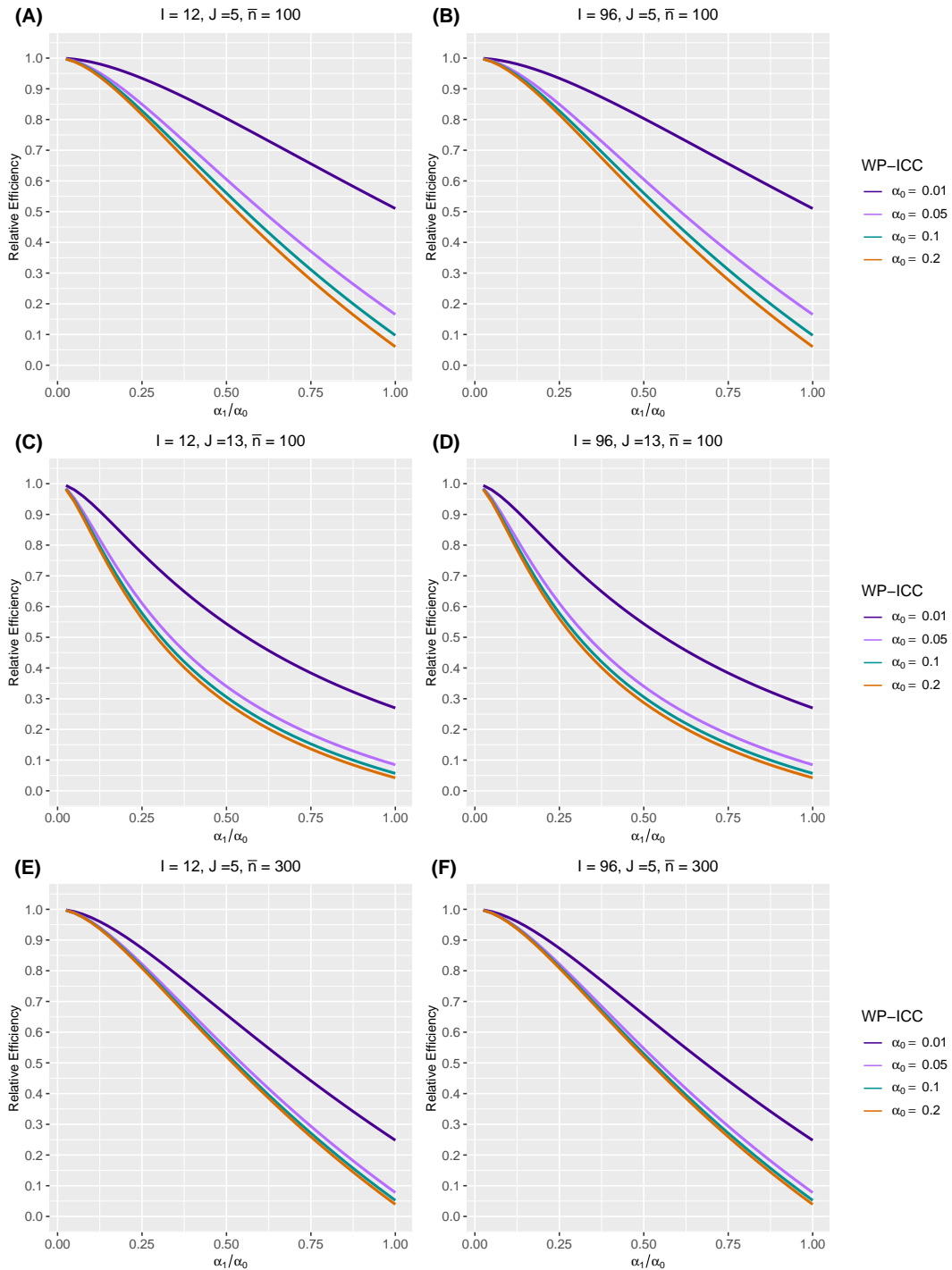
Web Figure 45 Median of new defined relative efficiency (RE) under the true versus independence (IND) working correlation model as a function of the within-period intraclass correlation coefficient (WP-ICC) \alpha_0 \in \{0.01, 0.05, 0.1, 0.2\} and the ratio of between-period intraclass correlation coefficient (BP-ICC) to WP-ICC, \alpha_1/\alpha_0 \in [0, 1] , when the true correlation model is nested exchangeable (NEX). Design factors considered are as follows: number of clusters I = 12 and 96 , number of periods J = 5 and 13 , and mean cluster-period sizes \bar{n} = 100 and 300 .
