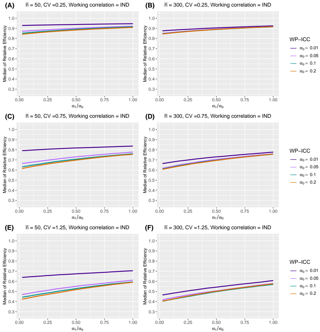
Web Figure 20 The median of relative efficiency (RE) as a function of the within-period intraclass correlation coefficient (WP-ICC) \alpha_0 \in \{0.01, 0.05, 0.1, 0.2\} and the ratio of between-period intraclass correlation coefficient (BP-ICC) to WP-ICC, \alpha_1/\alpha_0 \in [0, 1] , when the true correlation model is nested exchangeable (NEX) and the working correlation model is independence (IND). Design factors considered are as follows: number of clusters I = 96 , number of periods J = 5 , mean cluster-period sizes \bar{n} \in \{50, 300\} , and the degree of between-cluster imbalance is defined by coefficient of variation CV \in \{0.25, 0.75, 1.25\} . Within-cluster imbalance (pattern 4: randomly permuted) is introduced.
