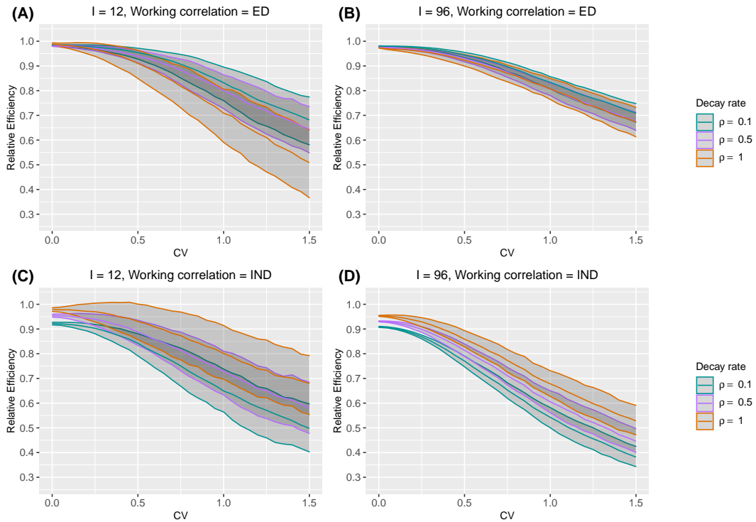
Web Figure 24 The median and interquartile range (IQR) of relative efficiency (RE) as a function of coefficient of variation (CV) measuring between-cluster imbalance, when the true correlation model is exponential decay. Design factors considered are as follows: number of clusters I = 12 and 96 , number of periods J = 5 . The within-period intraclass correlation coefficient (WP-ICC) \alpha_0 = 0.05 , and decay rate \rho \in \{0.1, 0.5, 1\} . Within-cluster imbalance (pattern 2: monotonically increasing) is introduced.
