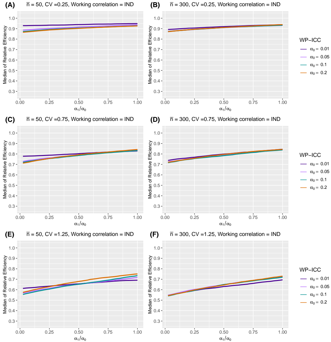
Web Figure 19 The median of relative efficiency (RE) as a function of the within-period intraclass correlation coefficient (WP-ICC) \alpha_0 \in \{0.01, 0.05, 0.1, 0.2\} and the ratio of between-period intraclass correlation coefficient (BP-ICC) to WP-ICC, \alpha_1/\alpha_0 \in [0, 1] , when the true correlation model is nested exchangeable (NEX) and the working correlation model is independence (IND). Design factors considered are as follows: number of clusters I = 12 , number of periods J = 5 , mean cluster-period sizes \bar{n} \in \{50, 300\} , and the degree of between-cluster imbalance is defined by coefficient of variation CV \in \{0.25, 0.75, 1.25\} . Within-cluster imbalance (pattern 4: randomly permuted) is introduced.
