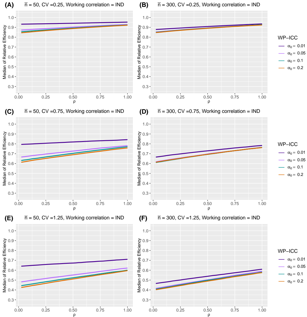
Web Figure 44 The median of relative efficiency (RE) as a function of the within-period intraclass correlation coefficient (WP-ICC) \alpha_0 \in \{0.01, 0.05, 0.1, 0.2\} and the decay rate \rho \in (0, 1) , when the true correlation model is exponential decay (ED) and the working correlation model is independence (IND). Design factors considered are as follows: number of clusters I = 96 , number of periods J = 5 , mean cluster-period sizes \bar{n} \in \{50, 300\} , and the degree of between-cluster imbalance is defined by coefficient of variation CV \in \{0.25, 0.75, 1.25\} . Within-cluster imbalance (pattern 4: randomly permuted) is introduced.
