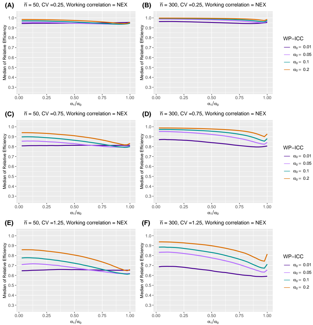
Web Figure 15 The median of relative efficiency (RE) as a function of the within-period intraclass correlation coefficient (WP-ICC) \alpha_0 \in \{0.01, 0.05, 0.1, 0.2\} and the ratio of between-period intraclass correlation coefficient (BP-ICC) to WP-ICC, \alpha_1/\alpha_0 \in [0, 1] , when both the true correlation model and the working correlation model are nested exchangeable (NEX). Design factors considered are as follows: number of clusters I = 12 , number of periods J = 5 , mean cluster-period sizes \bar{n} \in \{50, 300\} , and the degree of between-cluster imbalance is defined by coefficient of variation CV \in \{0.25, 0.75, 1.25\} . Within-cluster imbalance (pattern 4: randomly permuted) is introduced.
