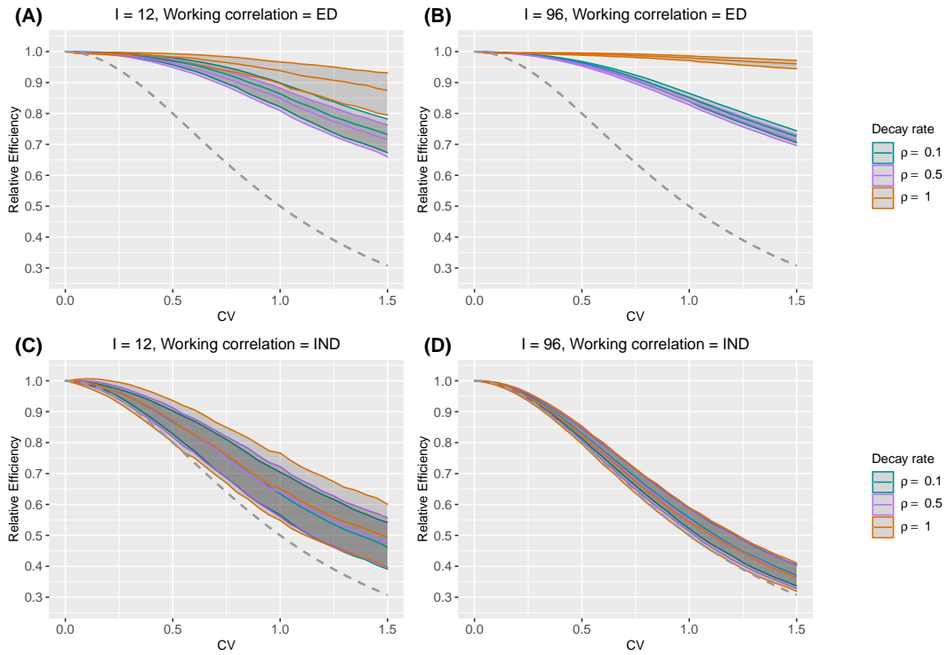
Web Figure 49 The median and interquartile range (IQR) of relative efficiency (RE) as a function of coefficient of variation (CV) measuring between-cluster imbalance, when the true correlation model is exponential decay (ED). Design factors considered are as follows: number of clusters I = 12 and 96, number of periods J = 5 . The within-period intraclass correlation coefficient (WP-ICC) \alpha_0 = 0.05 , and decay parameter \rho \in \{0.1, 0.5, 1\} . No within-cluster imbalance is introduced. The broken grey curve shows the reciprocal of the conservative inflation factor 1 + CV^2 .
