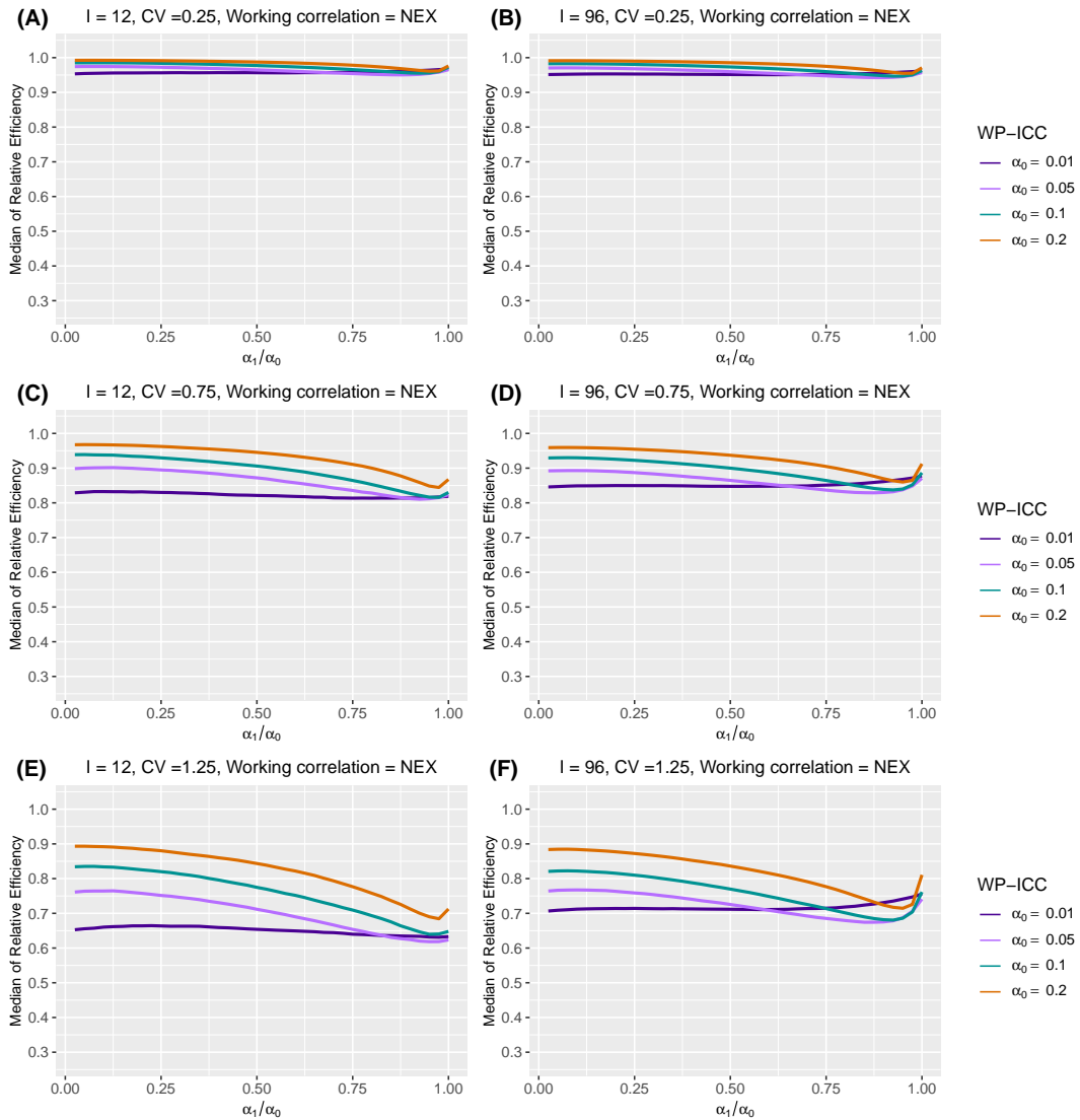
Web Figure 5 The median of relative efficiency (RE) as a function of the within-period intraclass correlation coefficient (WP-ICC) \alpha_0 \in \{0.01, 0.05, 0.1, 0.2\} and the ratio of between-period intraclass correlation coefficient (BP-ICC) to WP-ICC, \alpha_1/\alpha_0 \in [0, 1] , when both the true correlation model and the working correlation model are nested exchangeable (NEX). Design factors considered are as follows: number of clusters I = 12 and 96, number of periods J = 5 , and the degree of between-cluster imbalance is defined by CV \in \{0.25, 0.75, 1.25\} . Within-cluster imbalance (pattern 2: monotonically increasing) is introduced.
