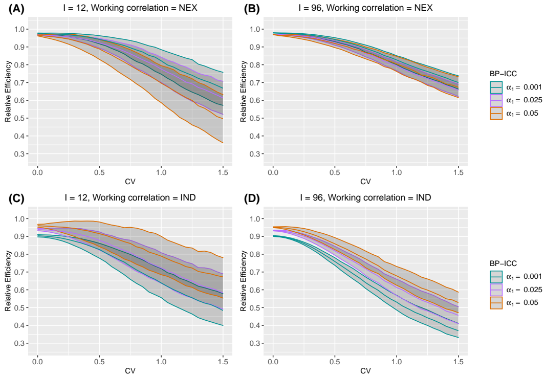
Web Figure 3 The median and interquartile range (IQR) of relative efficiency (RE) as a function of coefficient of variation (CV) measuring between-cluster imbalance, when the true correlation model is nested exchangeable (NEX). Design factors considered are as follows: number of clusters I = 12 and 96 , number of periods J = 5 . The within-period intraclass correlation coefficient (WP-ICC) \alpha_0 = 0.05 , and between-period intraclass correlation coefficient (BP-ICC) \alpha_1 \in \{0.001, 0.025, 0.05\} . The working correlation structure is either NEX or independence (IND). Within-cluster imbalance (pattern 3: monotonically decreasing) is introduced.
