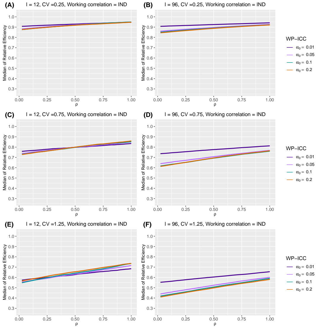
Web Figure 35 The median of relative efficiency (RE) as a function of within-period intraclass correlation coefficient (WP-ICC) \alpha_0 \in \{0.01, 0.05, 0.1, 0.2\} and the decay rate \rho \in (0, 1) , when the true correlation model is exponential decay (ED) and the working correlation model is independence (IND). Design factors considered are as follows: number of clusters I = 12 and 96, number of periods J = 5 , mean cluster-period size \bar{n} = 100 , and the degree of between-cluster imbalance is defined by coefficient of variation CV \in \{0.25, 0.75, 1.25\} . Within-cluster imbalance (pattern 3: monotonically decreasing) is introduced.
