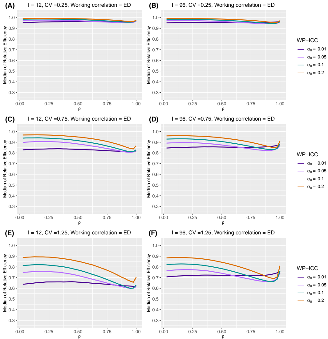
Web Figure 29 The median of relative efficiency (RE) as a function of within-period intraclass correlation coefficient (WP-ICC) \alpha_0 \in \{0.01, 0.05, 0.1, 0.2\} and the decay rate \rho \in (0, 1) , when both the true correlation model and the working correlation model are exponential decay (ED). Design factors considered are as follows: number of clusters I = 12 and 96 , number of periods J = 5 , mean cluster-period size \bar{n} = 100 , and the degree of between-cluster imbalance is defined by coefficient of variation CV \in \{0.25, 0.75, 1.25\} . Within-cluster imbalance (pattern 2: monotonically increasing) is introduced.
