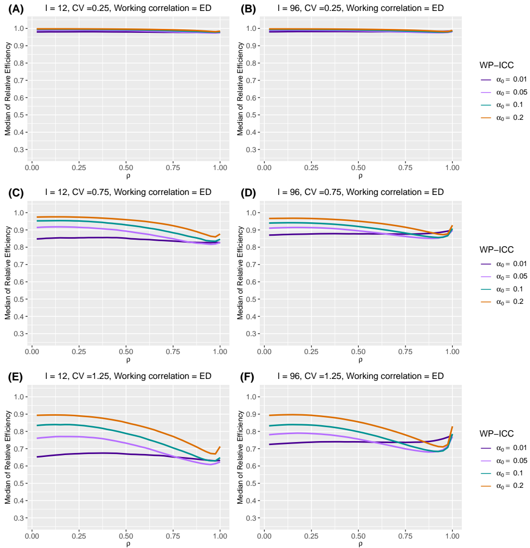
Web Figure 28 The median of relative efficiency (RE) as a function of within-period intraclass correlation coefficient (WP-ICC) \alpha_0 \in \{0.01, 0.05, 0.1, 0.2\} and the decay rate \rho \in (0, 1) , when both the true correlation model and the working correlation model are exponential decay (ED). Design factors considered are as follows: number of clusters I = 12 and 96 , number of periods J = 5 , mean cluster-period size \bar{n} = 100 , and the degree of between-cluster imbalance is defined by coefficient of variation CV \in \{0.25, 0.75, 1.25\} . Within-cluster imbalance (pattern 1: constant) is introduced.
