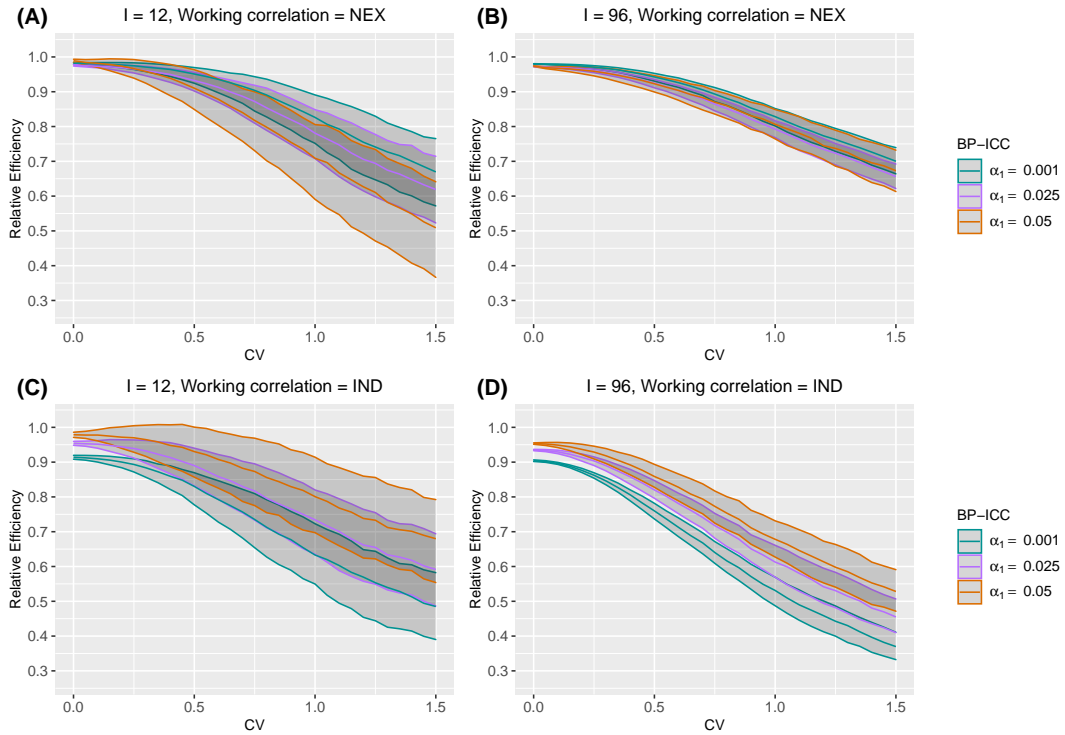
Web Figure 2 The median and interquartile range (IQR) of relative efficiency (RE) as a function of coefficient of variation (CV) measuring between-cluster imbalance, when the true correlation model is nested exchangeable (NEX). Design factors considered are as follows: number of clusters I = 12 and 96 , number of periods J = 5 . The within-period intraclass correlation coefficient (WP-ICC) \alpha_0 = 0.05 , and between-period intraclass correlation coefficient (BP-ICC) \alpha_1 \in \{0.001, 0.025, 0.05\} . The working correlation structure is either NEX or independence (IND). Within-cluster imbalance (pattern 2: monotonically increasing) is introduced.
