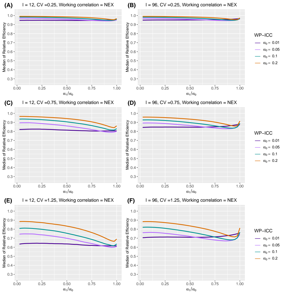
Web Figure 7 The median of relative efficiency (RE) as a function of the within-period intraclass correlation coefficient (WP-ICC) \alpha_0 \in \{0.01, 0.05, 0.1, 0.2\} and the ratio of between-period intraclass correlation coefficient (BP-ICC) to WP-ICC, \alpha_1/\alpha_0 \in [0, 1] , when both the true correlation model and the working correlation model are nested exchangeable (NEX). Design factors considered are as follows: number of clusters I = 12 and 96, number of periods J = 5 , and the degree of between-cluster imbalance is defined by CV \in \{0.25, 0.75, 1.25\} . Within-cluster imbalance (pattern 4: randomly permuted) is introduced.
