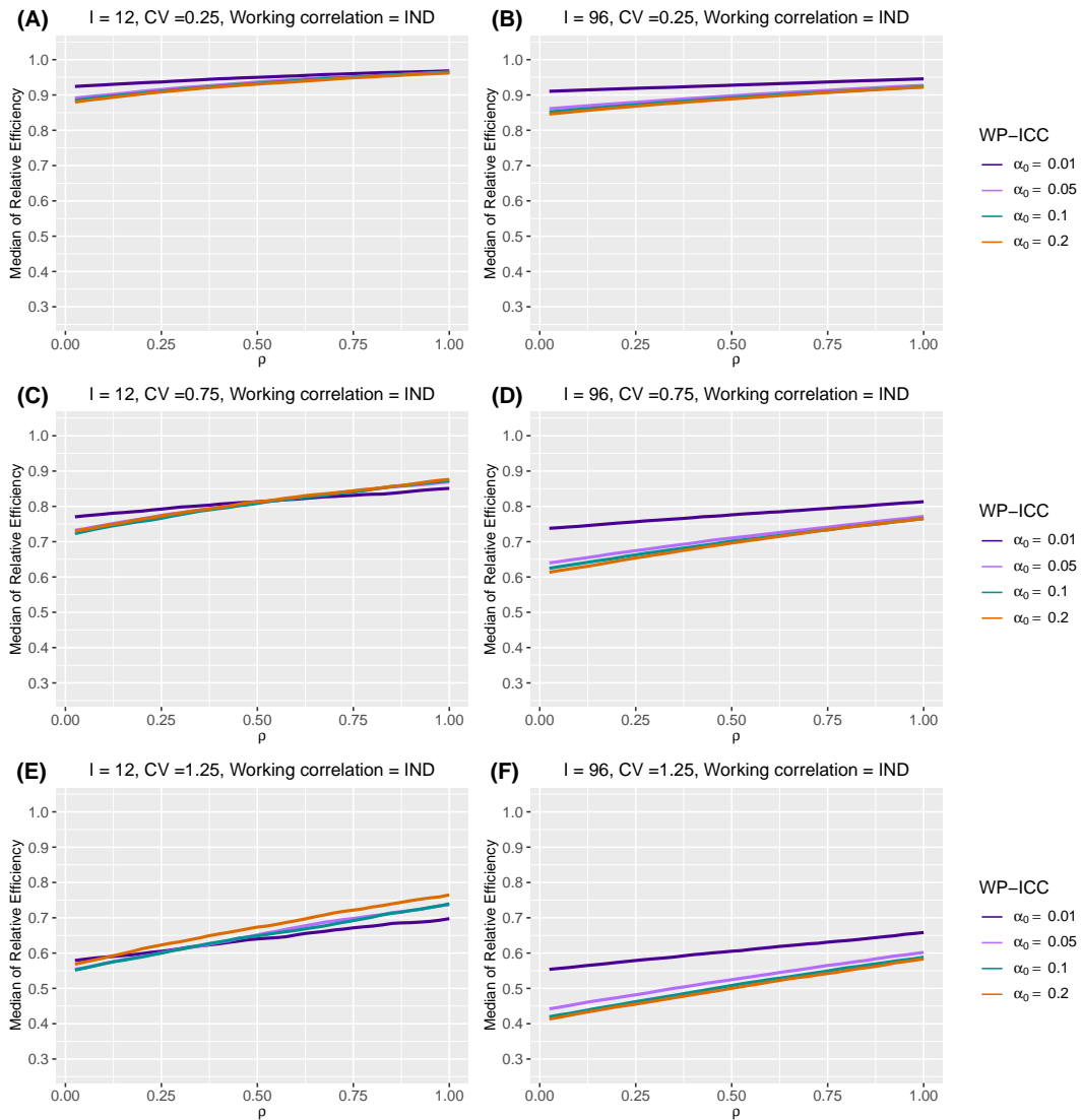
Web Figure 36 The median of relative efficiency (RE) as a function of within-period intraclass correlation coefficient (WP-ICC) \alpha_0 \in \{0.01, 0.05, 0.1, 0.2\} and the decay rate \rho \in (0, 1) , when the true correlation model is exponential decay (ED) and the working correlation model is independence (IND). Design factors considered are as follows: number of clusters I = 12 and 96, number of periods J = 5 , mean cluster-period size \bar{n} = 100 , and the degree of between-cluster imbalance is defined by coefficient of variation CV \in \{0.25, 0.75, 1.25\} . Within-cluster imbalance (pattern 4: randomly permuted) is introduced.
