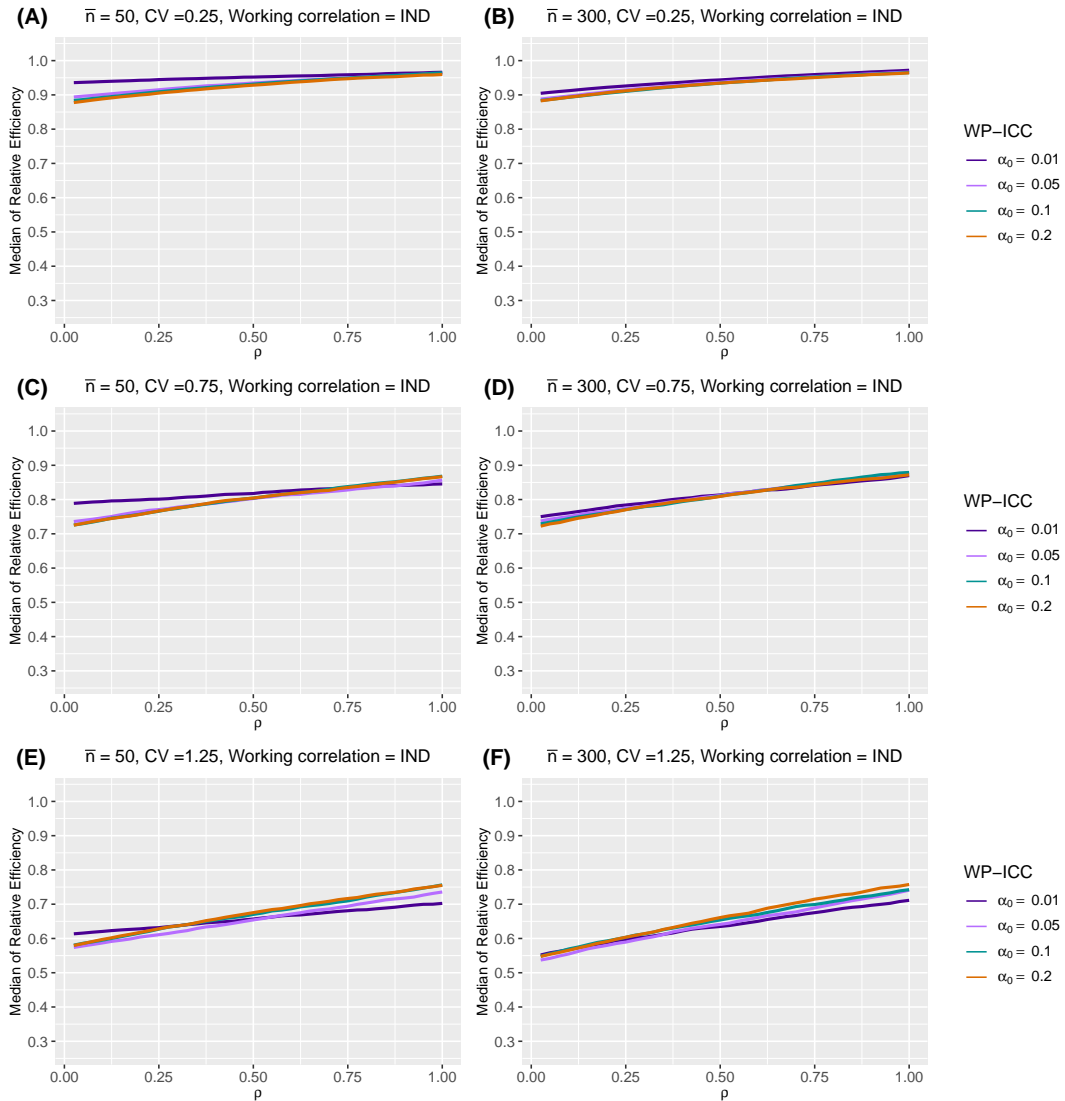
Web Figure 43 The median of relative efficiency (RE) as a function of the within-period intraclass correlation coefficient (WP-ICC) \alpha_0 \in \{0.01, 0.05, 0.1, 0.2\} and the decay rate \rho \in (0, 1) , when the true correlation model is exponential decay (ED) and the working correlation model is independence (IND). Design factors considered are as follows: number of clusters I = 12 , number of periods J = 5 , mean cluster-period sizes \bar{n} \in \{50, 300\} , and the degree of between-cluster imbalance is defined by coefficient of variation CV \in \{0.25, 0.75, 1.25\} . Within-cluster imbalance (pattern 4: randomly permuted) is introduced.
