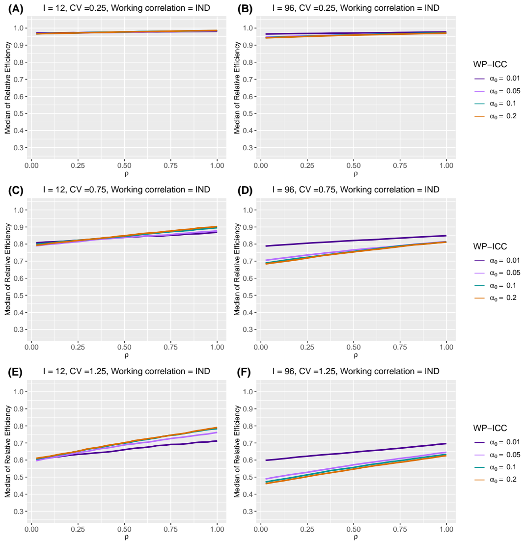
Web Figure 33 The median of relative efficiency (RE) as a function of within-period intraclass correlation coefficient (WP-ICC) \alpha_0 \in \{0.01, 0.05, 0.1, 0.2\} and the decay rate \rho \in (0, 1) , when the true correlation model is exponential decay (ED) and the working correlation model is independence (IND). Design factors considered are as follows: number of clusters I = 12 and 96 , number of periods J = 5 , mean cluster-period size \bar{n} = 100 , and the degree of between-cluster imbalance is defined by coefficient of variation CV \in \{0.25, 0.75, 1.25\} . Within-cluster imbalance (pattern 1: constant) is introduced.
