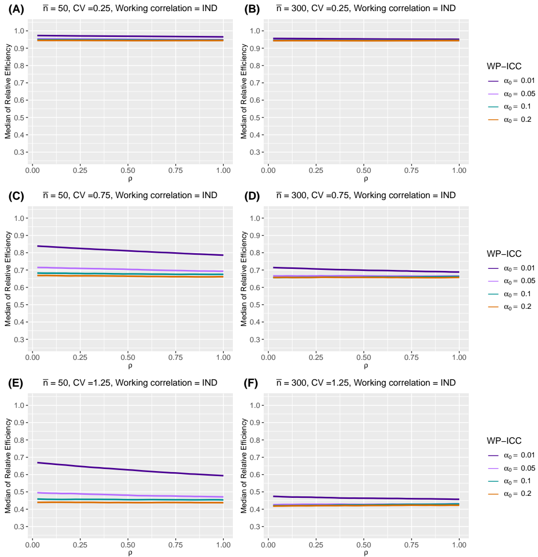
Web Figure 42 The median of relative efficiency (RE) as a function of the within-period intraclass correlation coefficient (WP-ICC) \alpha_0 \in \{0.01, 0.05, 0.1, 0.2\} and the decay rate \rho \in (0, 1) , when the true correlation model is exponential decay (ED) and the working correlation model is independence (IND). Design factors considered are as follows: number of clusters I = 96 , number of periods J = 5 , mean cluster-period sizes \bar{n} \in \{50, 300\} , and the degree of between-cluster imbalance is defined by coefficient of variation CV \in \{0.25, 0.75, 1.25\} . No within-cluster imbalance is introduced.
