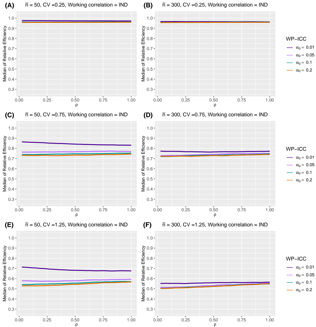
Web Figure 41 The median of relative efficiency (RE) as a function of the within-period intraclass correlation coefficient (WP-ICC) \alpha_0 \in \{0.01, 0.05, 0.1, 0.2\} and the decay rate \rho \in (0, 1) , when the true correlation model is exponential decay (ED) and the working correlation model is independence (IND). Design factors considered are as follows: number of clusters I = 12 , number of periods J = 5 , mean cluster-period sizes \bar{n} \in \{50, 300\} , and the degree of between-cluster imbalance is defined by coefficient of variation CV \in \{0.25, 0.75, 1.25\} . No within-cluster imbalance is introduced.
