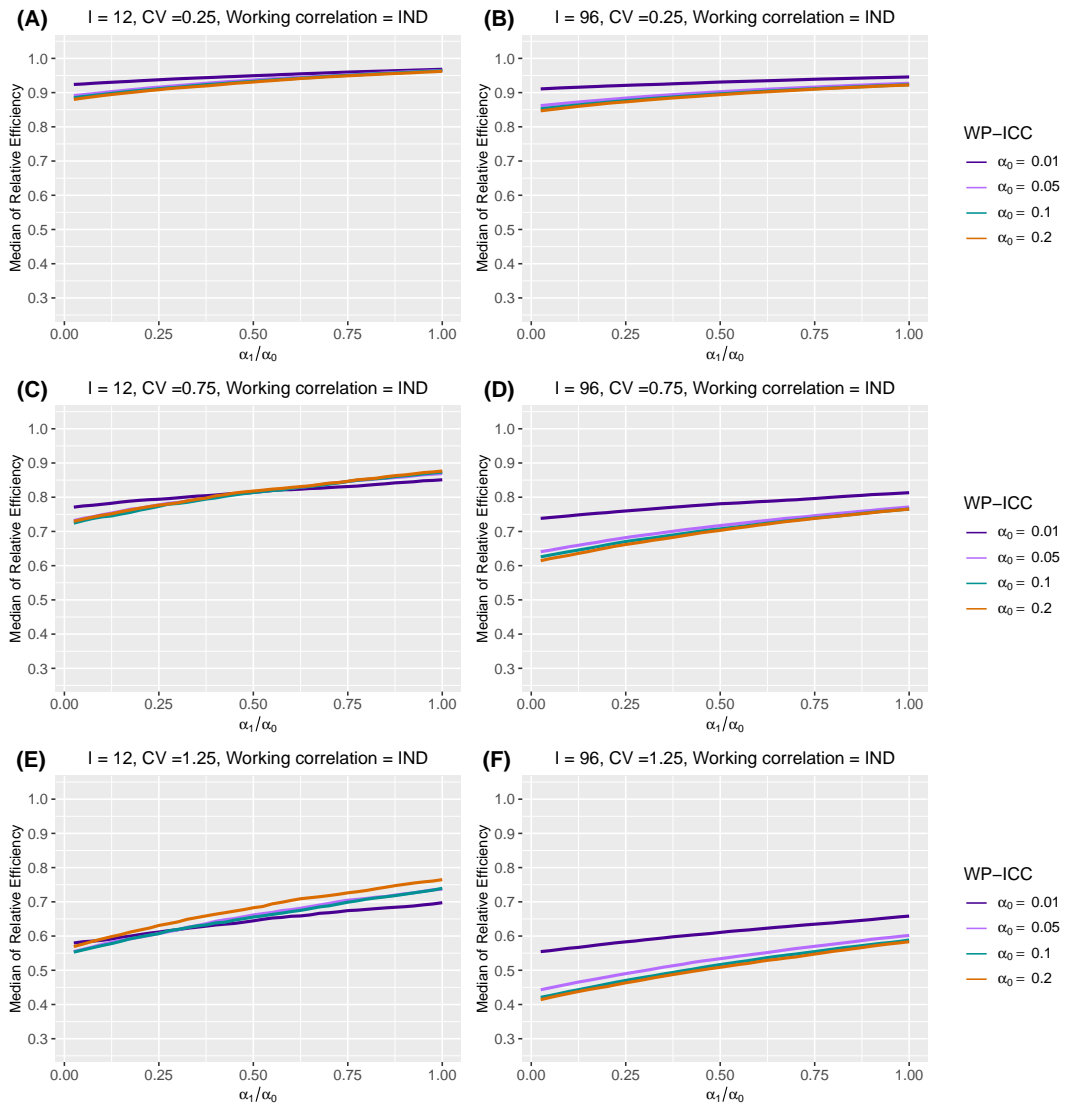
Web Figure 9 The median of relative efficiency (RE) as a function of the within-period intraclass correlation coefficient (WP-ICC) \alpha_0 \in \{0.01, 0.05, 0.1, 0.2\} and the ratio of between-period intraclass correlation coefficient (BP-ICC) to WP-ICC, \alpha_1/\alpha_0 \in [0, 1] , when the true correlation model is nested exchangeable (NEX) and the working correlation model is independence (IND). Design factors considered are as follows: number of clusters I = 12 and 96 , number of periods J = 5 , and the degree of between-cluster imbalance is defined by CV \in \{0.25, 0.75, 1.25\} . Within-cluster imbalance (pattern 2: monotonically increasing) is introduced.
