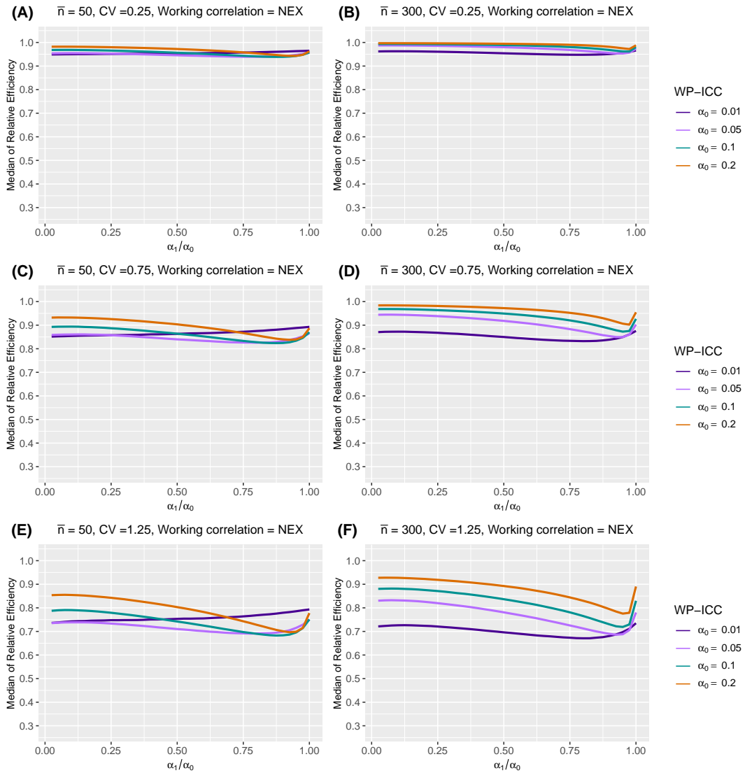
Web Figure 16 The median of relative efficiency (RE) as a function of the within-period intraclass correlation coefficient (WP-ICC) \alpha_0 \in \{0.01, 0.05, 0.1, 0.2\} and the ratio of between-period intraclass correlation coefficient (BP-ICC) to WP-ICC, \alpha_1/\alpha_0 \in [0, 1] , when both the true correlation model and the working correlation model are nested exchangeable (NEX). Design factors considered are as follows: number of clusters I = 96 , number of periods J = 5 , mean cluster-period sizes \bar{n} \in \{50, 300\} , and the degree of between-cluster imbalance is defined by coefficient of variation CV \in \{0.25, 0.75, 1.25\} . Within-cluster imbalance (pattern 4: randomly permuted) is introduced.
