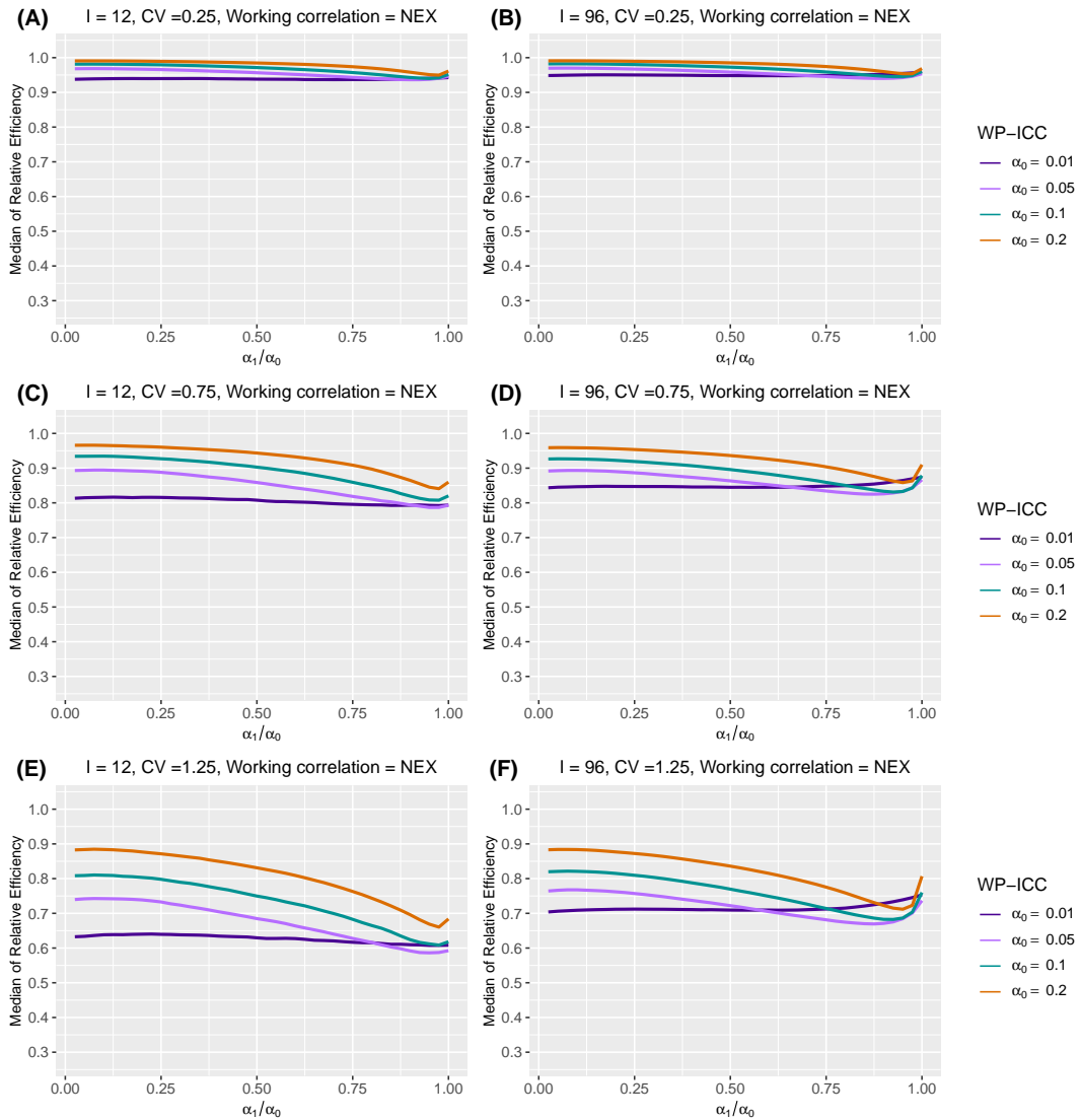
Web Figure 6 The median of relative efficiency (RE) as a function of the within-period intraclass correlation coefficient (WP-ICC) \alpha_0 \in \{0.01, 0.05, 0.1, 0.2\} and the ratio of between-period intraclass correlation coefficient (BP-ICC) to WP-ICC, \alpha_1/\alpha_0 \in [0, 1] , when both the true correlation model and the working correlation model are nested exchangeable (NEX). Design factors considered are as follows: number of clusters I = 12 and 96 , number of periods J = 5 , and the degree of between-cluster imbalance is defined by CV \in \{0.25, 0.75, 1.25\} . Within-cluster imbalance (pattern 3: monotonically decreasing) is introduced.
