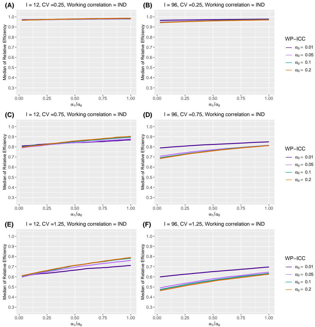
Web Figure 8 The median of relative efficiency (RE) as a function of the within-period intraclass correlation coefficient (WP-ICC) \alpha_0 \in \{0.01, 0.05, 0.1, 0.2\} and the ratio of between-period intraclass correlation coefficient (BP-ICC) to WP-ICC, \alpha_1/\alpha_0 \in [0, 1] , when the true correlation model is nested exchangeable (NEX) and the working correlation model is independence (IND). Design factors considered are as follows: number of clusters I = 12 and 96 , number of periods J = 5 , and the degree of between-cluster imbalance is defined by CV \in \{0.25, 0.75, 1.25\} . Within-cluster imbalance (pattern 1: constant) is introduced.
