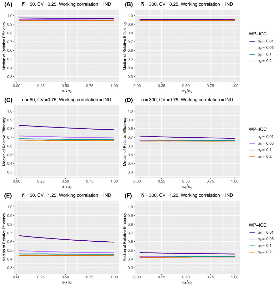
Web Figure 18 The median of relative efficiency (RE) as a function of the within-period intraclass correlation coefficient (WP-ICC) \alpha_0 \in \{0.01, 0.05, 0.1, 0.2\} and the ratio of between-period intraclass correlation coefficient (BP-ICC) to WP-ICC, \alpha_1/\alpha_0 \in [0, 1] , when the true correlation model is nested exchangeable (NEX) and the working correlation model is independence (IND). Design factors considered are as follows: number of clusters I = 96 , number of periods J = 5 , mean cluster-period sizes \bar{n} \in \{50, 300\} , and the degree of between-cluster imbalance is defined by coefficient of variation CV \in \{0.25, 0.75, 1.25\} . No within-cluster imbalance is introduced.
