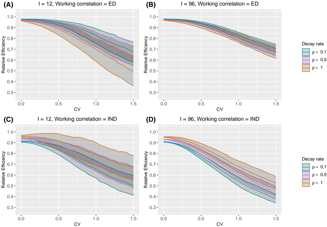
Web Figure 25 The median and interquartile range (IQR) of relative efficiency (RE) as a function of coefficient of variation (CV) measuring between-cluster imbalance, when the true correlation model is exponential decay. Design factors considered are as follows: number of clusters I = 12 and 96 , number of periods J = 5 . The within-period intraclass correlation coefficient (WP-ICC) \alpha_0 = 0.05 , and decay rate \rho \in \{0.1, 0.5, 1\} . Within-cluster imbalance (pattern 3: monotonically decreasing) is introduced.
