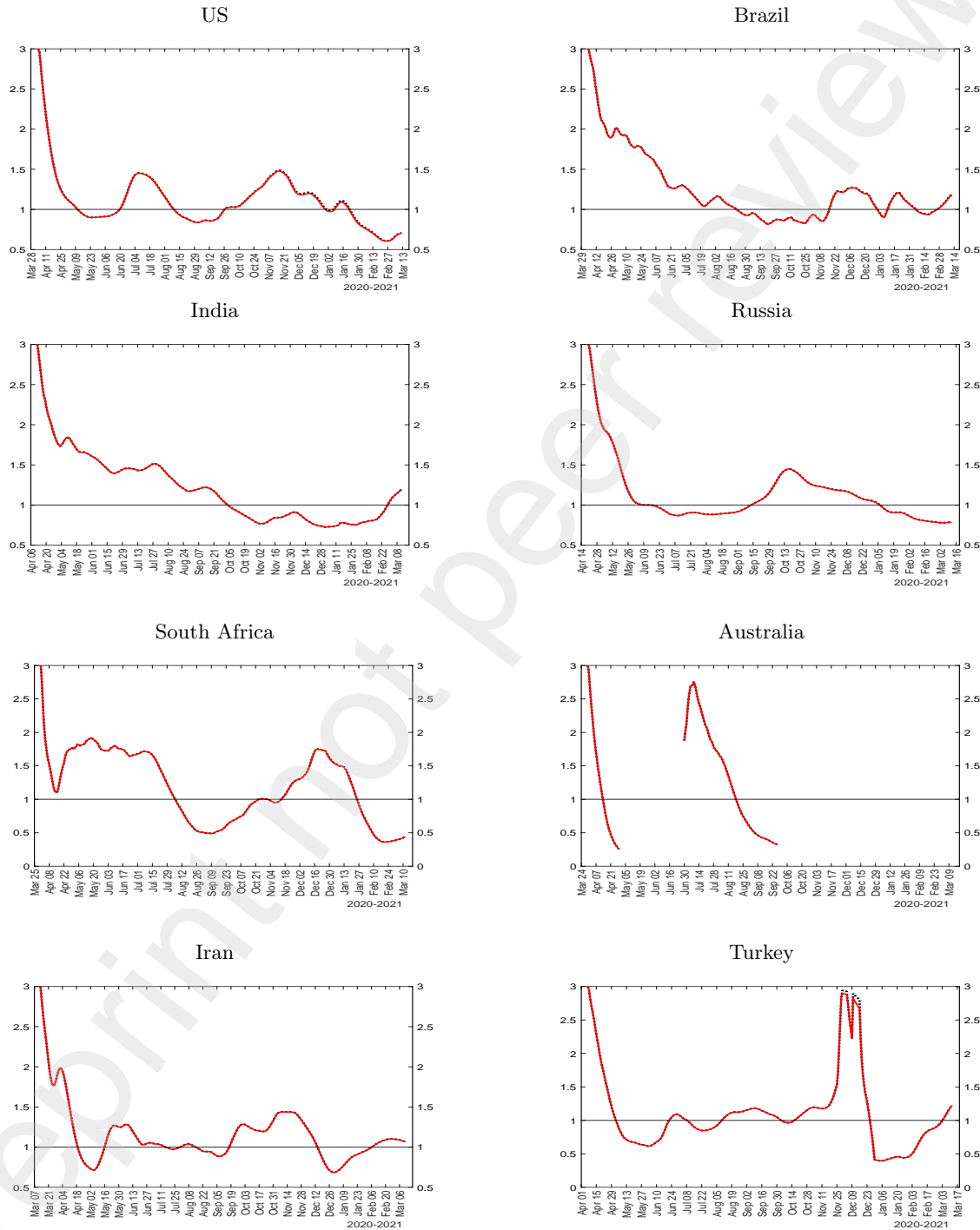
Figure A.4: Comparisons of estimated \mathcal{R} numbers for selected countries for two choices of multiplication factors, MF=5 (solid red line) and MF=3 (dotted black line)
