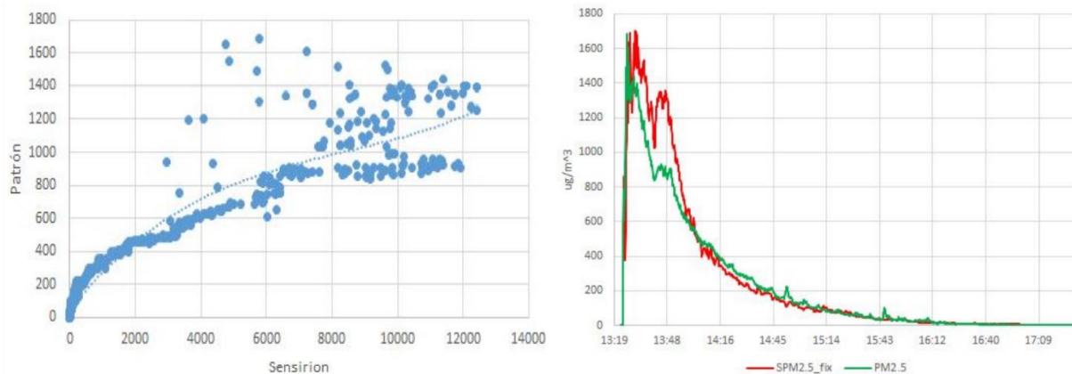
Figure S3. (left) Calibration curve for PM 2.5 concentrations between Sensirion SPS30 sensors (x-axis) and Grimm laser aerosol spectrometer 11-E (y-axis) (right) Corrected Sensirion SPS30 sensor PM 2.5 measurements (SPM2.5_fix) alongside Grimm laser aerosol spectrometer 11-E PM 2.5 concentrations (PM2.5)
