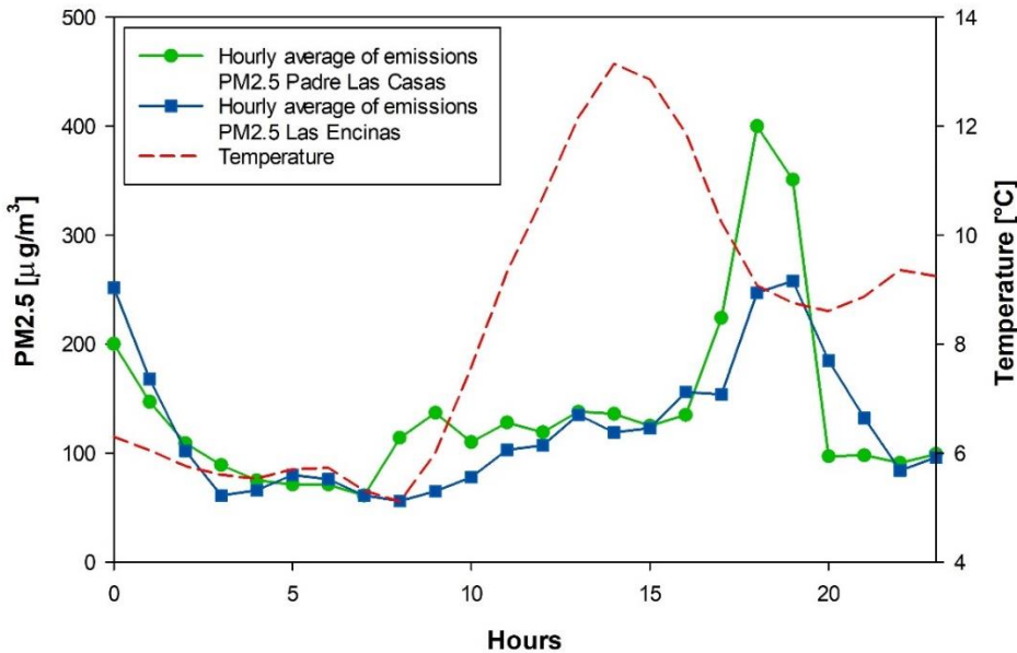
Figure S2. Example of average hourly PM 2.5 concentrations and temperatures at Las Encinas and Padre Las Casas (May 25, 2019)
