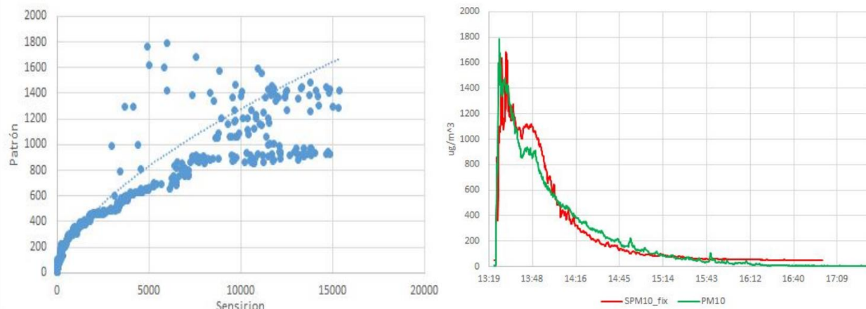
Figure S4. (left) Calibration curve for PM 10 concentrations between Sensirion SPS30 sensors (x-axis) and Grimm laser aerosol spectrometer 11-E (y-axis) (right) Corrected Sensirion SPS30 sensor PM 10 measurements (PM10_fix) alongside Grimm laser aerosol spectrometer 11-E PM 10 concentrations (PM10)
