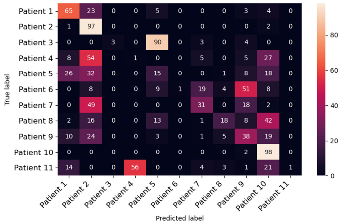
Supplementary Figure 2: Confusion matrix for patient prediction. Each row shows the true labels while the columns show the predicted labels. The diagonal indicates correct predictions.
