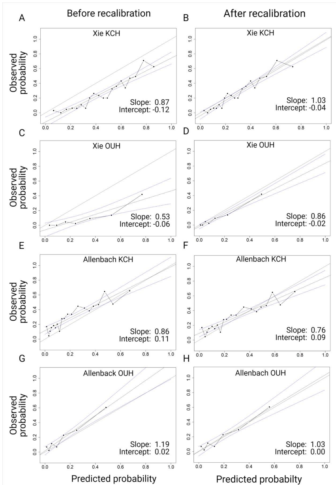
Figure S3: Results for calibration of the Xie and Allenbach models at KCH and OUH before and after recalibration
