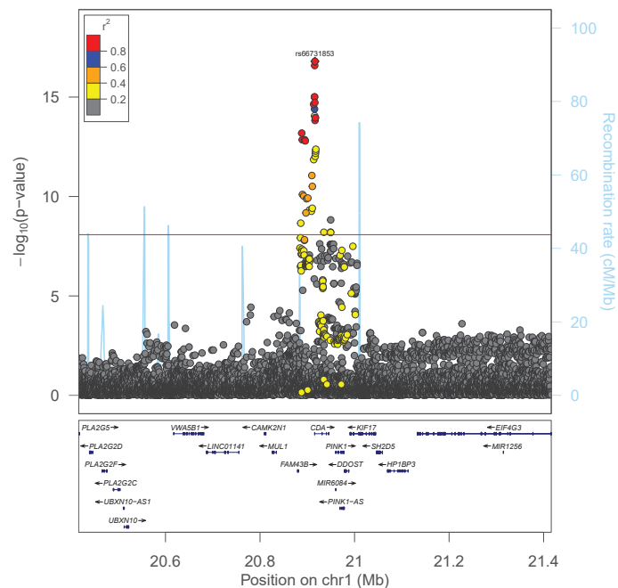
Supplementary Figure 3. regional association plots for GWAS sentinels.
