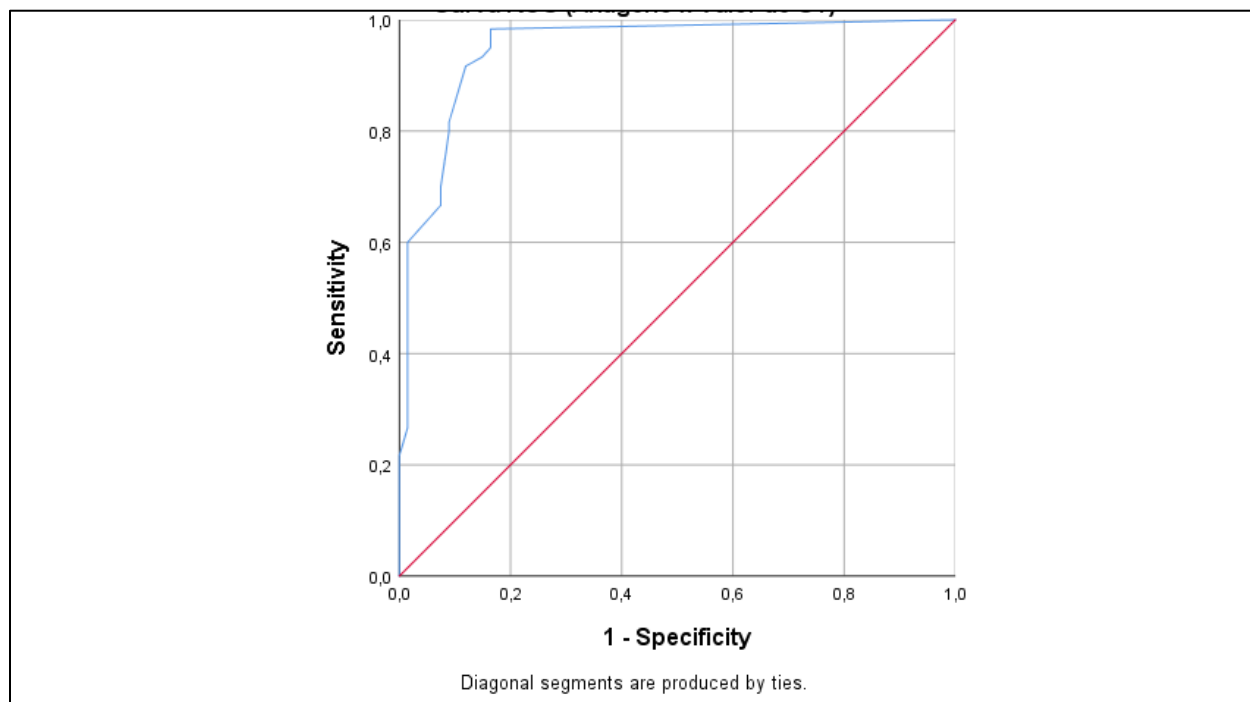
Figure 1: ROC Curve: Panbio™ COVID-19 Ag test results versus Ct
