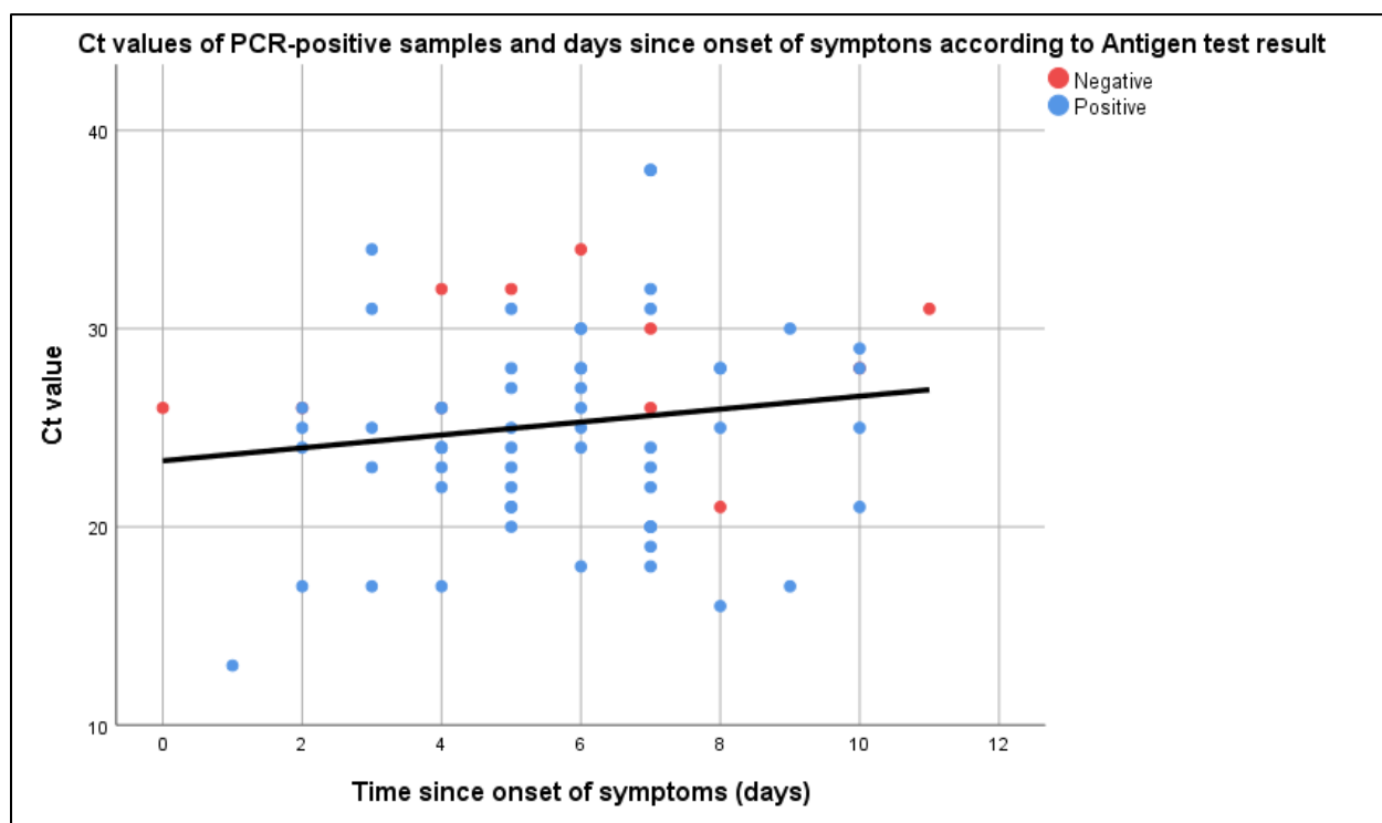
Figure 2: Ct Values of PCR-Positive Samples versus Days Post Onset of Symptoms
