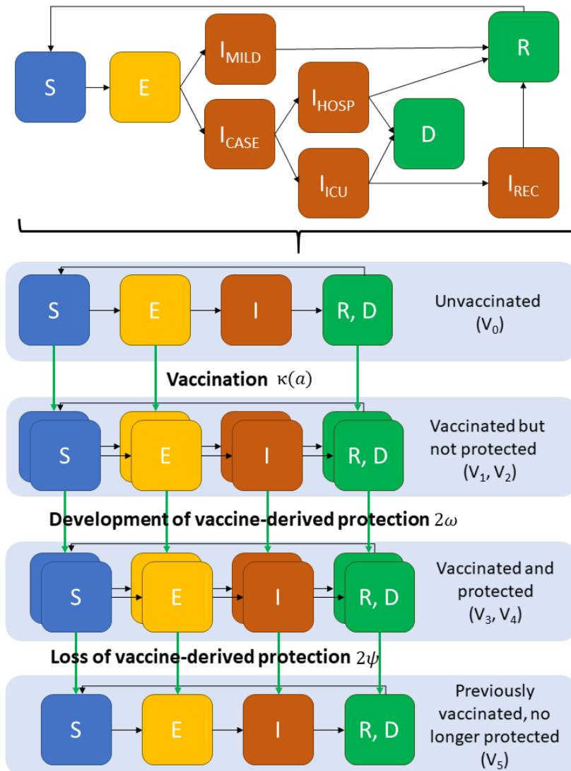
Figure S1: Schematic of the SARS-CoV-2 transmission model. The schematic in the upper section is based on the model in Walker et al. 1 Individuals in the susceptible (S), exposed (E) and recovered (R) compartments can be vaccinated. Vaccination status is stratified into 6 categories – those who are unvaccinated ( v_0 ), those who have recently been vaccinated but are not yet protected ( v_1 and v_2 ) and those who are vaccinated and protected ( v_3 and v_4 ) and those that have previously been vaccinated but are no longer protected ( v_5 ). Protection may refer to partial protection. We do not model revaccination of previously vaccinated individuals, due to all vaccination occurring within a one-month period. Pathways for receiving healthcare for the proportions of the population in the I_{HOSPITAL} and I_{ICU} compartments are described in Walker et al. 1
