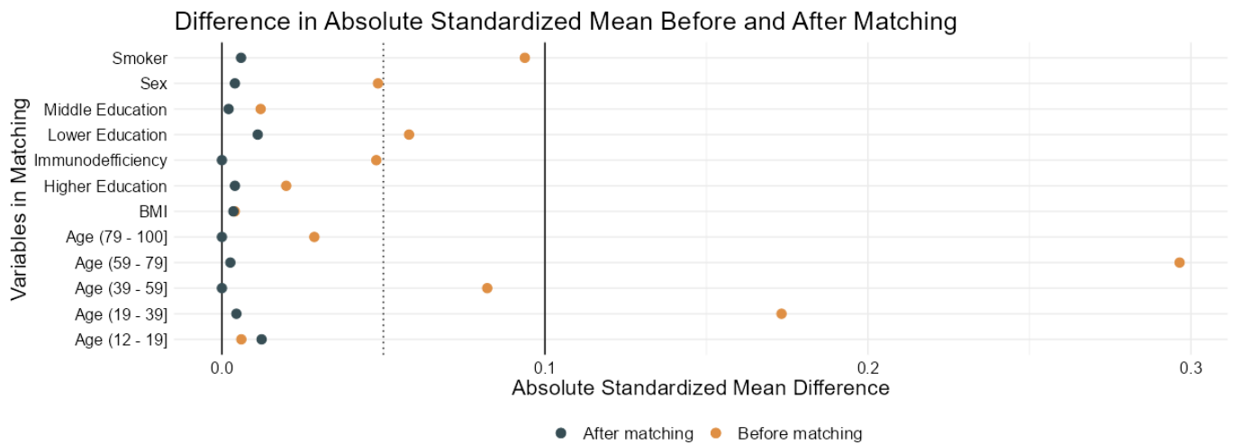
eFigure 1. Standardized mean difference before (orange dots) and after (black dots) propensity score matching. A difference of less than 0.1 considered to be acceptable.
