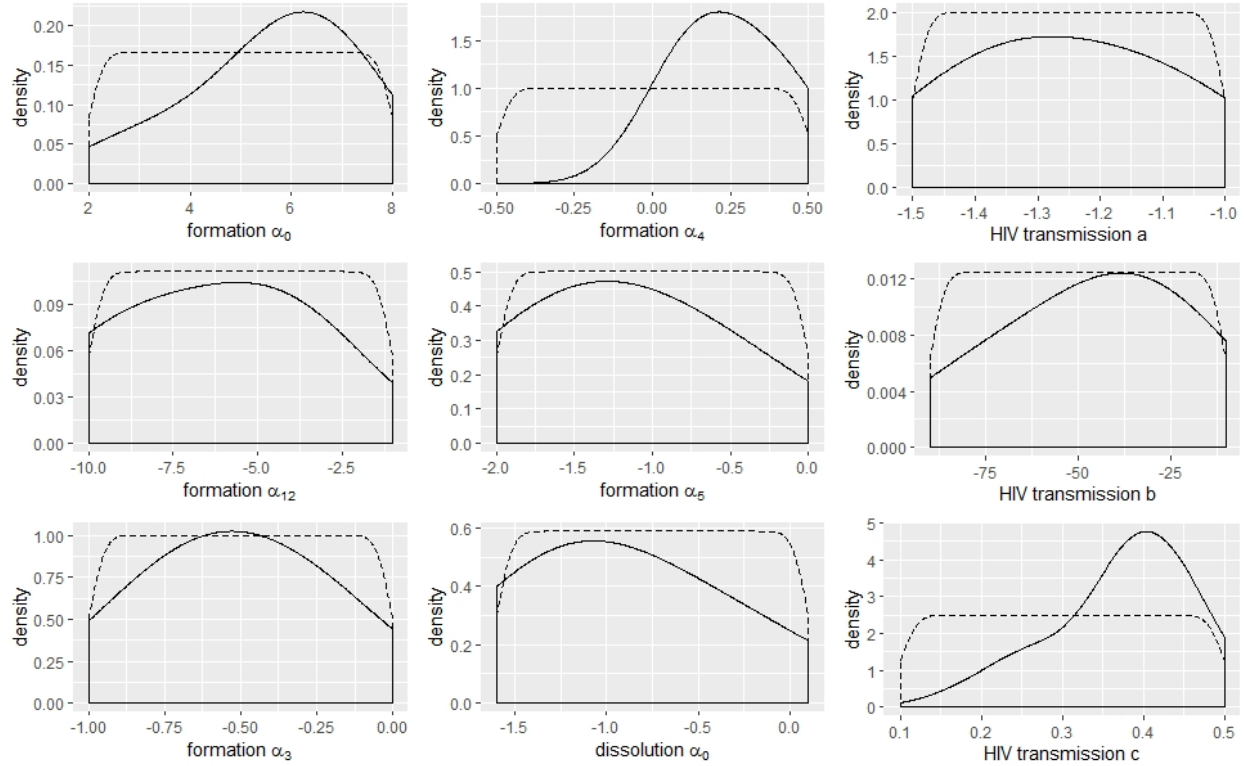
Figure S9. Analysis of the parameter space for the STI-BC model. Smoothed density plots for the initial uniform distribution (dashed line) and the distribution of the top 1% solutions (solid line) for the nine estimated parameters.
