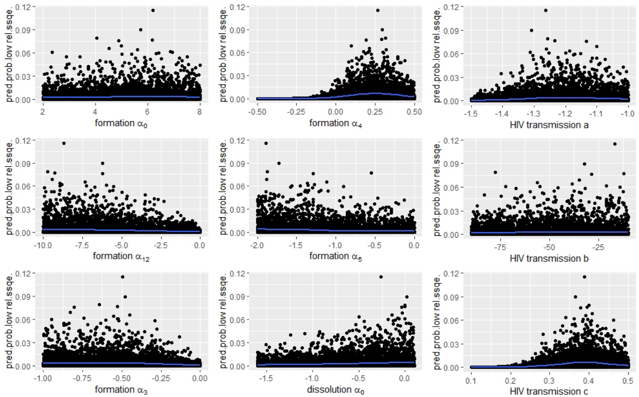
Figure S6. Analysis of the parameter space for the STI-nBC model. Results of the GAM: predicted probabilities of low relative sum of squared errors (SSE) for the nine estimated parameters.
