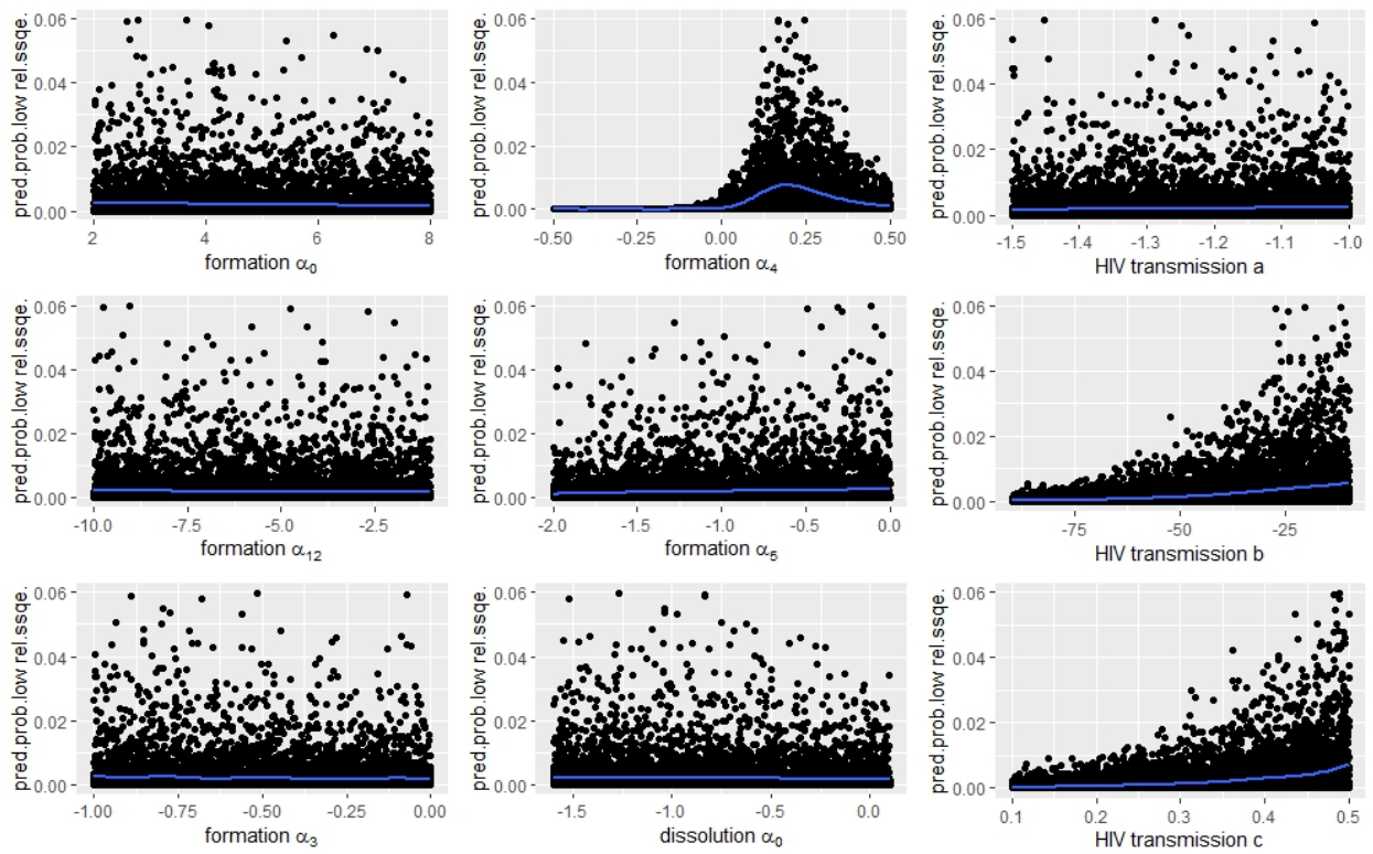
Figure S8. Analysis of the parameter space for the nSTI-BC model. Results of the GAM: predicted probabilities of low relative sum of squared errors (SSE) for the nine estimated parameters.
