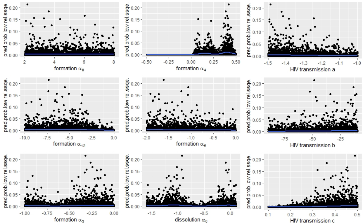
Figure S4. Analysis of the parameter space for the nSTI-nBC model. Results of the GAM: predicted probabilities of low relative sum of squared errors (SSE) for the nine estimated parameters.
