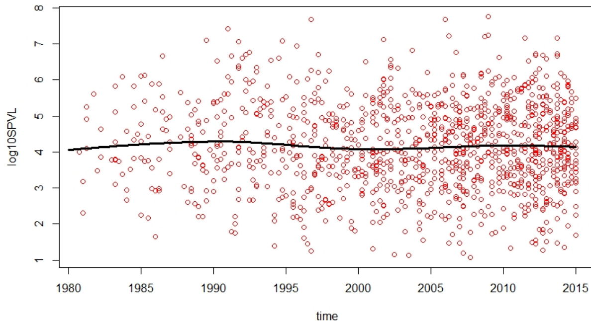
Figure S11. First HIV RNA at 9-27 months after seroconversion for each person with date of seroconversion between 1980 and 2015 (red dots) for a single simulation. Black line: cubic spline fitted through the red dots, representing the mean log 10 SPVL over time.
