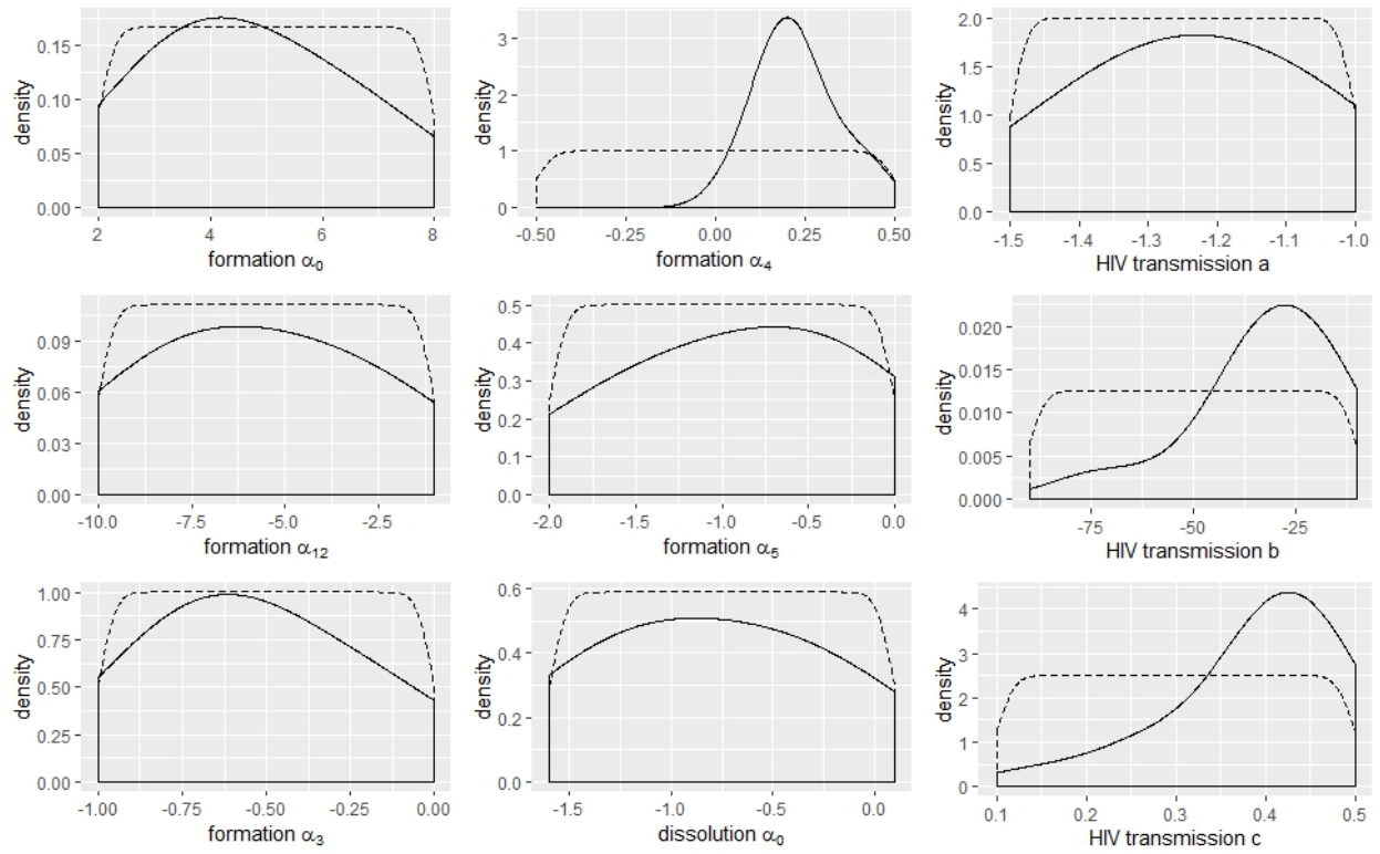
Figure S7. Analysis of the parameter space for the nSTI-BC model. Smoothed density plots for the initial uniform distribution (dashed line) and the distribution of the top 1% solutions (solid line) for the nine estimated parameters.
