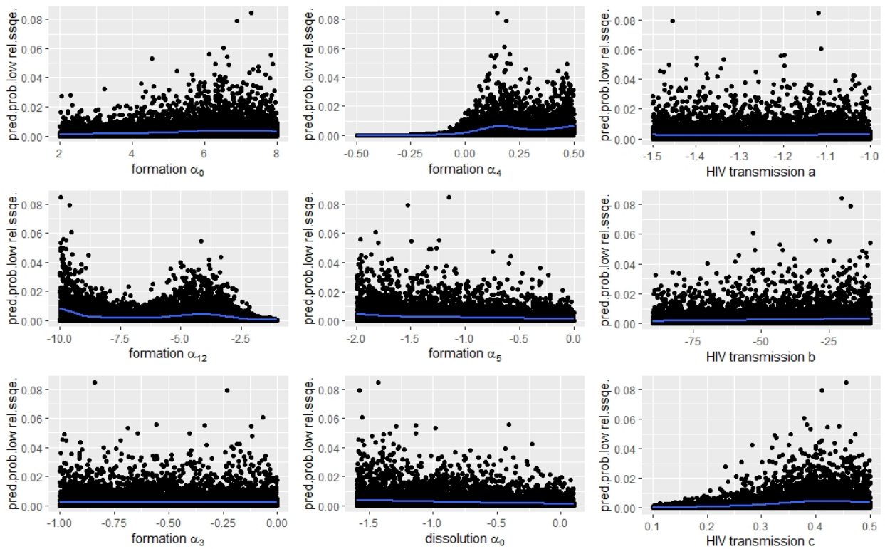
Figure S10. Analysis of the parameter space for the STI-BC model. Results of the GAM: predicted probabilities of low relative sum of squared errors (SSE) for the nine estimated parameters.
