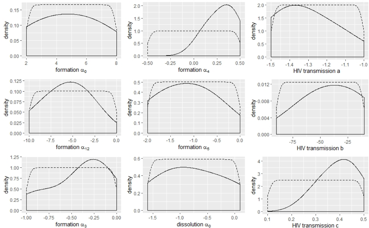
Figure S3. Analysis of the parameter space for the nSTI-nBC model. Smoothed density plots for the initial uniform distribution (dashed line) and the distribution of the top 1% solutions (solid line) for the nine estimated parameters.
