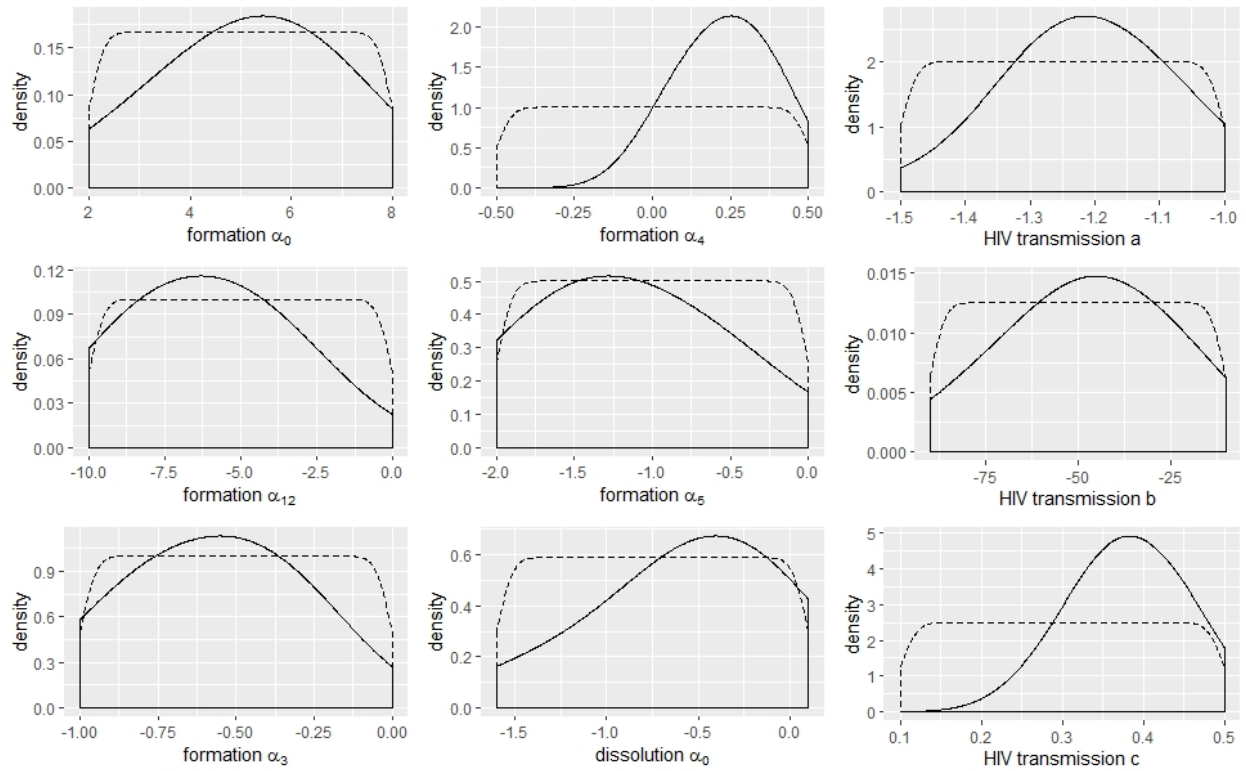
Figure S5. Analysis of the parameter space for the STI-nBC model. Smoothed density plots for the initial uniform distribution (dashed line) and the distribution of the top 1% solutions (solid line) for the nine estimated parameters.
