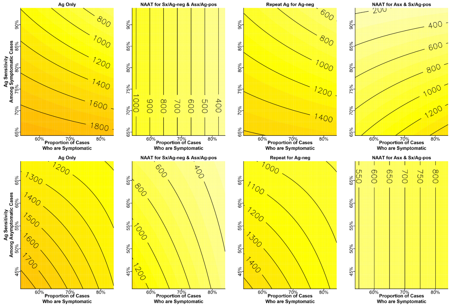
Supplementary Figure 3. Missed Cases per 100,000 Persons Tested as a Function of Antigen Test Sensitivity and the Prevalence of Symptoms Among Cases in a Population of 5% SARS-CoV-2 Prevalence.
