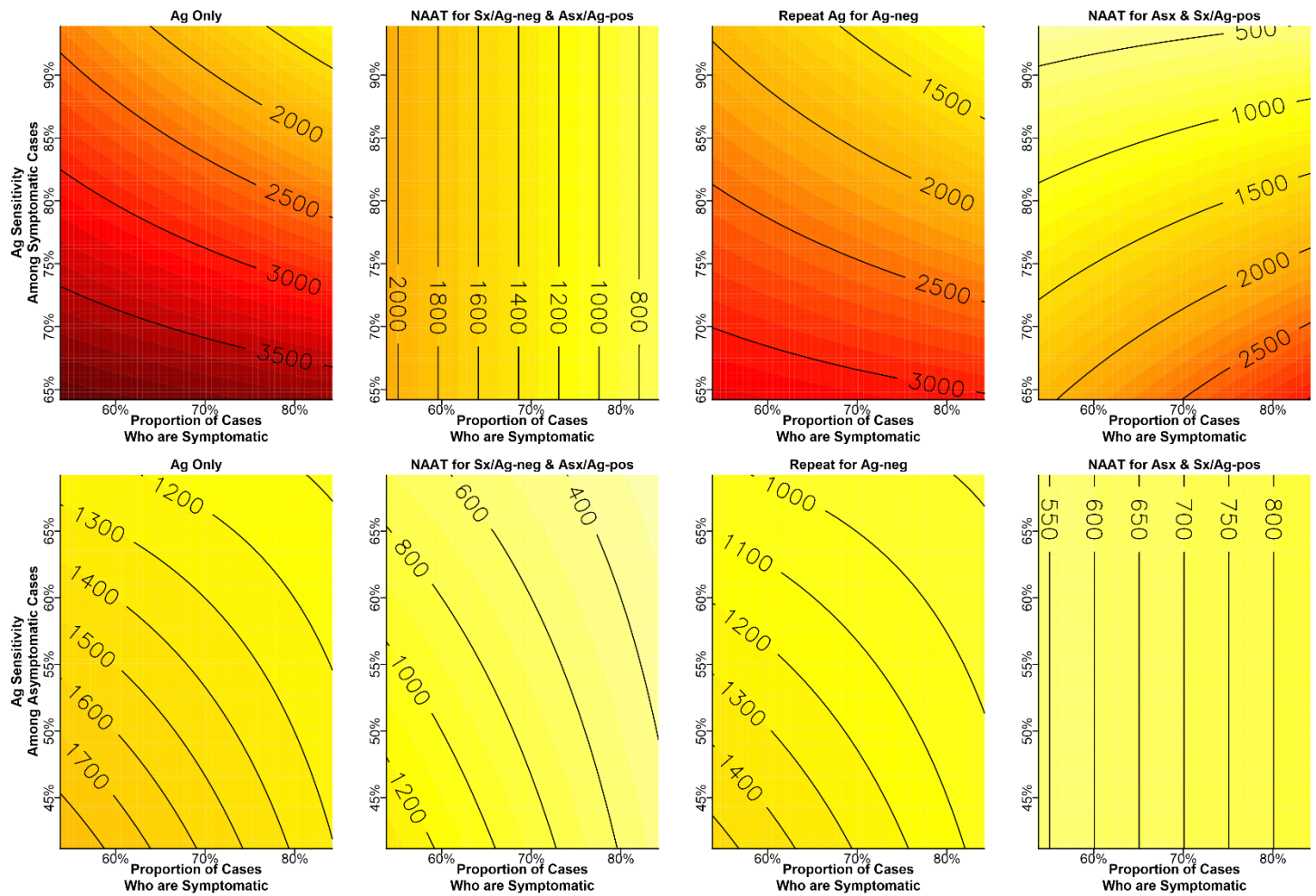
Supplementary Figure 4. Missed Cases per 100,000 Persons Tested as a Function of Antigen Test Sensitivity and the Prevalence of Symptoms Among Cases in a Population of 10% SARS-CoV-2 Prevalence.
