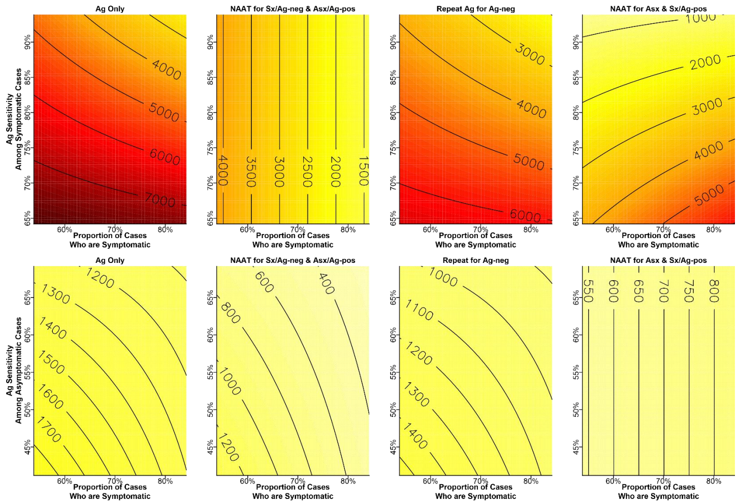
Supplementary Figure 6. Missed Cases per 100,000 Persons Tested as a Function of Antigen Test Sensitivity and the Prevalence of Symptoms Among Cases in a Population of 20% SARS-CoV-2 Prevalence.
