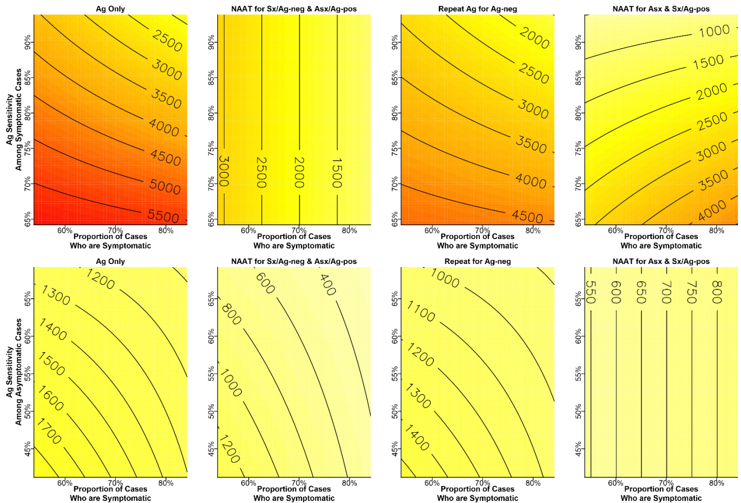
Supplementary Figure 5. Missed Cases per 100,000 Persons Tested as a Function of Antigen Test Sensitivity and the Prevalence of Symptoms Among Cases in a Population of 15% SARS-CoV-2 Prevalence.
