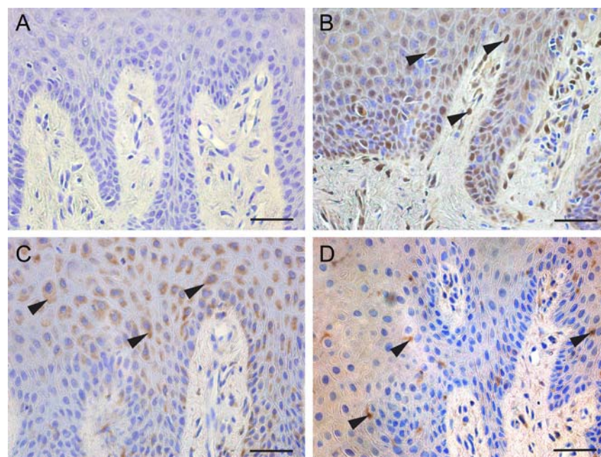
Fig. 1 Immunohistochemistry for CYLD, A20 and OTULIN on sections from gingival tissue. a The negative control of immunohistochemistry. b CYLD staining in gingival tissue. Arrows show positive staining for CYLD. c A20 staining in gingival tissue. Arrows show positive staining for A20. d OTULIN staining in gingival tissue. Arrows show positive staining for OTULIN. Scale bar, 50 \mu m
