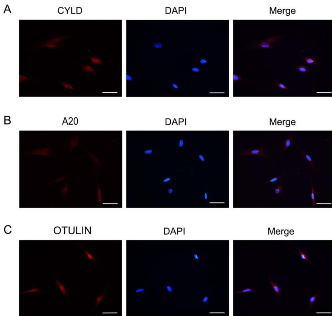
Fig. 2 Immunofluorescence staining for CYLD (a), A20 (b) and OTULIN (c) in HGFs.
