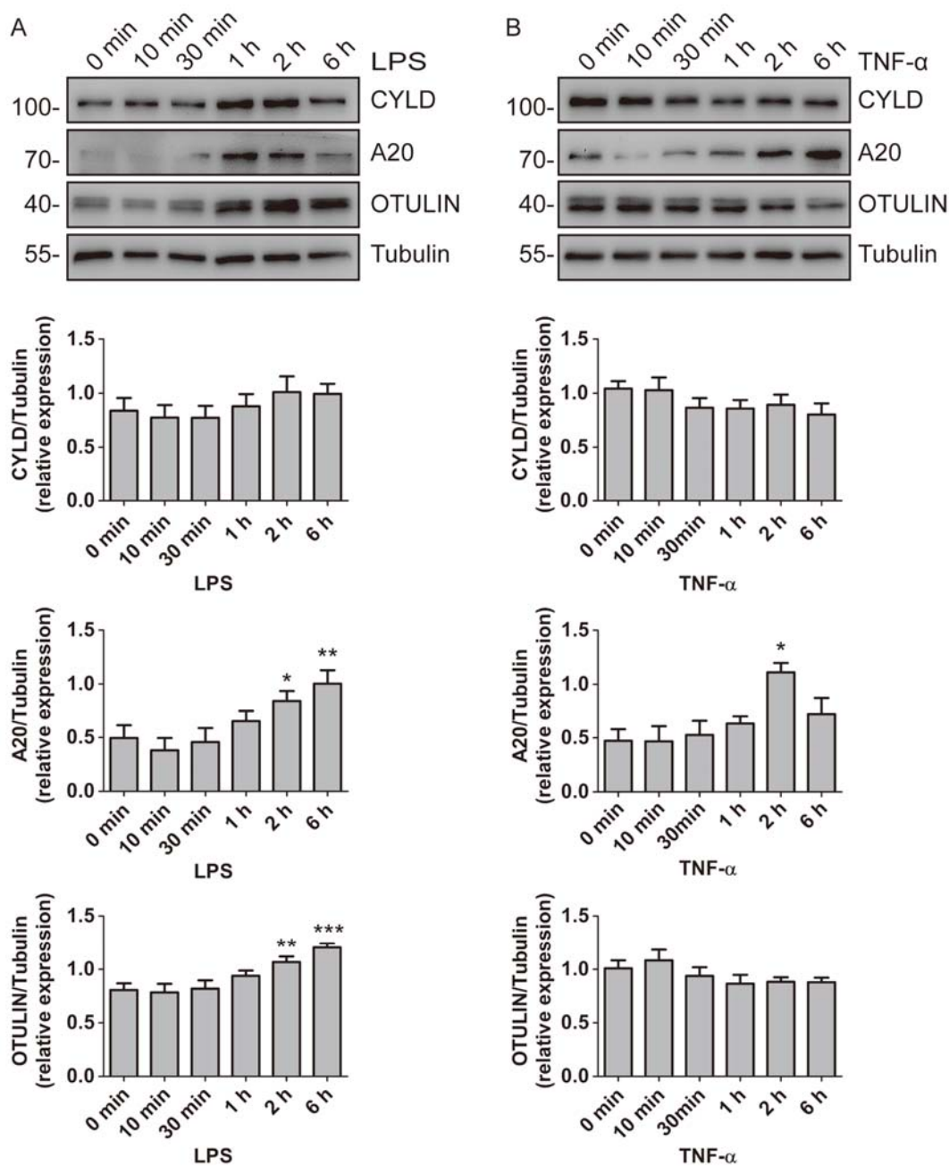
Fig. 4 Protein expression of CYLD, A20 and OTULIN in HGFs pretreated with LPS (a) or TNF- \alpha (b) for the indicated periods of time. Below, quantification of the band intensity results, presented relative to Tubulin. * P <0.05, ** P <0.01, *** P <0.001, 0 h versus 2h or 6h, one-way ANOVA with Dunnett's multiple comparison test. Data presented are from three independent experiments
