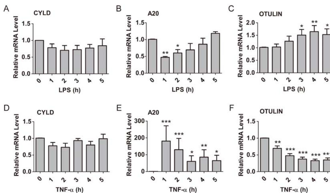
Fig. 3 mRNA levels of CYLD, A20 and OTULIN in HGFs pretreated with LPS (a, b, c) or TNF- \alpha (d, e, f) for the indicated periods of time. * P <0.05, ** P <0.01, *** P <0.001, 0 h versus 1h, 2h, 3h, 4h or 5 h, one-way ANOVA with Dunnett's multiple comparison test. Data presented are from three independent experiments
