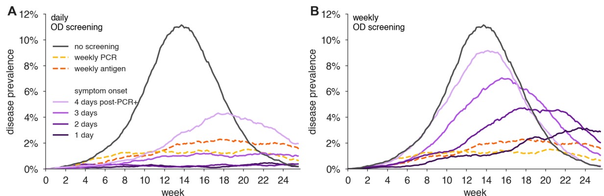
Figure S2: Impact of the timing of olfactory dysfunction onset on its effectiveness to limit viral spread. Example of viral spread in fully-mixed community of 20,000 individuals performing olfactory dysfunction (OD) screening daily (A) or weekly (B). olfactory dysfunction is modeled to be present in 75% of infected individuals, and to last 7 days. We consider 80% participation in testing and that 20% of individuals would suffer COVID-19-independent olfactory dysfunction which would exclude them from effective testing. Timing of olfactory dysfunction is varied from one to four days after virions levels reaching 1000 virions/ml (purple shaded lines as indicated). No mitigation is shown as black line. For comparison, weekly RT-PCR testing with a one day turnaround is shown.
