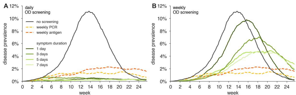
Figure S3: Impact of duration of olfactory dysfunction on its effectiveness to limit viral spread. Examples of viral spread in fully-mixed community of 20,000 individuals performing olfactory dysfunction (OD) screening daily (A) or weekly (B). Olfactory dysfunction is modeled to be present in 75% of infected individuals, and to begin two days after virion levels reach 1000 virions/ml. We consider 80% participation in testing and that 20% of individuals would suffer COVID-19-independent olfactory dysfunction which would exclude them from effective testing. Duration of olfactory dysfunction is varied from 7 days (lightest green), 5 days (light green), 3 days (green), to 1 day (dark green). No mitigation is shown as black line. For comparison, weekly RT-PCR testing with a one day turnaround is shown.
