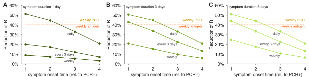
Figure 4: Impact of the timing of onset and duration of olfactory dysfunction on its effectiveness to limit viral spread. Reductions of the reproductive number R by testing daily, every third day, or weekly for olfaction dysfunction are shown for olfactory dysfunction lasting (A) one day, (B) three days, and (C) five days, for varying symptom onset times, relative to when viral levels reach \sim 1000 virions/ml. We consider 80% participation in testing and 75% prevalence of olfactory dysfunction as a COVID-19 symptom, and 20% COVID-19-independent olfactory dysfunction in all panels.
