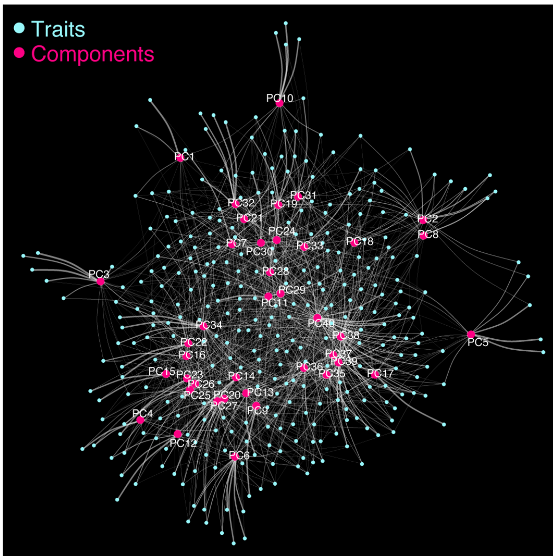
Extended Data Figure 13 | Network representation of the TSVD analysis.
