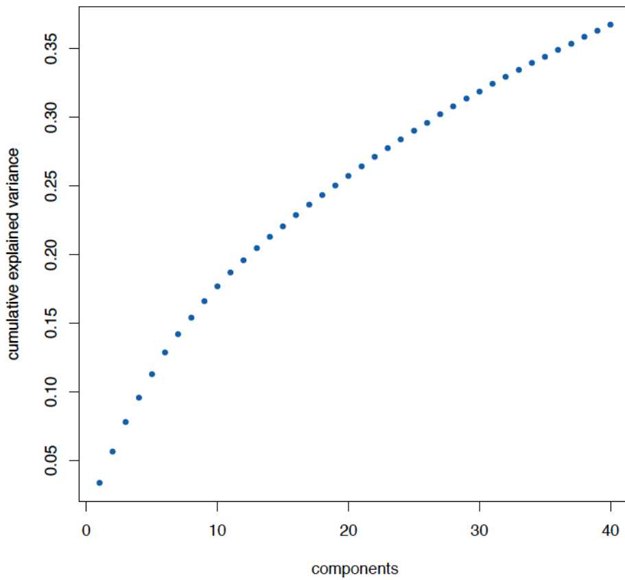
Extended Data Figure 12 | A scree plot from the decomposition of summary statistics.
