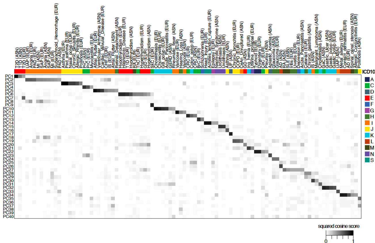
Extended Data Figure 15 | Heatmap representation of squared cosine scores of diseases to components.
