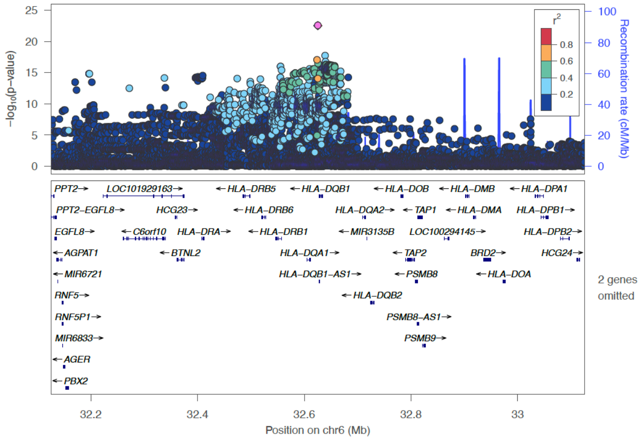
Extended Data Figure 2 | Locus plot for Pulmonary Tuberculosis (PTB) in BBJ.
