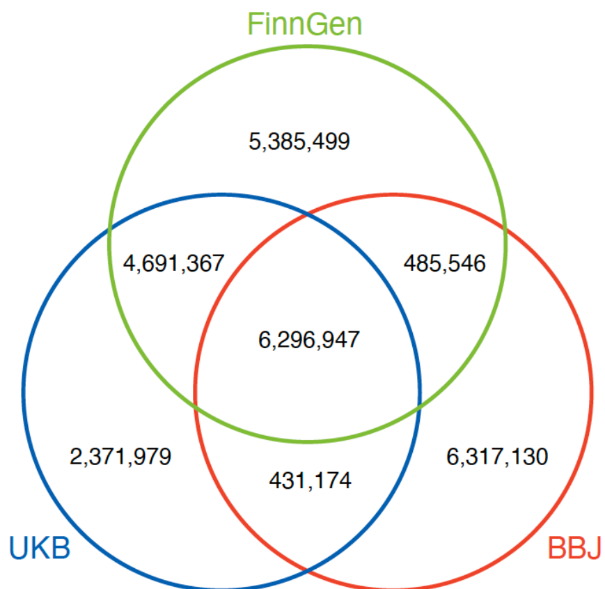
Extended Data Figure 17 | Genetic variants analyzed in the three cohorts.
