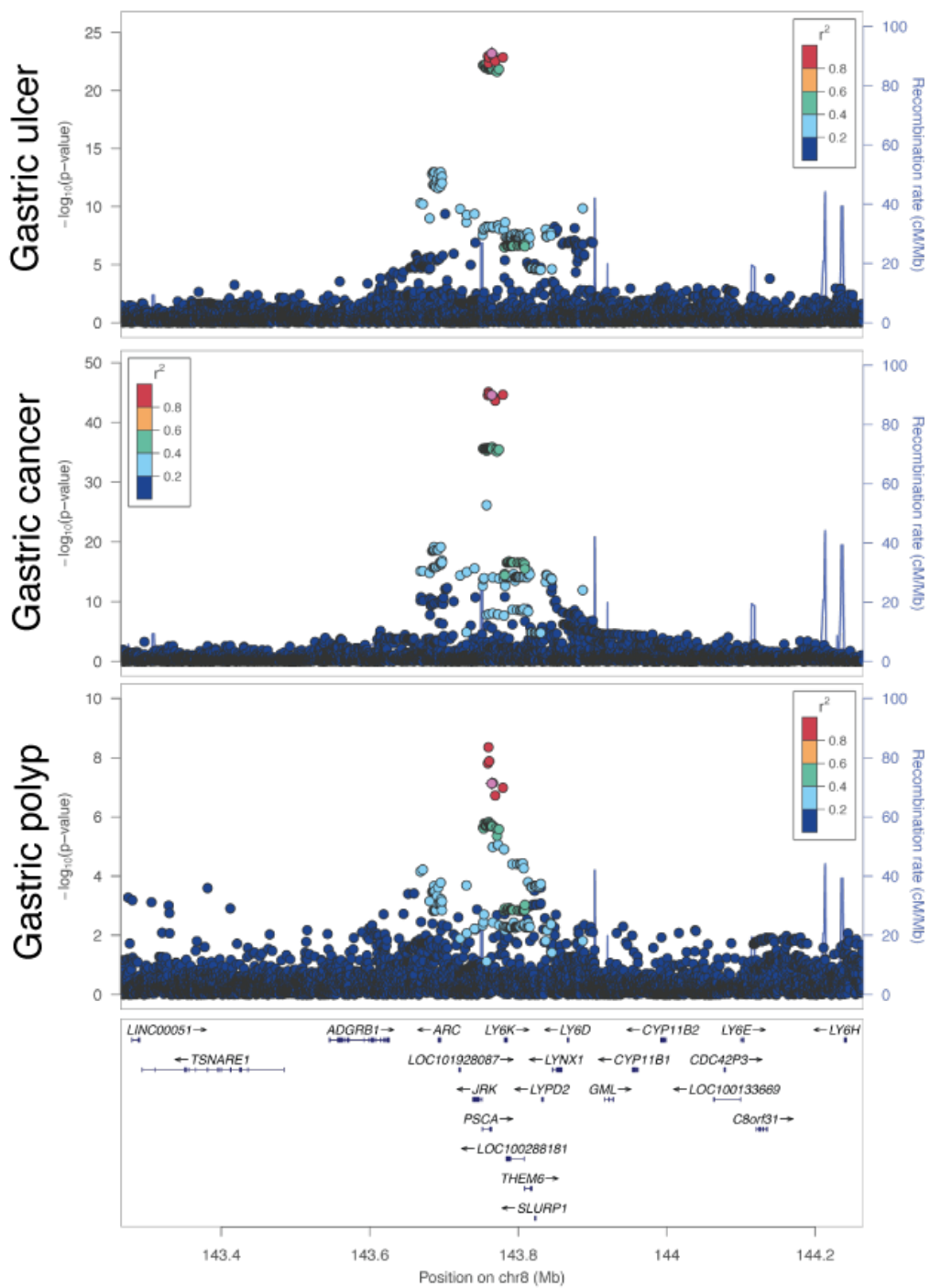
Extended Data Figure 4 | Locus plot for gastric diseases in BBJ.
