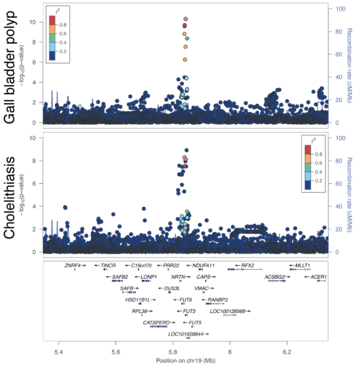
Extended Data Figure 5 | Locus plot for gall bladder diseases in BBJ.
