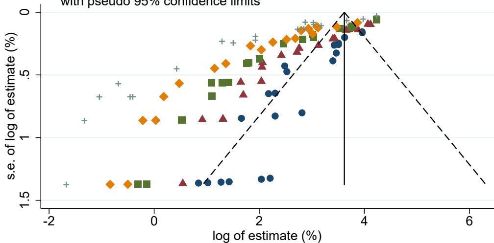
Funnel plot of Sars-CoV-2 attack rate by accommodation size with pseudo 95% confidence limits
