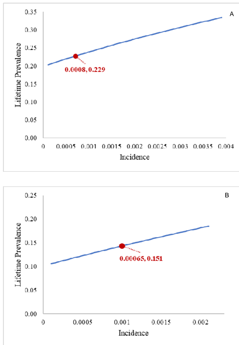
Figure 2. Feasible pairs of incidence and lifetime prevalence, with initial conditions, recurrence, remission, and mortality.
