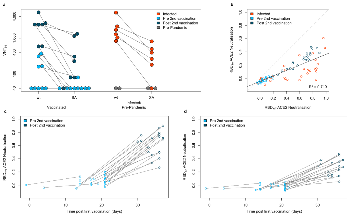
Figure 4 – South African RBD variant has decreased neutralization compared to wild-type in vaccinated and infected samples.
