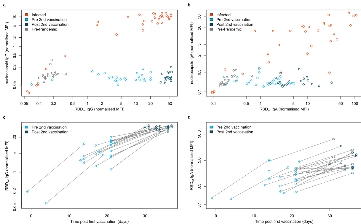
Figure 1 – IgG and IgA response in serum samples of vaccinated, infected and negative individuals.
