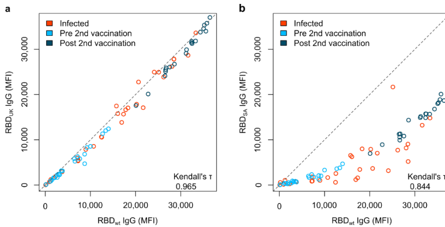
Figure 3 - South African RBD mutant has a reduced response compared to UK RBD mutant
