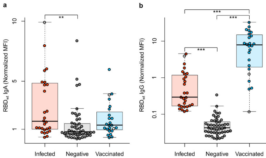
Figure 2 - IgA and IgG response in saliva samples of vaccinated, infected and negative individuals.
