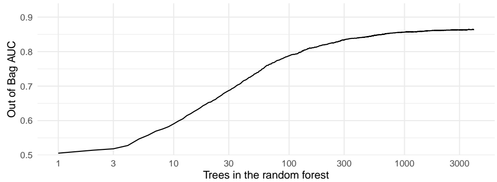
Figure A2. Random forest convergence plot shows ROC-AUC on out-of-bag data as forest size is increased exponentially.
