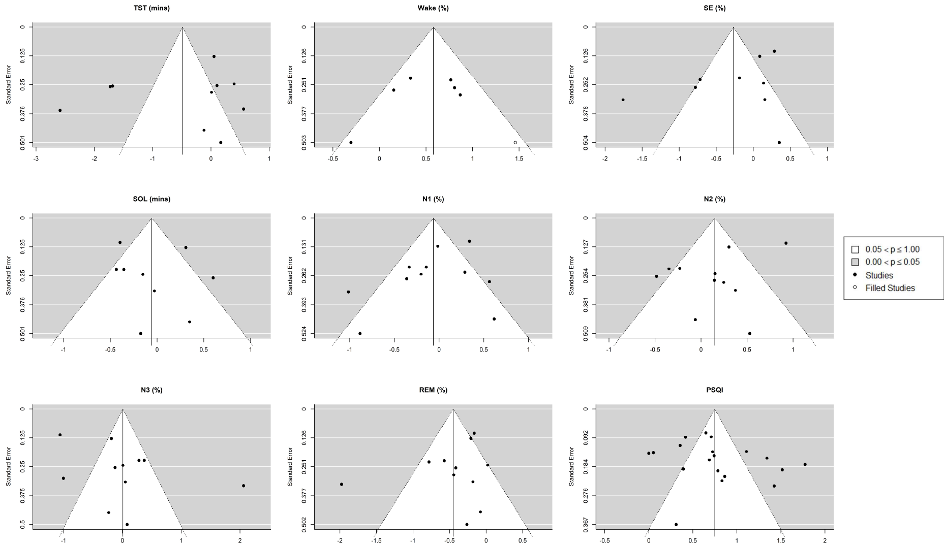
Figure e-1: Trim-and-fill funnel plots for each of the meta-analyses in migraineurs and controls
