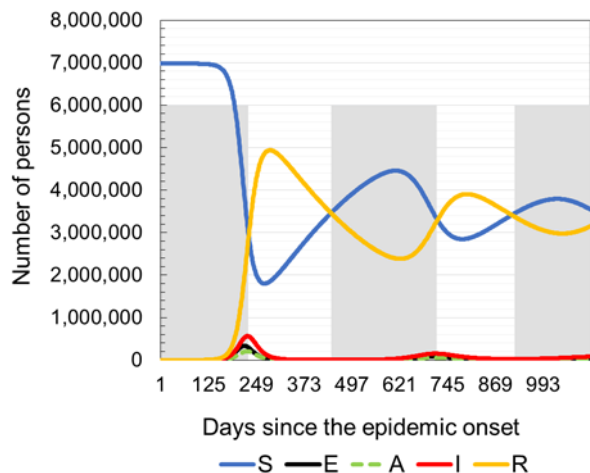
a) Prediction of the total number of the susceptible, latently infected, asymptomatic infectious individuals, infected and recovered on a daily basis since the epidemic onset. No intervention measures applied ( R_0=2.46 )
