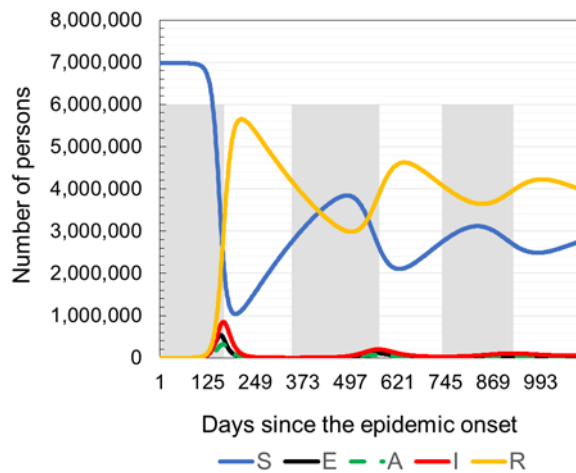
b) Prediction of the total number of the susceptible, latently infected, asymptomatic infectious individuals, infected and recovered on a daily basis since the epidemic onset. No intervention measures applied ( R_0=3.1 )
