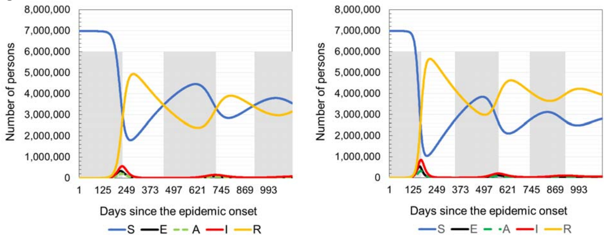
a) Distribution of the total number of the susceptible, latently infected, asymptomatic infectious individuals, infected and recovered on a daily basis since the epidemic onset ( R_0=2.46 )
