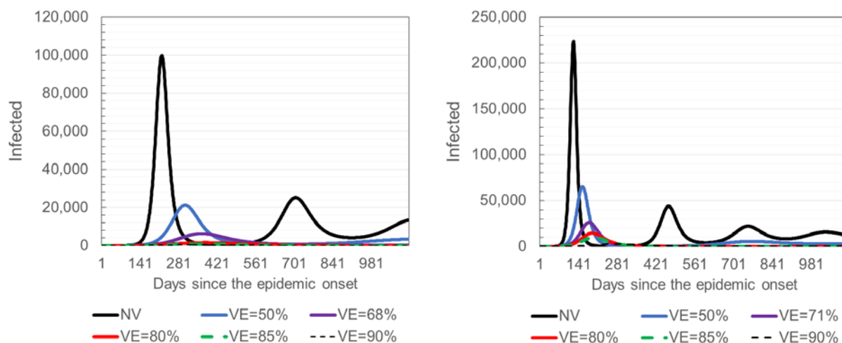
a) Comparative overview of daily incidences ( R_0=2.46 ).
