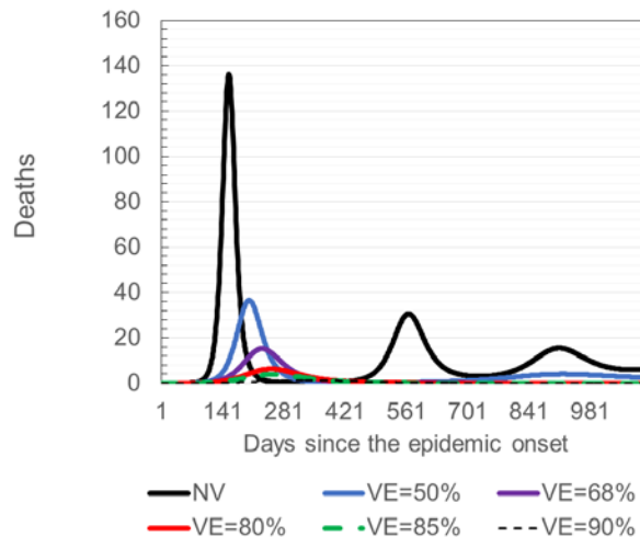
e) Comparative overview of deaths ( R_0=2.46 )
