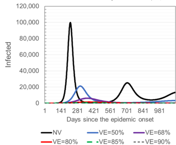
e) Results of simulated COVID19 control based solely on vaccination, scenarios 6-9 ( R_0=2.46 ).
