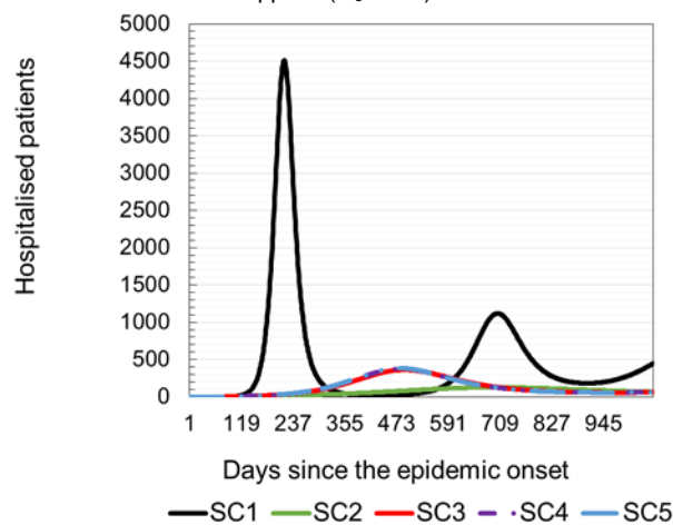
c) The results obtained during the simulation of the application of various contact reduction measures (scenarios 1-5, R_0=2.46 )
