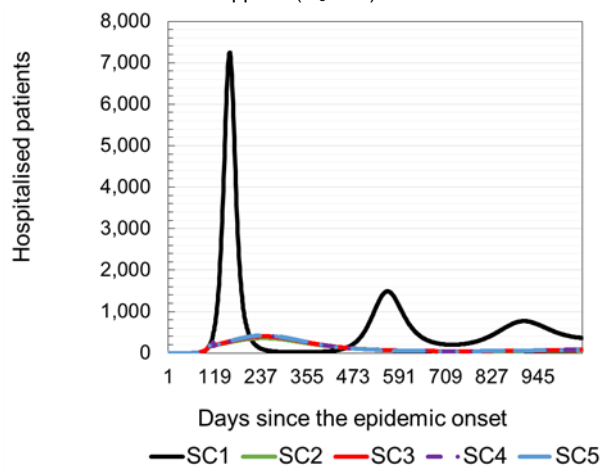
d) The results obtained during the simulation of the application of various contact reduction measures (scenarios 1-5, R_0=3.1 )
