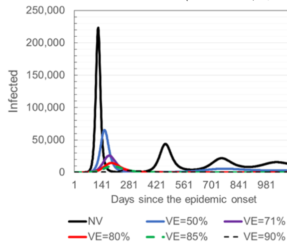
f) Results of simulated COVID19 control based solely on vaccination, scenarios 6-9 ( R_0=3.1 ).
