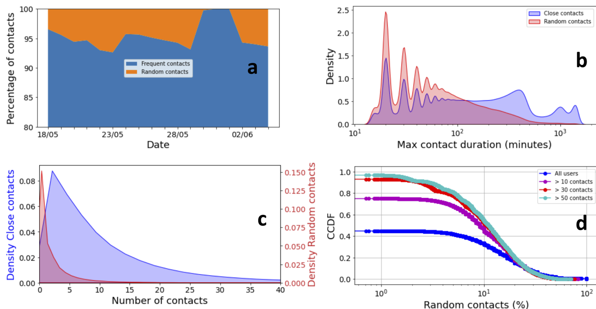
Figure 3: a) : The contacts split over time. The fraction of risky random contacts is stable over time and decreases in weekends and holidays, b) : The density of encounter duration. Frequent contacts tend to be markedly longer, c) : The density of the number of contacts per user, which are split based on the inferred contact type, d) : The complementary cumulative distribution of the percentage of random contacts per user for all users, users with 10 contacts or more (49% of all users), users with 30 contacts or more (12% of all users) and users with 50 contacts or more (4% of all users).
