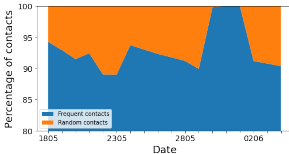
Figure S5: The timeseries of the fraction of random contacts for the RRC dataset.
