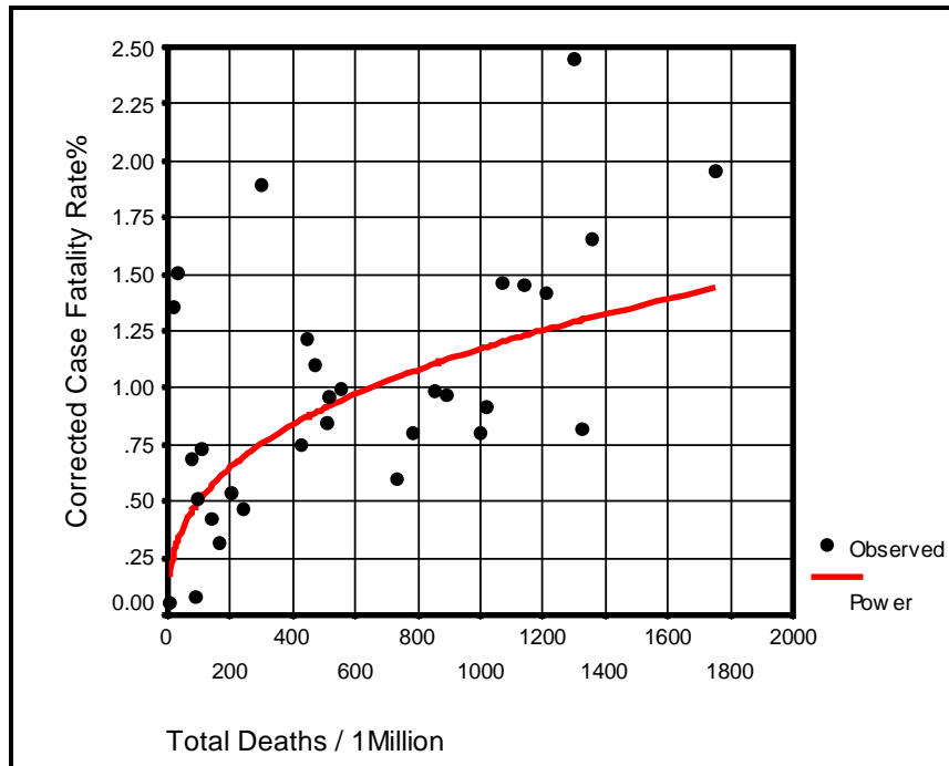
Figure No. (4): Shows the long term trend of scatter diagram effectiveness of Total Deaths No./1M. on Case Fatality Rate.
