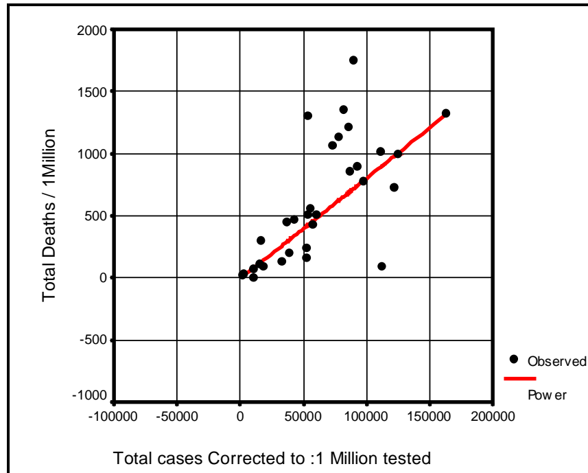
Figure (3): Long term trend of the scatter diagram concerning impact of total confirmed cases corrected to :1 M. tested on total deaths / 1Million
