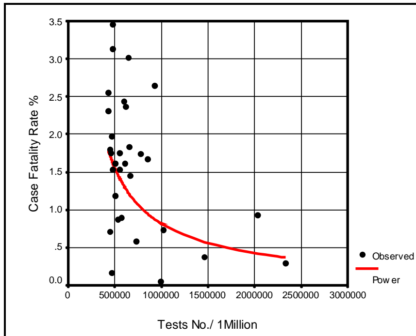
Figure No. (2): Shows the long term trend of scatter diagram effectiveness of tested no./1M. tested on corrected CFR.
