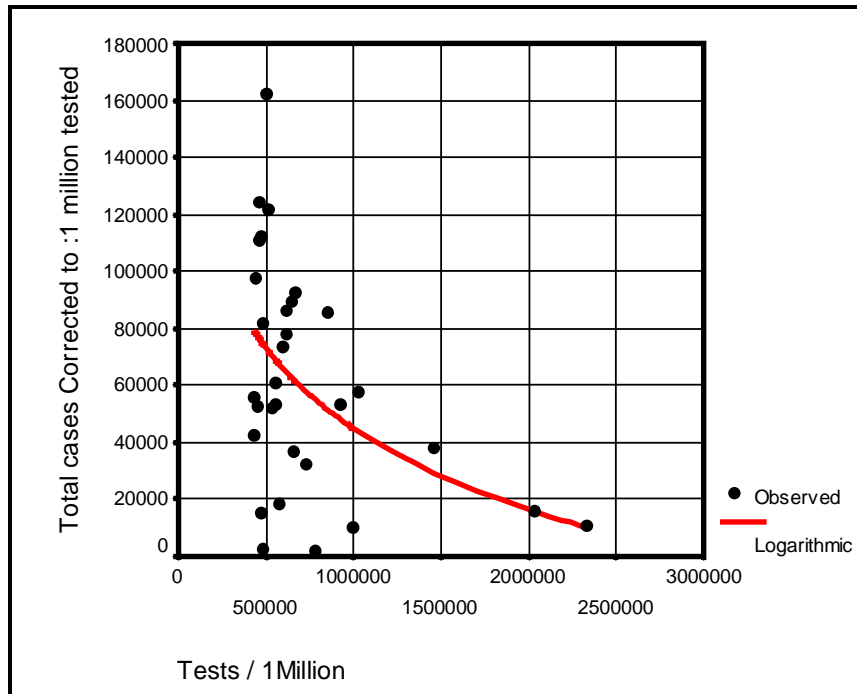
Figure (1): Long term trend of the scatter diagram concerning impact of test no. / 1M. on total cases corrected to 1M. tested
