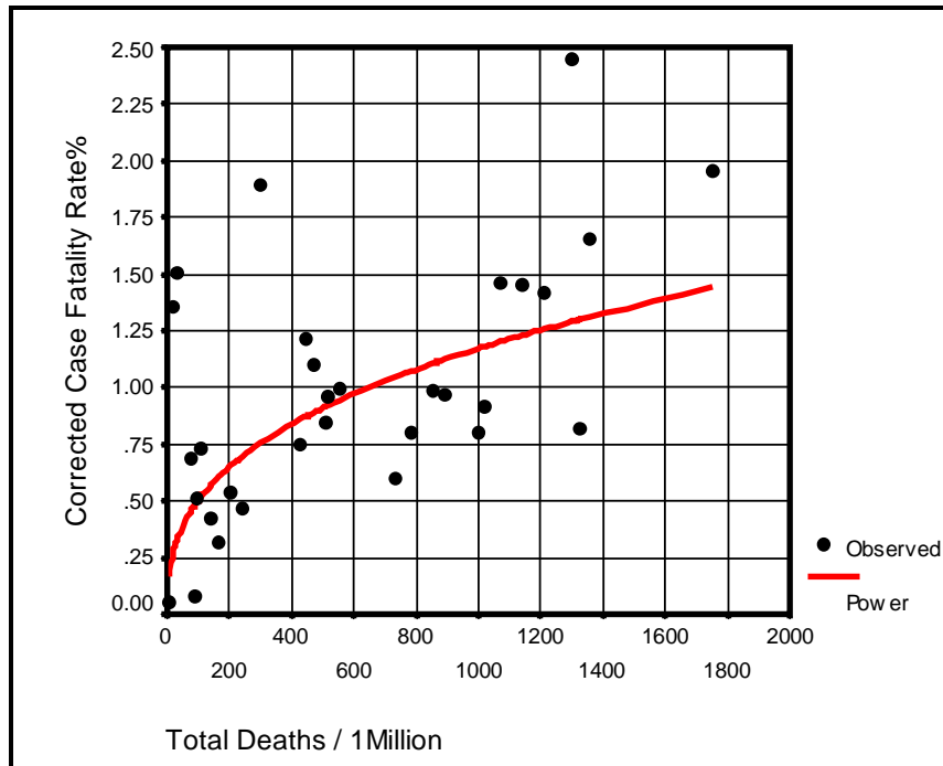
Figure (4): Long term trend of the scatter diagram concerning total deaths No./1M. population on CFR
