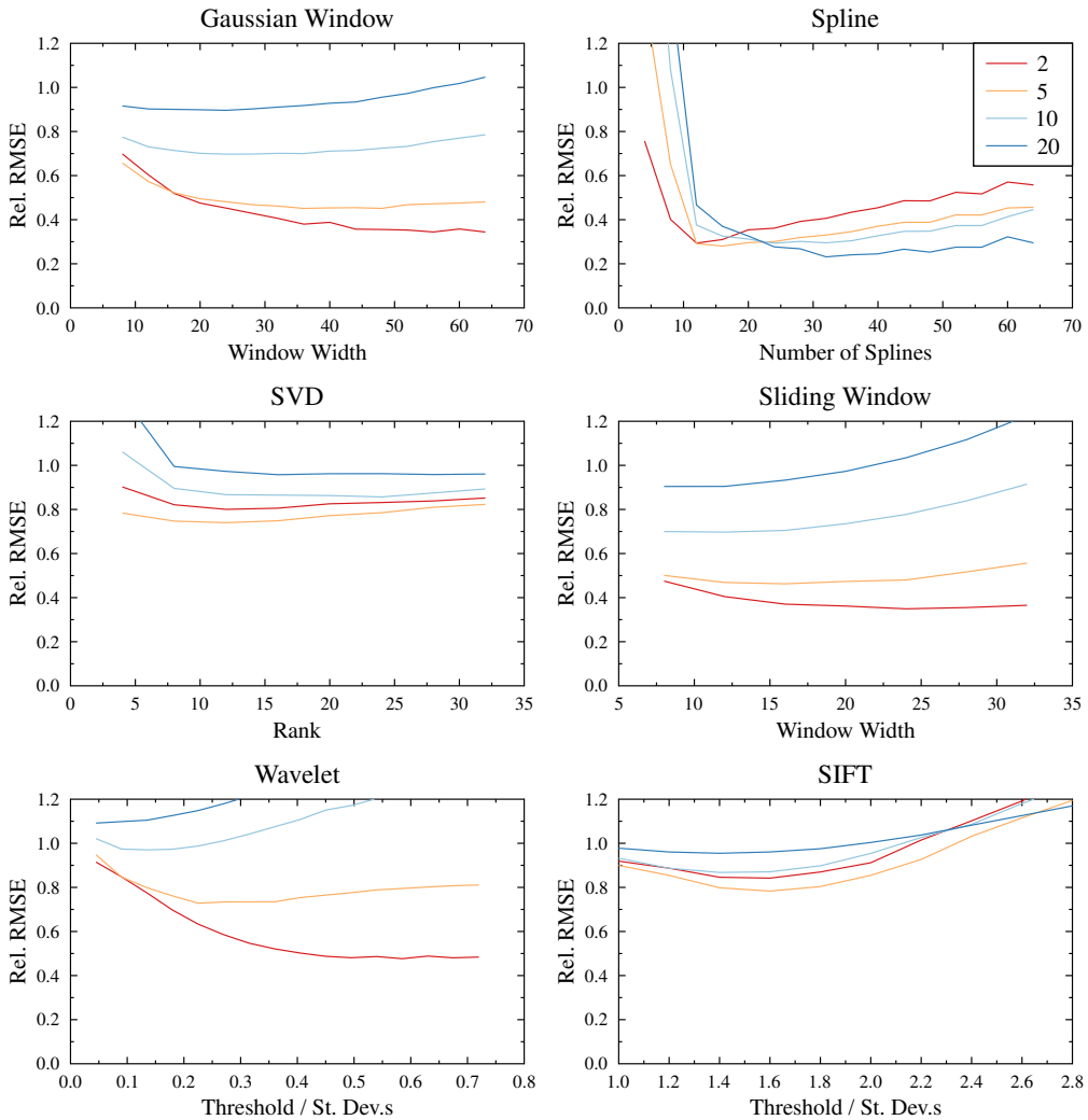
FIGURE 2 Effect of indirect time domain denoising on quantification of dynamic spectra. Each panel shows the average RMSE between the ground truth and the quantified metabolite timecourse of the denoised pseudo-synthetic data, relative to un-denoised data, as the denoising tuning parameter is varied, for four different levels of SNR.
