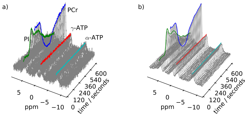
FIGURE 3 Pseudo-synthetic dataset with SNR 5 before (a) and after (b) applying spline denoising in the indirect time domain. Also shown are the quantified metabolite concentrations for the metabolites of interest. PCr=Phosphocreatine; PI=Inorganic phosphate; ATP=Adenosinetriphosphate.
