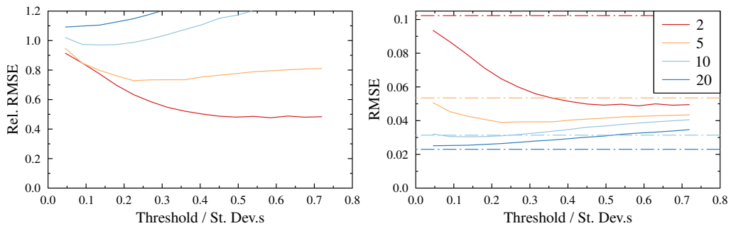
FIGURE 5 Performance of the wavelet denoising technique shown both relative to raw (un-denoised) data (left) and in absolute performance (right). From the absolute RMSE representation it is clear that as the threshold increases, the wavelet denoising converges to the same representation of the signal irrespective of the SNR. While this is closer to correct than the low SNR raw data, we can see that the spectra are distorted relative to the high SNR raw data.
