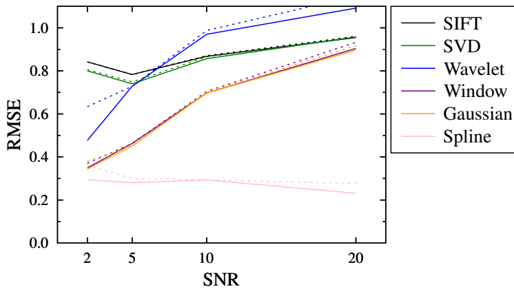
FIGURE 4 Relative performance of the different denoising methods with optimal tuning parameters. The solid lines show performance with per-SNR tuning parameters, while the dashed line shows performance with a common, globally optimal tuning parameter.
