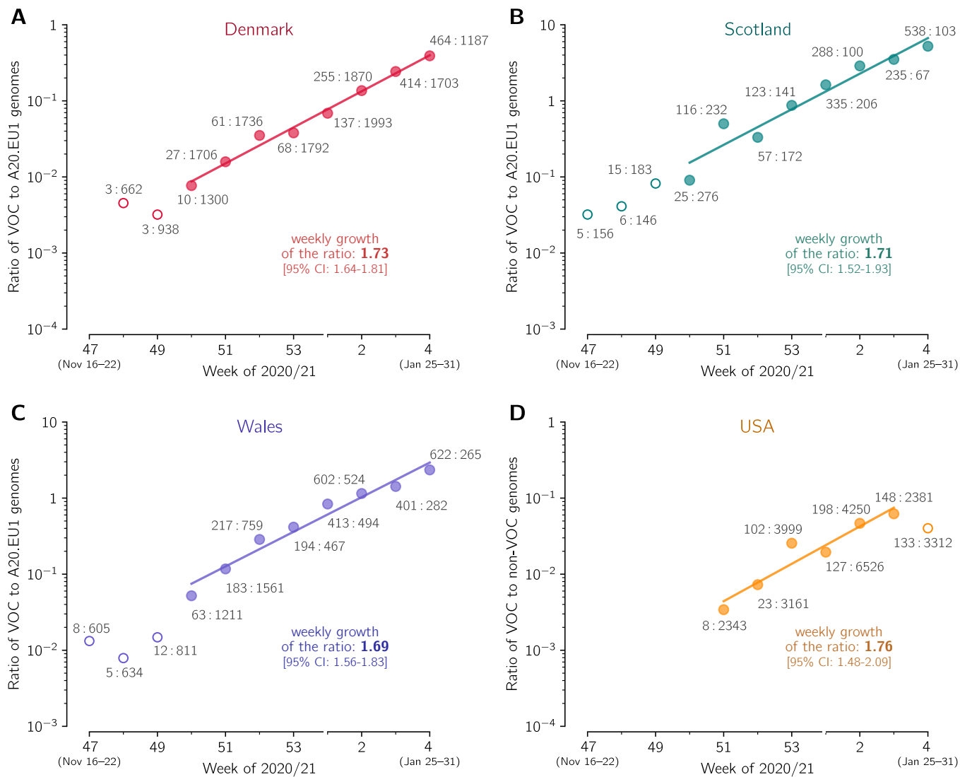
Figure 3: The replicative advantage of the VOC in Denmark, Scotland, Wales, and USA. (A) The ratio of the VOC to the 20A.EU1 sequences collected in Denmark. The trend line is fitted to data points from week 50 of 2020 to week 4 of 2021. (B) The ratio of the VOC to 20A.EU1 sequences collected in Scotland. The trend line is fitted to data points from weeks 50 of 2020 to week 4 of 2021. (C) The ratio of the VOC to 20A.EU1 sequences collected in Wales. The trend line is fitted to data points from week 50 of 2020 to week 4 of 2021. (D) The ratio of the VOC to non-VOC sequences collected in USA. The trend line is fitted to data points from week 51 of 2020 to week 3 of 2021. Data points are labeled with ratios of the counts of genome sequences. The weekly growth rates and respective confidence intervals are given in each panel. All panels are based on GISAID data submitted till February 17, 2021 (provided in supplementary Data File S1).
