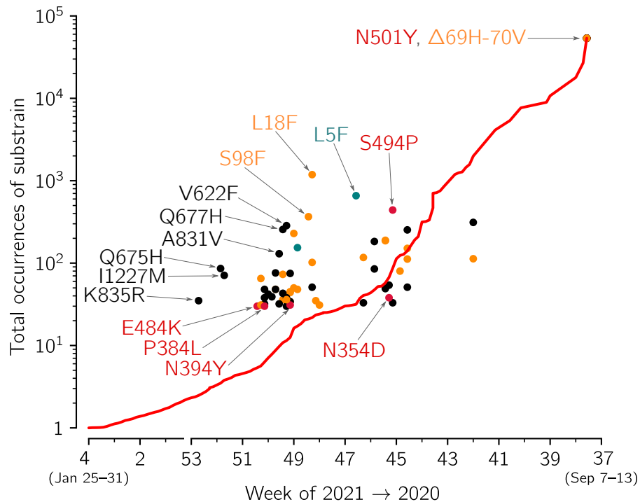
Figure 6: The growth of VOC substrains with respect the whole VOC strain. The figure is based on spike protein sequences from genomes collected in England and submitted to GISAID till February 12, 2021. The growth of the whole VOC strain (red line) in the time span between t and t_0 = February 12, 2021 is calculated as VOC(t_0)/VOC(t) , i.e., the ratio of the number of the VOC genomes collected till February 12, 2021 and the number of VOC genomes collected till t (date given on horizontal axis). Disks denote VOC substrains defined by particular mutations (with at least 30 genomes submitted); horizontal axis value for each circle is the date of first collection of a sequence with a given mutation; vertical axis value is the number of genomes collected till February 12, 2021, conferring a given mutation. Red, orange, and green circles denote substrains with leading mutation in respectively in RBD, NTD, and signal peptide; black circles denote mutations in other domains. Selected substrains that may have replicative advantage and all substrains with the leading mutation in RBD are annotated. Detailed data that were analyzed to prepare this figure are provided in supplementary Data File S1 (sheet 'Mutations').
