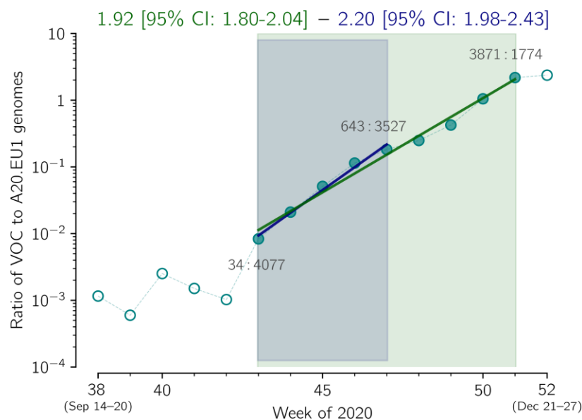
Figure S1. The replicative advantage of VOC over 20A.EU1 in England, based on COG. Ratio of VOC to 20A.EU1 genomes collected from pillar 2 tests in weeks 38-51 in England. The trend line is fitted to data points from weeks 43-51 (green) and from weeks 43-47 (blue). The weekly growth rate is 1.92 [95% CI: 1.80-2.04] for weeks 43-51 and 2.20 [95% CI: 1.98-2.43] for weeks 43-47. The estimated R ratio is R_t^{\text{VOC}} / R_t^{20\text{A.EU1}} = 1.87 [95% CI: 1.76-1.98] for weeks 43-51 and 2.13 [95% CI: 1.93-2.35] for weeks 43-47.
