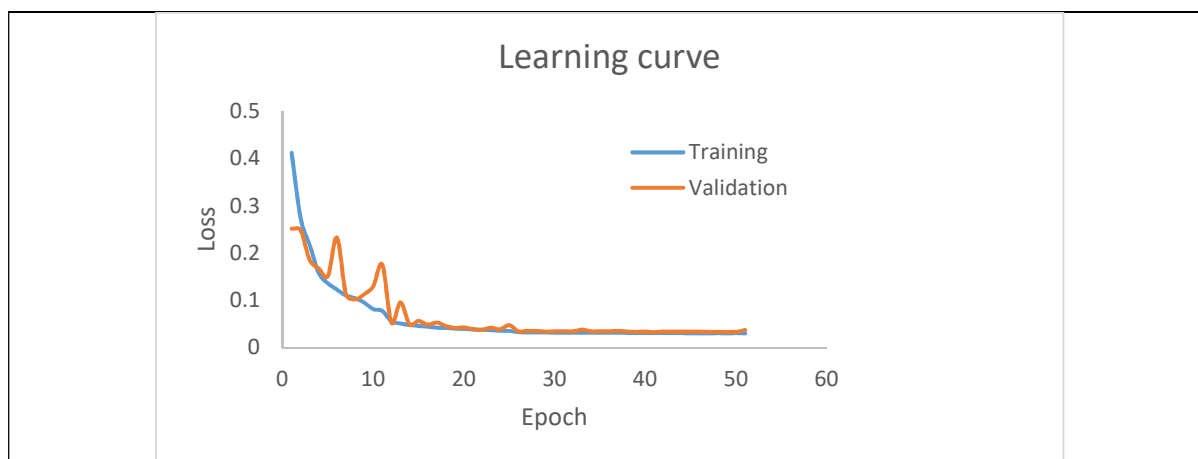
Figure 5: Learning curves: trained with (A) aorta and coronary arteries (B) coronary arteries only
