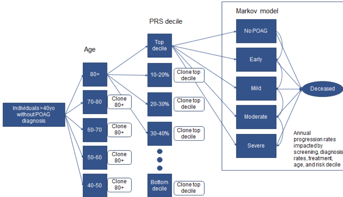
447 Figure 1: A schematic of Markov Model structure used for the genetic screening of 448 primary open-angle glaucoma ‘pathway’
