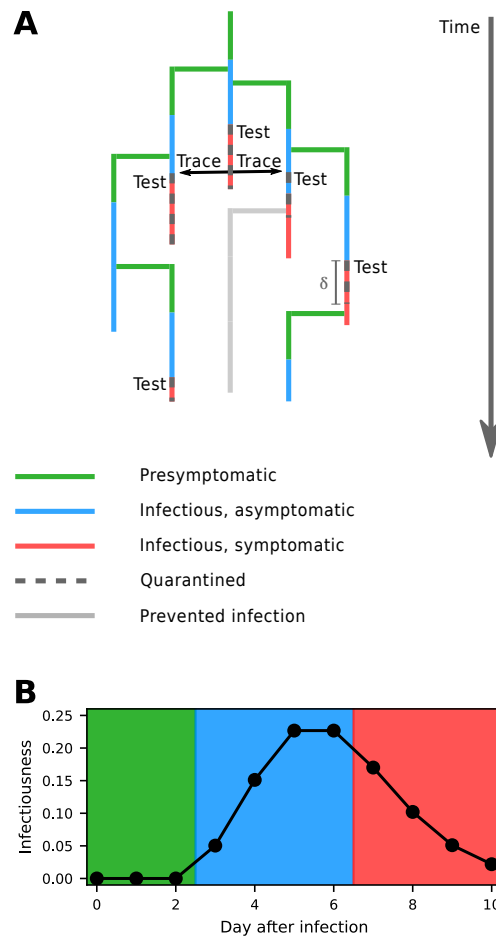
FIG. 1. A Illustration of our model. Infectious people transmit the disease unless they are placed in quarantine following testing and tracing efforts. The success of these efforts are contingent on the three key parameters of the model: the test waiting time \delta , test sensitivity 1 - p_{\text{false}} , and tracing efficiency p_{\text{trace}} . B Infectiousness over time, P_{\text{time}}(t) , in our model. Background colors specify whether the infected experiences symptoms and is infectious at the given time (see legend in Figure 1A) The value on the vertical axis for day x after infection is the probability that a given secondary case gets infected on day x . For asymptomatic cases, P_{\text{time}}(t) is as depicted – the only difference being that the final, symptomatic, phase is replaced with an asymptomatic phase.
