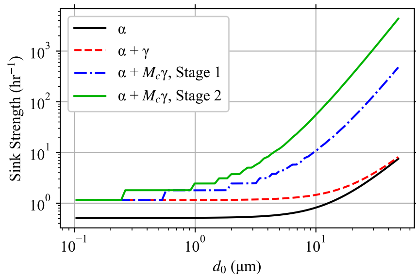
Fig 4. Sink Strength by Bin. The strength of the sink terms for each bin with 80 bins, which is \alpha without inactivation, \alpha + \gamma for k = 1 , and \alpha + M_c \gamma for k = M_c (different values for Stage 1 and 2).
