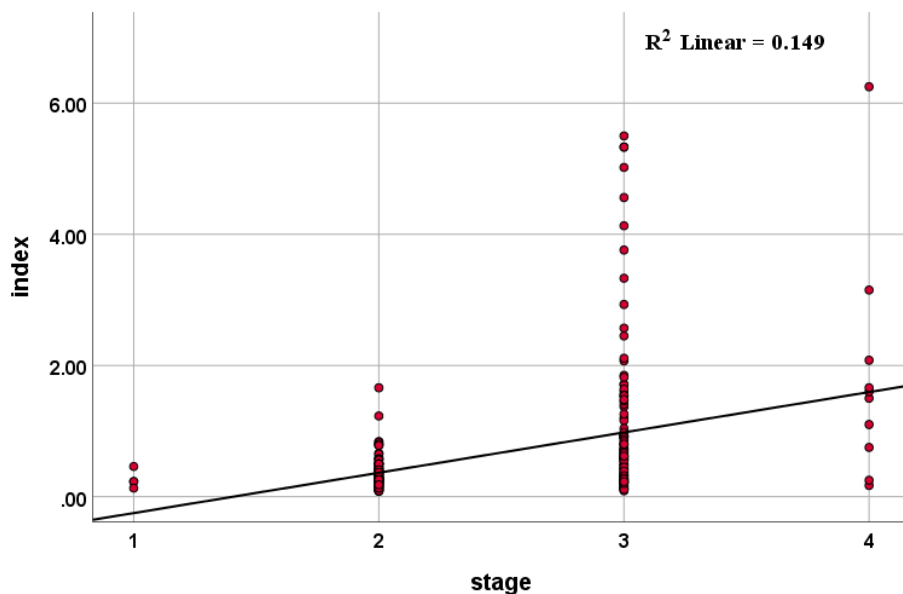
Figure 1: Dot plot represent the regression model between the index and the stage of Covid -19 disease.
