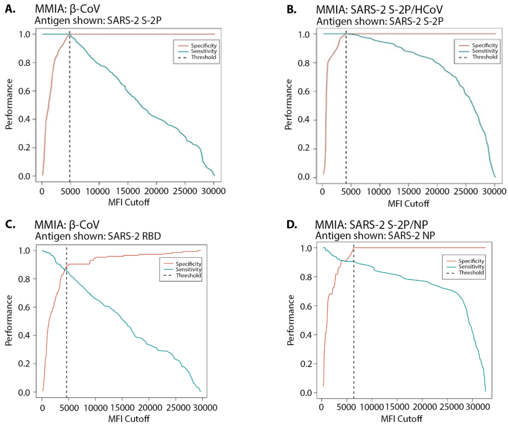
Figure S2. Receiver operating characteristic (ROC) curve analysis of SARS-CoV-2 PCR-positive and -negative serum samples from the EPICC study provided a second measurement of threshold cutoffs for SARS-CoV-2 antigen reactive IgG. EPICC Sera were tested with MMIA indicated in panels; antigens shown as follows: (A) SARS-CoV-2 spike (S-2P), (B) SARS-CoV-2 spike (S-2P), (C) SARS-CoV-2 RBD, and (D) SARS-CoV-2 N
