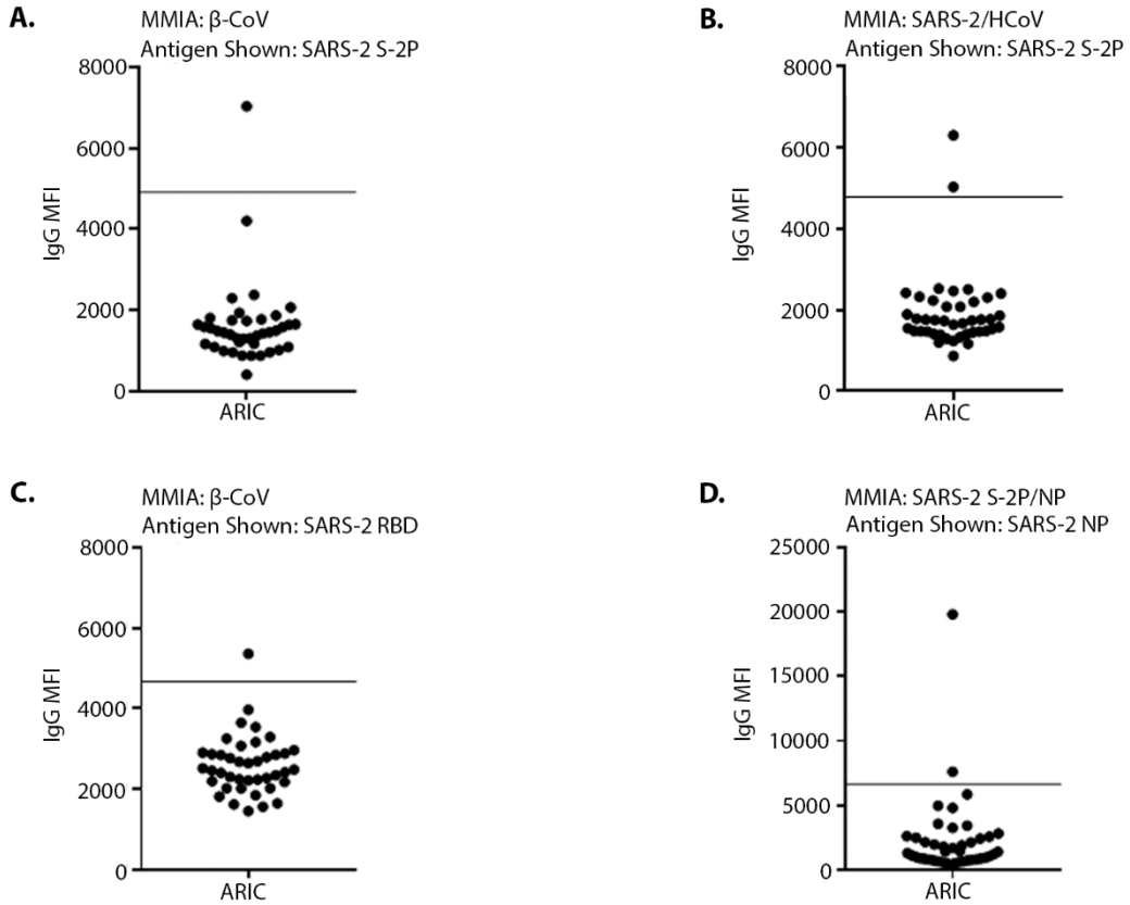
Figure S1. 99.7% probability distribution threshold cutoffs for SARS-CoV-2 antigen
