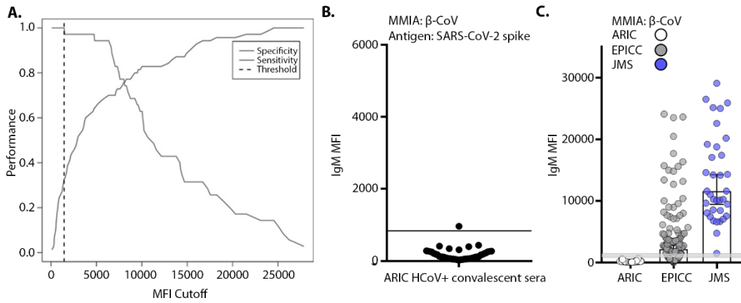
Figure S3. SARS-CoV-2 spike reactive IgM detection with the \beta -CoV MMIA.
