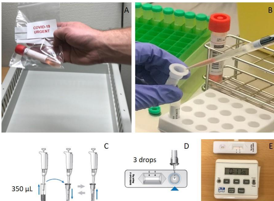
Figure 2. Antigen testing procedure with reference test (Roche).
