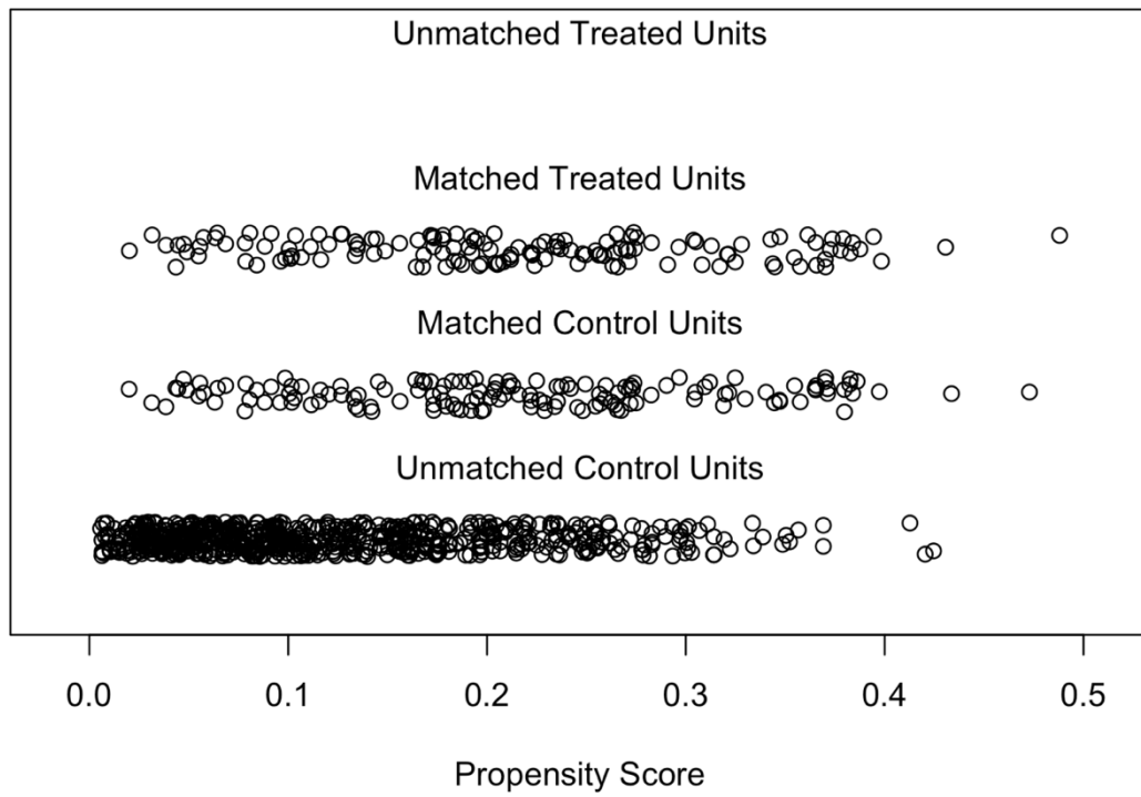
Supplemental Figure S3: Distribution of Propensity Scores
