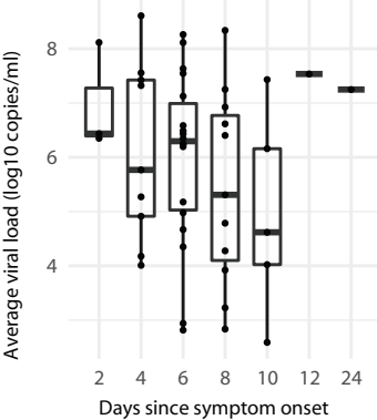
Figure S3. SARS-CoV-2 viral load at different days post symptom onset. Index cases (N=49) were asked when their symptoms started, and viral load was measured at study start. Individuals are binned together based on their reported symptom onset, relative to the study start. The y-axis shows the average viral load in log10 copies/ml extracted sample.
