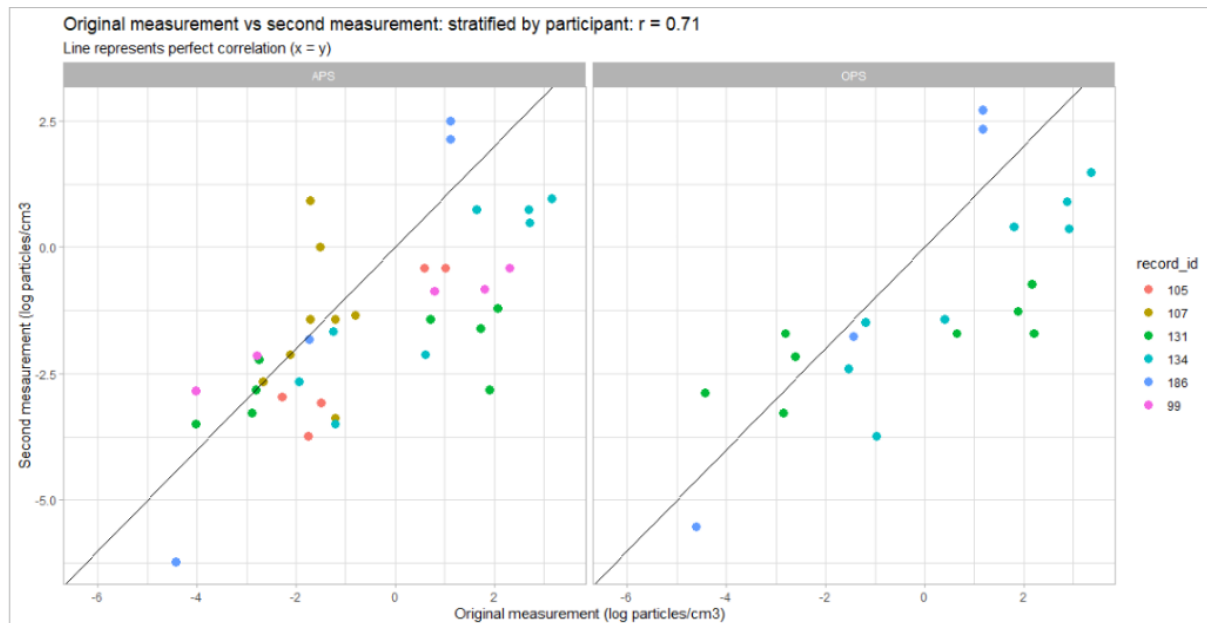
Figure S1: The aerosol number concentration sampled by an APS during baseline measurements for six subjects compared to that for a repeat measurement at a later date. For breathing and speaking activities, the mean concentration per sample (equivalent to 1 s acquisition) is reported; for coughing the peak concentration sampled during any sample (1 s acquisition) is reported. Data are classified by colour according to the subject (displayed in legend).
