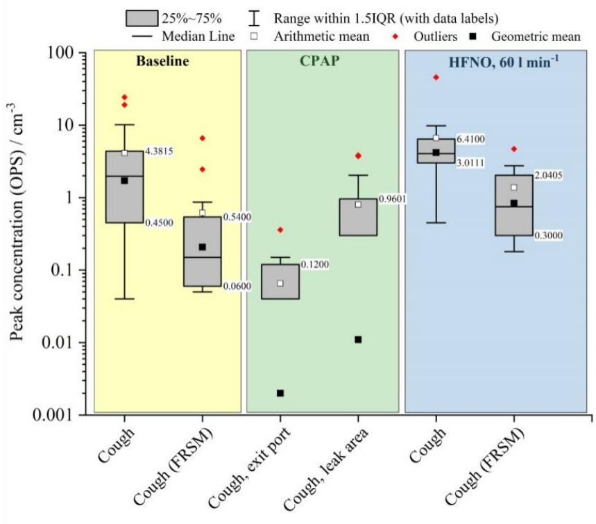
Figure S3: The aerosol number concentration sampled by an OPS during baseline activities, CPAP or HFNO, with a) reporting the mean concentration sampled during breathing and speaking and b) reporting the peak concentration sampled during coughs.
