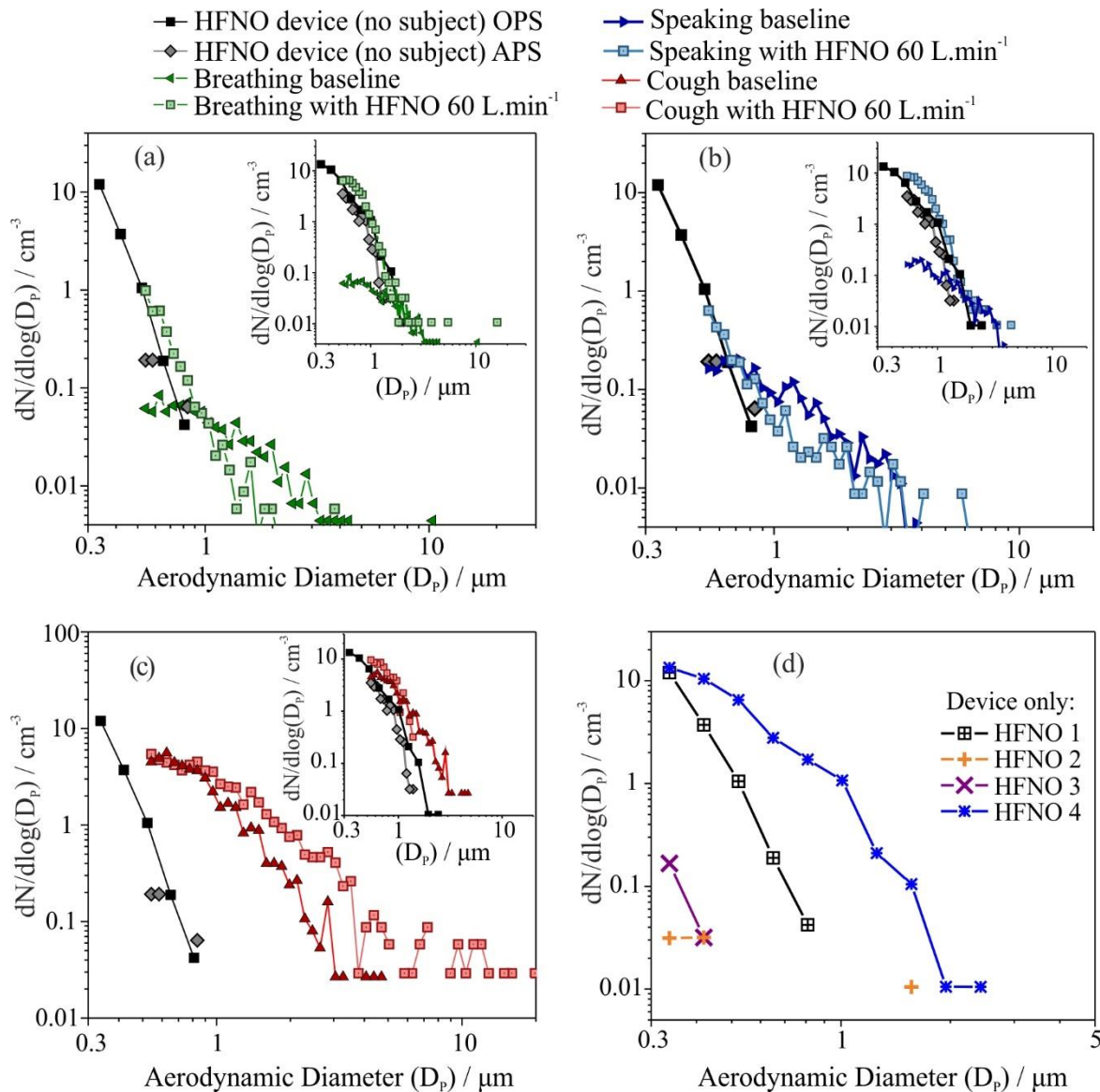
Figure S8: The mean size distribution of healthy subjects performing a baseline respiratory activity ( n=25 ) and also during 60 \text{ L}\cdot\text{min}^{-1} HFNO ( n=23 ), compared to the size distribution of particles generated by the HFNO device and cannula. Inset shows the mean distribution of healthy subjects performing the same baseline activity ( n=6 ), but with an alternative HFNO device that generates more particles in a different size distribution. Respiratory activities are breathing, speaking and coughing for a), b) and c), respectively. d) OPS size distributions of particles originating just from the HFNO device for four different devices, where “HFNO 1” is that used for the majority of HFNO datasets ( n=23 ) and “HFNO 4” is that used for the additional six subjects in the figure insets. HFNO devices 2 and 3 generate fewer particles but were not used for subject datasets.
