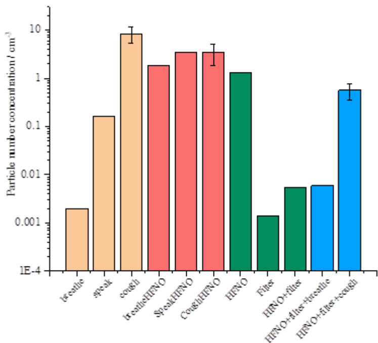
Figure S5: APS total particle count detected from 1 second of activity / \text{cm}^{-3} for breathing and speaking and peak height cough data / \text{cm}^{-3} from one subject assessing particle source during HFNO delivery. Baseline measurements (cream) show breathing and speaking and coughing data without HFNO. Baseline measurements whilst receiving HFNO delivery (coral) for subject are greater. Addition of the 0-particle HEPA filter without the subject present measurements are shown in green. The subject was then introduced with the filter in series (blue). The sustained, timed activities (breathing, speaking, HFNO device alone) have the mean concentration per sample reported (equivalent to 1 s acquisition)
