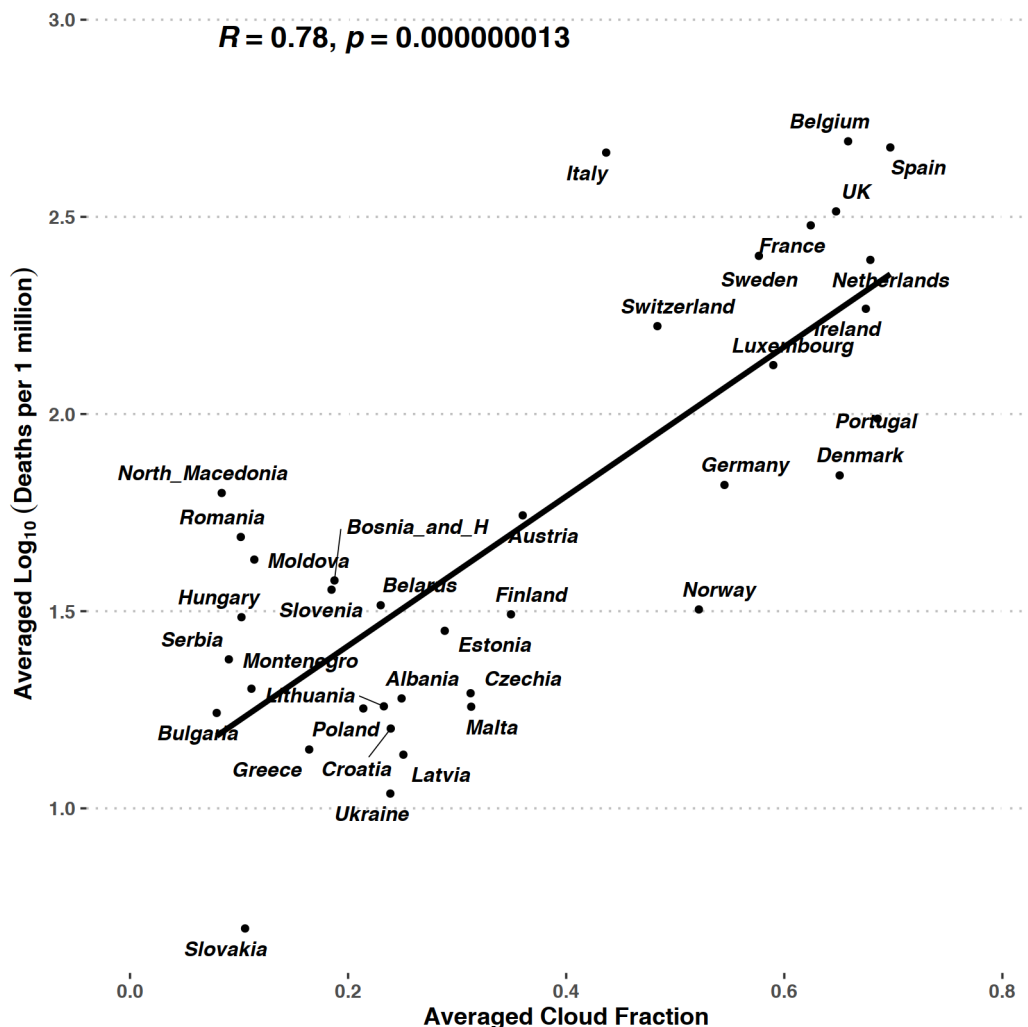
Figure 1. Overall correlation between mortality and cloudiness.
