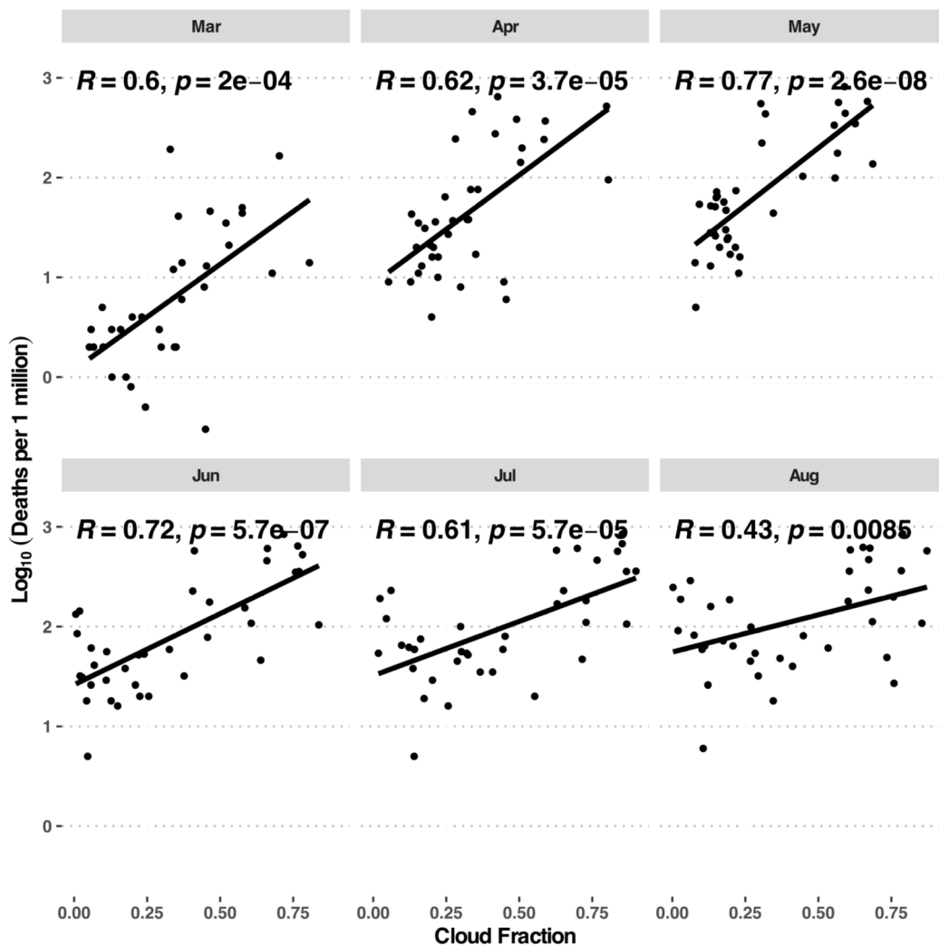
Figure 3. Monthly correlation between mortality and cloudiness. The data points are the values for all European countries included in the study for each month of the interval studied (March – August 2020). Cloudiness is expressed as the cloud fraction, which ranges between 0.0 (completely sunny sky) and 1.0 (clouds completely obscure the sun).
