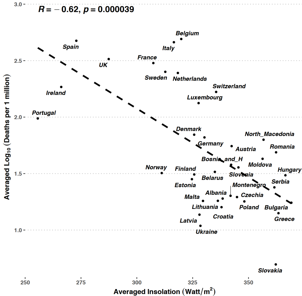
Figure 2. Overall correlation between averaged mortality and averaged insolation (solar irradiance). The data points are the averaged values for all European countries included in the study during March – July 2020. The dashed line represents the apparently good-fitting linear model, although this model is not valid upon close inspection (see text). We included it as a guide for the eye.
