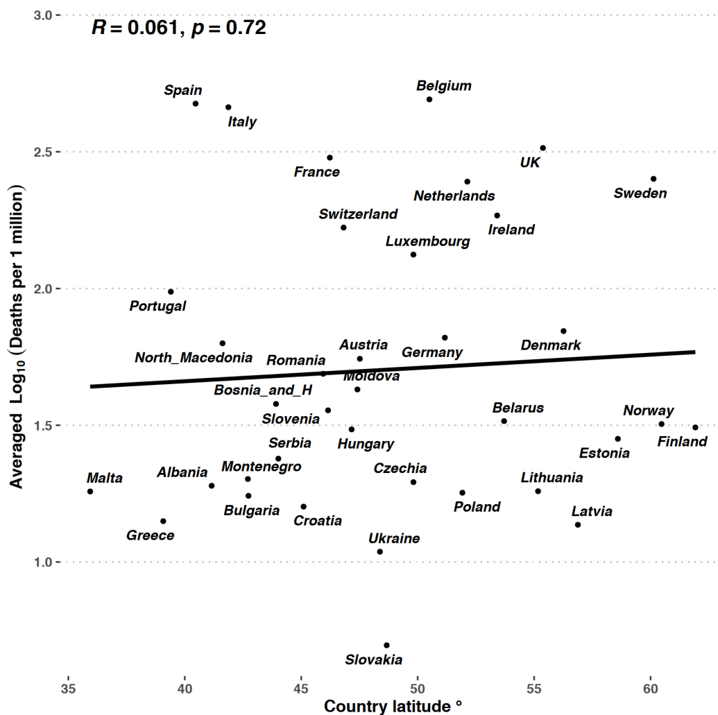
Figure 4. COVID-19 mortality and latitude of the European countries. No correlation found; the data points are the averaged mortality values for all European countries included in the study during March – August 2020.
