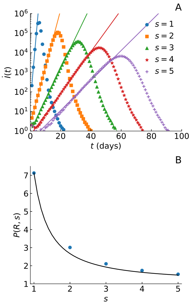
FIG. 4. Numerical simulations of disease transmission in a virtual city. A) Average number of new infectious as a function of time for different number of intermediate states (symbols). The lines are fits to the exponential function in Eq. (27), providing an estimate of P . B) Population reproductive number P as a function of s , as obtained from the fitting to the numerical data (symbols) and from the expected theoretical line (28) (line).
