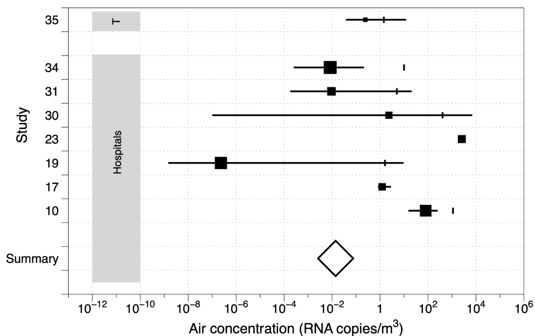
Figure 4: Imputed geometric mean SARS-CoV-2 RNA air concentrations
