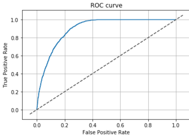
Fig. B.3. ROC Curve of the Binary Gradient Boosting Decision Tree Model.
