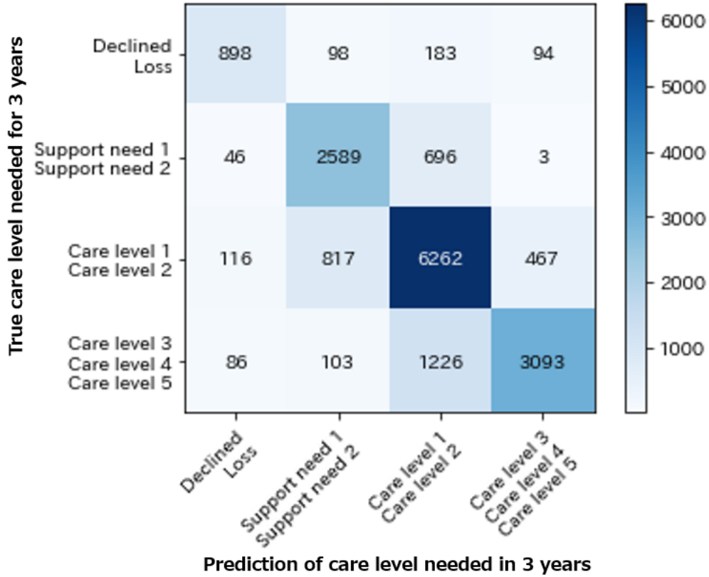
Fig. B.1. Confusion Matrix of the Four-Category Predictive Model.
