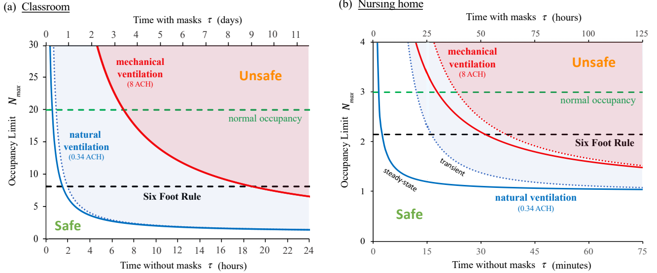
Fig. 3. The COVID-19 indoor safety guideline would limit the cumulative exposure time in a room with an infected individual to lie beneath the curves shown. Solid curves are deduced from the pseudo-steady formula, Eq. [5], for both natural ventilation ( \lambda_a = 0.34/h ; blue curve) and mechanical ventilation ( \lambda_a = 8.0/h ; red curve). Horizontal axes denote occupancy times with and without masks. Evidently, the Six-Foot Rule (which limits occupancy to N_{max} = \sqrt{A}/(6ft) ) becomes inadequate after a critical time, and the 15-Minute Rule above a critical occupancy. (a) A typical school classroom: 20 persons share a room with an area of 900 square feet and a ceiling height of 12 feet ( A = 83.6 \text{ m}^2 , V = 301 \text{ m}^3 ). We assume low relative transmissibility ( s_r = 25\% ), cloth masks ( p_m = 30\% ) and moderate risk tolerance ( \epsilon = 10\% ) suitable for children. (b) A nursing home shared room ( A = 22.3 \text{ m}^2 , V = 53.5 \text{ m}^3 ) with a maximum occupancy of three elderly persons ( s_r = 100\% ), disposable surgical or hybrid-fabric masks ( p_m = 10\% ) and a low risk tolerance ( \epsilon = 1\% ) to reflect the vulnerability of the community. The transient formula, Eq. [S8], is shown with dotted curves. Other parameters are C_q = 30 \text{ quanta/m}^3 , \lambda_v = 0.3/h , Q_b = 0.5 \text{ m}^3/h , \bar{\tau} = 0.5 \mu\text{m} .
