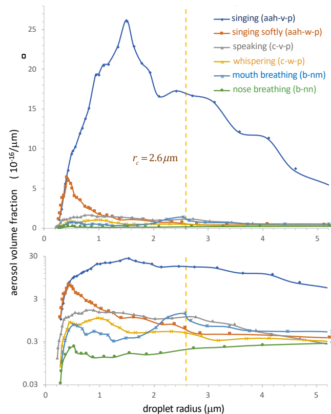
Fig. 1. Model predictions for the steady-state, droplet-radius-resolved aerosol volume fraction, \phi_s(r) , produced by a single infectious person in a well-mixed room. The model accounts for the effects of ventilation, pathogen deactivation and droplet settling for several different types of respiration in the absence of face masks ( p_m = 1 ). The ambient conditions are taken to be those of the Skagit Valley Chorale super-spreading incident (24, 26) ( H = 4.5\text{m} , A = 180\text{m}^2 , \lambda_a = 0.65\text{h}^{-1} , r_c = 2.6\mu\text{m} , \lambda_v = 0.3\text{h}^{-1} , RH = 50\% ). The expiratory droplet size distributions are computed from the data of Morawska et al. at RH = 59.4\% (9) (see their Fig. 3) for aerosol concentration per log-diameter, using n_d(r) = (dC/d \log D)/(r \ln 10) . The breathing flow rate is assumed to be 0.5\text{m}^3/\text{h} for nose and mouth breathing, 0.75\text{m}^3/\text{h} for whispering and speaking, and 1.0\text{m}^3/\text{h} for singing.
