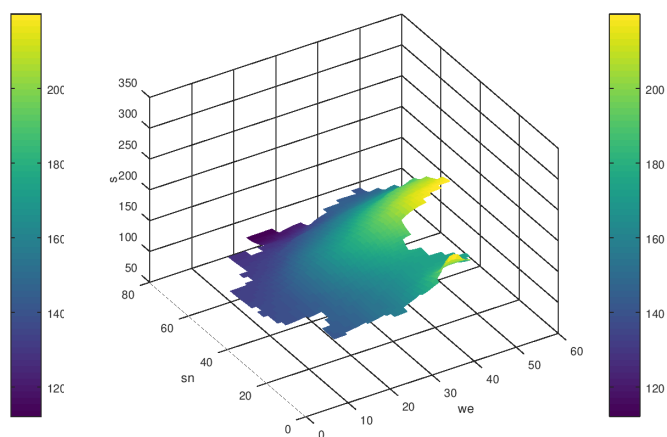
Figure 12: s after 200 time-steps, \gamma = 50\text{km/day} , q = 0
