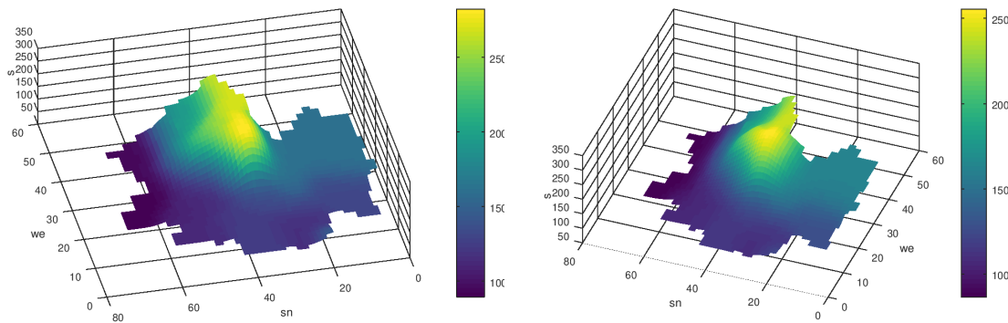
Figure 13: s after 10 time-steps, q \neq 0 , based on table 2 Figure 14: s after 20 time-steps, q \neq 0 , based on table 2
