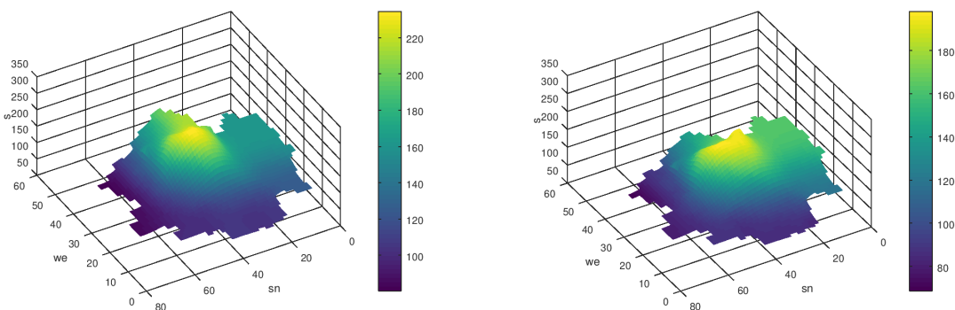
Figure 15: s after 30 time-steps, q \neq 0 , based on table 2 Figure 16: s after 50 time-steps, q \neq 0 , based on table 2
